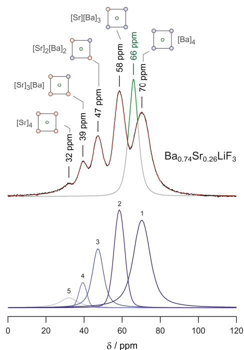
Fig. 7: ^{19}\text{F} MAS NMR spectrum of \text{Ba}_{0.74}\text{Sr}_{0.26}\text{LiF}_3 revealing the individual NMR signals of the different environments of the F ions. Since in \text{BaLiF}_3 the F sites are magnetically equivalent only a single signal shows. Depending on the number of Sr atoms in the direct vicinity of the ^{19}\text{F} nucleus the chemical shift ranges from 70 to 32 ppm. Figure taken from ref. 52.
