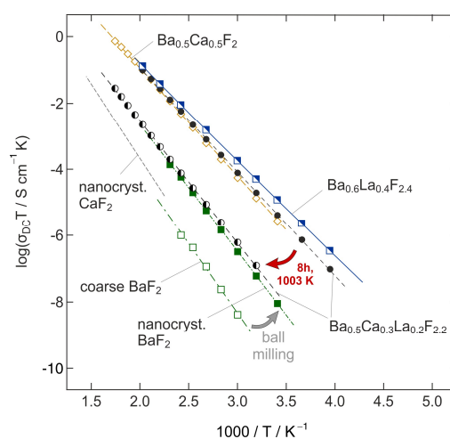
Fig. 9: Overview of the ionic conductivities of several \text{BaF}_2 -derived compounds. Ball milling of coarse-grained \text{BaF}_2 yields a nanocrystalline sample which shows a conductivity that is almost two orders of magnitudes higher compared to the non-milled material. Ion conductivity can be further improved by mixing \text{BaF}_2 and \text{CaF}_2 yielding a non-equilibrium phase taking advantage of local disorder and strain introduced when missing cations of different sizes. The highest values are found for \text{Ba}_{0.6}\text{La}_{0.4}\text{F}_{2.4} , which was studied by NMR relaxometry in detail, see below.
