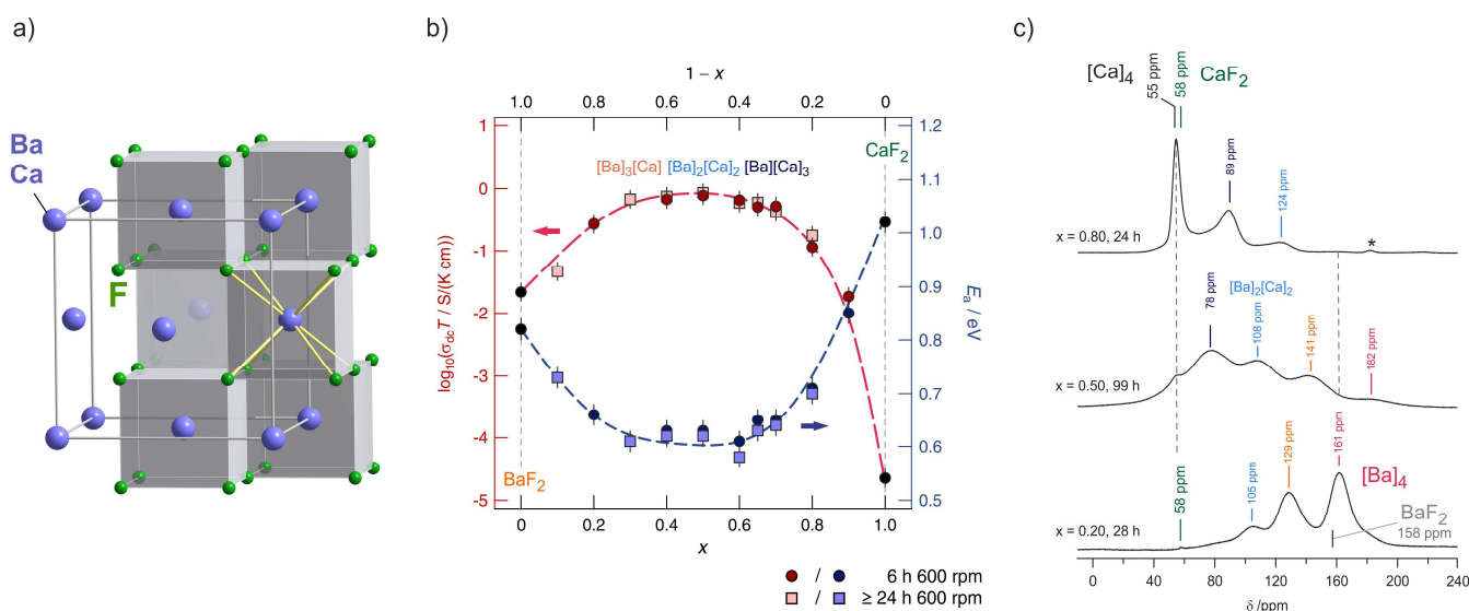
Fig. 10: a) Cubic crystal structure of (\text{Ba,Ca})\text{F}_2 . b) Variation of conductivity and activation energies for \text{Ba}_x\text{Ca}_{1-x}\text{F}_2 samples mechanically prepared by milling the starting materials for 6 h and > 24 h in a planetary mill. c) ^{19}\text{F} MAS spectra revealing the local magnetic environments sensed by the F anions. The maximum in structural disorder is reached if x = 0.5 . Figures b,c) adapted from ref. 53.
