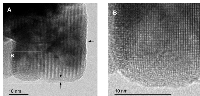
Fig. 8: High-resolution TEM image of nanocrystalline (\text{Ba,Sr})\text{LiF}_3 directly obtained by high-energy ball milling. The enlargement (B) reveal structurally disordered regions at the grain boundaries. Figure taken from ref. 52.
