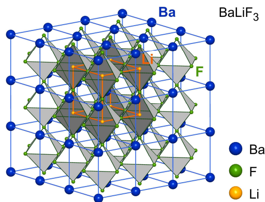
Fig. 6: Crystal structure of the inverse perovskite \text{BaLiF}_3 , the smaller Sr-atoms in (\text{Ba,Sr})\text{LiF}_3 occupy the same sites as Ba. This leads to lattice contraction and local distortions affecting fluorine ion dynamics. Figure adapted from ref. 55.
