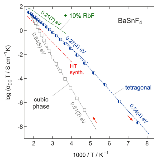
Fig. 15: Arrhenius diagram of the ionic conductivity of \text{BaSnF}_4 samples. The mechanochemical synthesis yield a metastable, cubic modification that starts to transform into the highly conductive tetragonal form at 483 K which can be seen by the inflection of the data points (grey empty cubes). The nanocrystalline tetragonal modification shows the highest conductivity of \text{BaSnF}_4 reported in the literature so far. The red, dotted line corresponds to the same material synthesized by high temperature (HT) methods. The conductivity of the material can be further increased by substitution of \text{Ba}^{2+} with monovalent \text{Rb}^+ , which is represented by the green line in the diagram.
