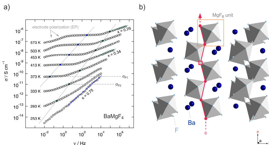
Fig. 13: a) Conductivity isotherms of mechano-synthesized \text{BaMgF}_4 in a one-pot route. The slope of the isotherms at higher temperatures was close to 0.3 which is associated with low dimensional (1D) transport. b) Crystal structure of \text{BaMgF}_4 : the corner sharing \text{MgF}_6 -octahedra form a diffusion pathway along the c -axis. Kannan et al. investigated oriented single crystals and reported on the highest conductivity along the c -axis. Figures adapted from ref. 29.
