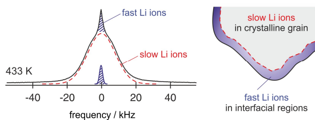
Fig. 2: {}^7\text{Li} NMR spectrum of nanocrystalline \text{Li}_2\text{O} prepared by high-energy ball milling. The line is composed of two contributions reflecting the slow and the fast ions in either the bulk or in/near the interfacial regions. Figure adapted from ref. 14.
