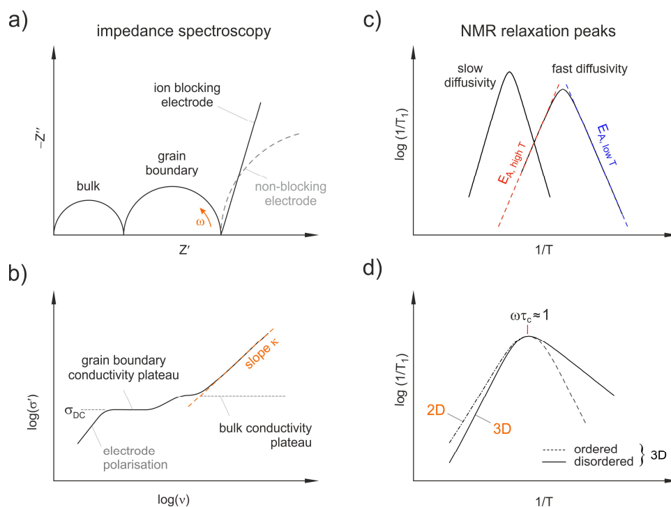
Fig. 4: Overview of important representations of impedance spectroscopy and solid state NMR data. a) Nyquist plot of the real part vs the imaginary part of the complex impedance. In the ideal case electrical responses of bulk and grain boundary regions can be distinguished; electrode effects are expected to show up at low frequencies. A spike at low frequencies results from the piling up of ions at the blocking electrode interface; conducting electrodes usually appear as large semicircles. b) The conductivity isotherm reveal the same features: at the highest frequencies a disperse regime shows up that includes forward-backward jumps. Each plateau reflects an individual transport process. c) Arrhenius plot of the NMR spin-lattice relaxation rate 1/T_1 ; the higher the diffusivity the more the peak is sifted towards lower T . The flanks yield activation energies reflecting local ( E_{A, low T} ) and long-range ion dynamics ( E_{A, high T} ). d) Structural disorder results in asymmetric rate peaks with a lower slope in the low- T regime. Dimensionality effects influence the NMR rates at higher temperatures only.
