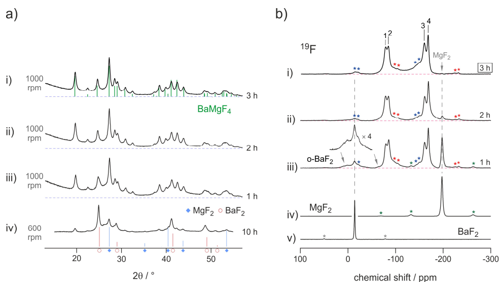
Fig. 14: Comparison of the information obtained from a) X-ray powder diffraction and b) ^{19}\text{F} solid state MAS NMR. The residual starting materials cannot be identified by XRPD (a) but were identified by MAS NMR. The latter one was used to follow the synthesis procedure, which was finished after three hours, as no noteworthy amounts of pure \text{BaF}_2 or \text{MgF}_2 could be identified any longer. Figures adapted from ref. 29.
