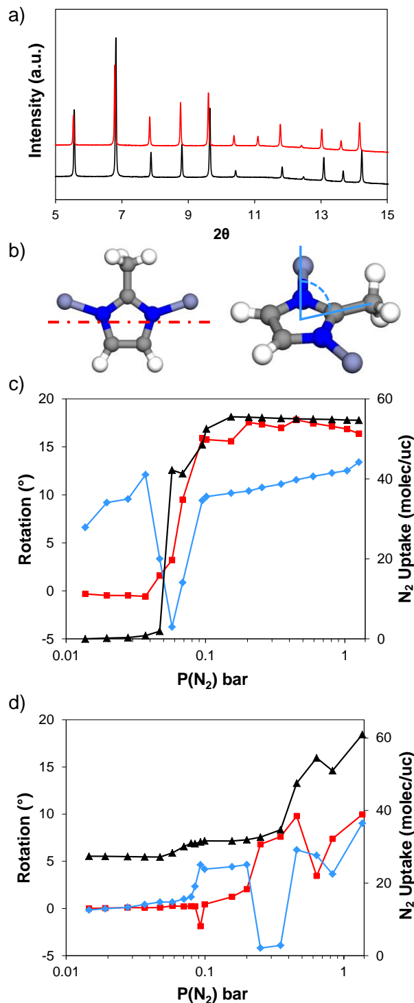
Fig. 6. a) Comparison of PXRD patterns for ZIF-8-0.14 during in situ N 2 adsorption at 0 (black line) and 0.63 bar (red line). b) Rotation of the mIM ring and methyl group respect to the mIM ring. Angle of rotation along with the amount of adsorbed N 2 molecules at different p(N_2) for c) ZIF-8-98 and d) ZIF-8-0.14. Red square, rotation of mIM ring; blue diamond, bend of the methyl group; black triangle, N 2 uptake.
