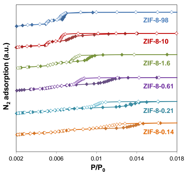
Fig. 4. Low pressure hysteresis loops of ZIF-8 samples with different particle size. Closed symbols, adsorption; open symbols, desorption.
