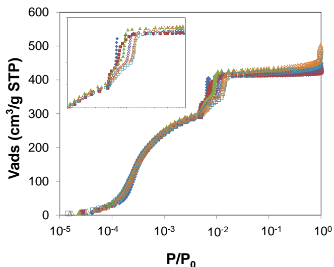
Fig. 3. Semi-log plot of N_2 adsorption isotherms at 77 K in ZIF-8 samples with different particle size. Blue closed diamonds, ZIF-98; red closed squares, ZIF-8-10; green closed triangles, ZIF-8-1.6; purple open diamonds, ZIF-8-0.61; blue open squares, ZIF-8-0.21; orange open triangles, ZIF-8-0.14.
