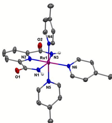
Fig. 2 X-ray crystal structure of the single-site Ru complex 4 at 50% probability level. Hydrogen atoms (except the N-H) and PF_6 have been omitted for clarity.
