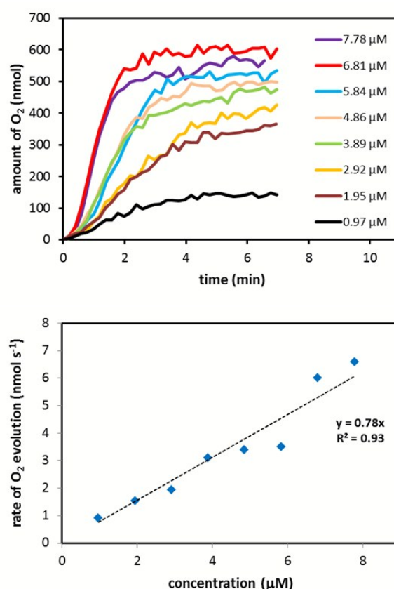
Fig. 4 (Upper) Plots of \text{O}_2 evolution versus time at various concentrations of Ru complex 4 . Reaction conditions: An aqueous phosphate buffer solution (0.1 M, pH 7.2, 0.50 mL) containing Ru complex 4 was added to the oxidant [\text{Ru}(\text{bpy})_3](\text{PF}_6)_3 (3.6 mg, 3.6 \mu\text{mol} ). (Lower) Initial rate of \text{O}_2 evolution plotted as a function of the concentration of Ru complex 4 .
