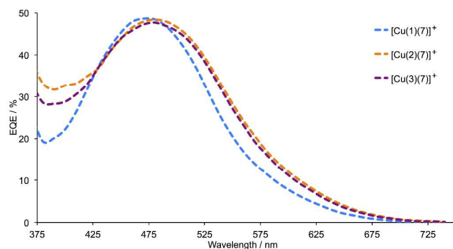
Fig. 11. EQE spectra for DSCs with [\text{Cu}(\text{L}_{\text{anchor}})(7)]^+ ( \text{L}_{\text{anchor}} = 1, 2 and 3 ) on commercial FTO/ \text{TiO}_2 electrodes, recorded on the day of assembling the DSCs.
