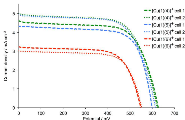
Fig. 4. J - V curves for duplicate DSCs with [\text{Cu}(1)(4)]^+ , [\text{Cu}(1)(5)]^+ and [\text{Cu}(1)(6)]^+ , recorded one day after DSC fabrication.
