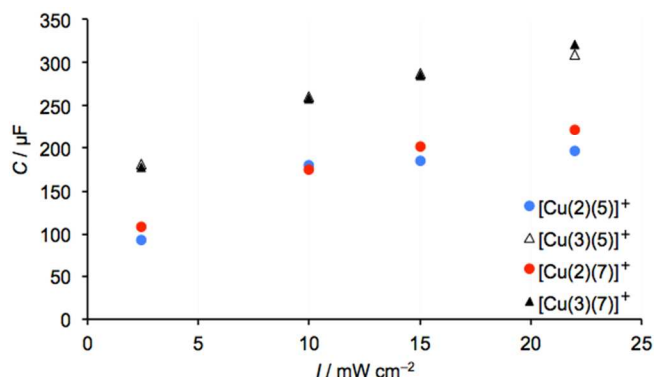
Fig. 17. Capacitance values of 3-day old DSCs containing dyes [\text{Cu}(2)(5)]^+ , [\text{Cu}(3)(5)]^+ , [\text{Cu}(2)(7)]^+ and [\text{Cu}(3)(7)]^+ .
