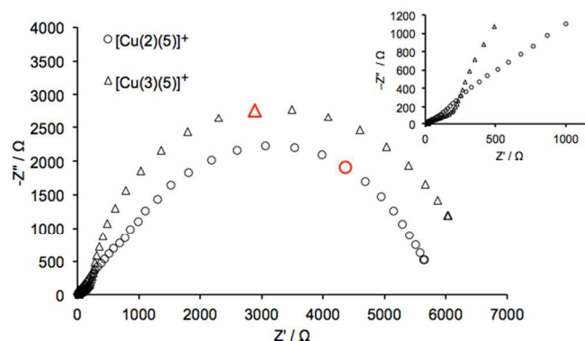
Fig. 18. Nyquist plots for [\text{Cu}(2)(5)]^+ and [\text{Cu}(3)(5)]^+ measured under a light intensity of 0.44 \text{ mW cm}^{-2} . The data points shown in red were measured at 0.3 Hz. The inset shows an expansion of the data measured in the high-to-mid frequency region.
