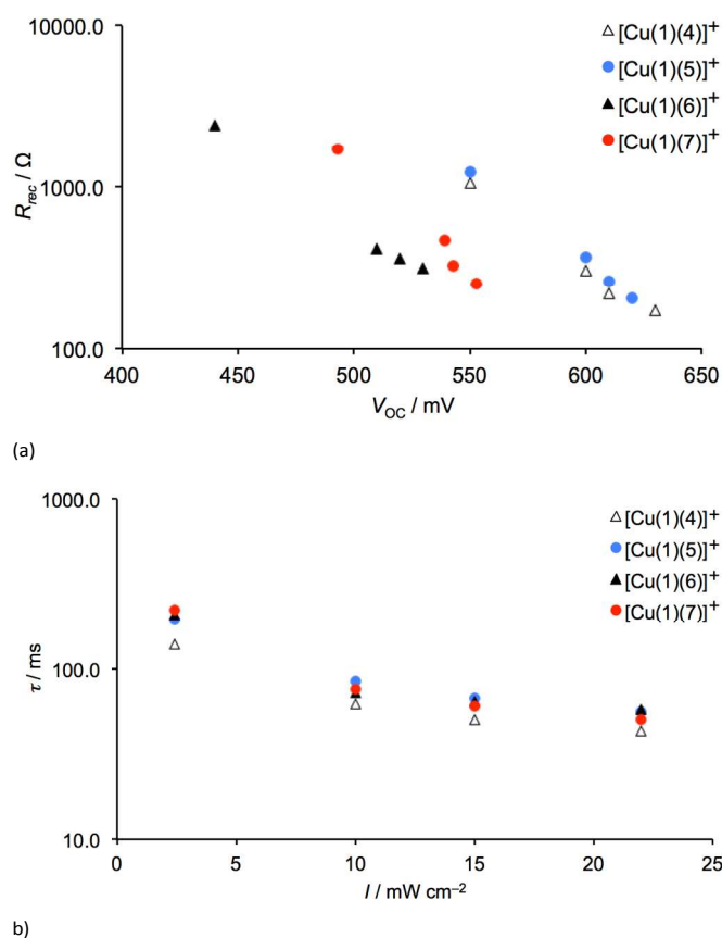
(Fig. 13. (a) The recombination resistance as a function of V_{OC} and (b) the electron lifetime as a function of bias-light intensity in 3-day old DSCs containing dyes [Cu(1)(4)] + , [Cu(1)(5)] + , [Cu(1)(6)] + , [Cu(1)(7)] + .
