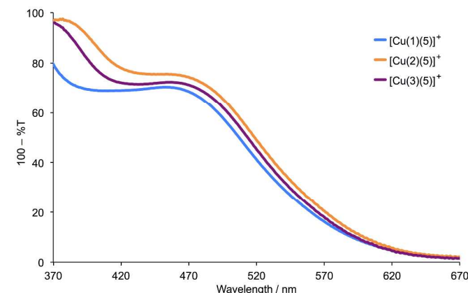
Fig. 6. Solid-state absorption spectra of FTO/ \text{TiO}_2 electrodes with adsorbed dyes [\text{Cu}(1)(5)]^+ , [\text{Cu}(2)(5)]^+ and [\text{Cu}(3)(5)]^+ . The spectra were recorded in transmission mode, and data are presented as 100-%T for ease of interpretation of \lambda_{\text{max}} .
