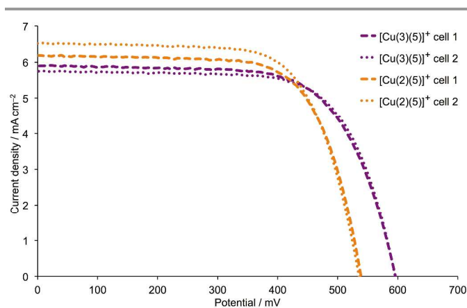
Fig. 9. J - V curves for duplicate DSCs with [\text{Cu}(\mathbf{2})(\mathbf{5})]^+ and [\text{Cu}(\mathbf{3})(\mathbf{5})]^+ dyes on in-house screen-printed FTO/TiO 2 electrodes, recorded on the day of DSC assembly.
