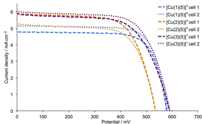
Fig. 7. J - V curves for duplicate DSCs with [\text{Cu}(\mathbf{1})(\mathbf{5})]^+ , [\text{Cu}(\mathbf{2})(\mathbf{5})]^+ and [\text{Cu}(\mathbf{3})(\mathbf{5})]^+ and commercial FTO/TiO 2 electrodes, recorded on the day of DSC fabrication.
