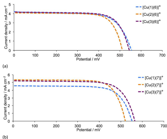
Fig. 10. J - V curves for DSCs with (a) [Cu(L anchor )(6)] + and (b) [Cu(L anchor )(7)] + dyes (L anchor = 1, 2 and 3) on commercial FTO/TiO 2 electrodes, recorded on the day of DSC assembly. See also Fig. S8†.
