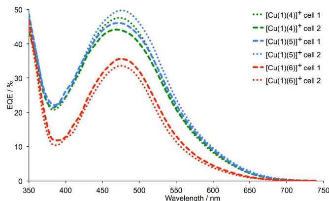
Fig. 5. EQE spectra for duplicate DSCs with [\text{Cu}(1)(4)]^+ , [\text{Cu}(1)(5)]^+ and [\text{Cu}(1)(6)]^+ , recorded one day after DSC fabrication.
