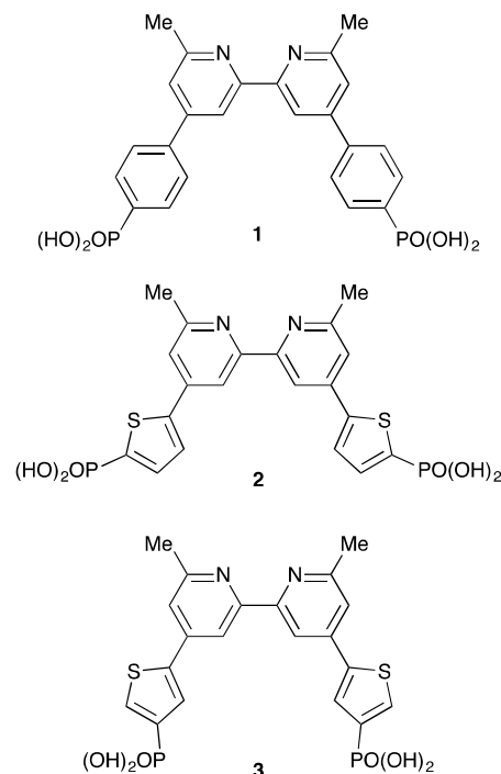
Scheme 2. Structures of anchoring ligands 1-3 .
