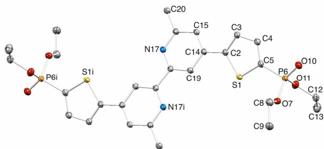
Fig. 2. Structure of 2a ; ellipsoids plotted at 40% probability level and H atoms omitted for clarity. Symmetry code i = 1-x, -y, 1-z . Selected bond parameters: S1–C2 = 1.731(2), S1–C5 = 1.718(2), C5–P6 = 1.780(2), P6–O7 = 1.5782(17), P6–O10 = 1.4644(18), P6–O11 = 1.5726(18) Å; C2–S1–C5 = 91.86(11), C5–P6–O7 = 107.07(10), C5–P6–O10 = 112.57(11), O7–P6–O10 = 115.04(10), C5–P6–O11 = 101.27(10), O7–P6–O11 = 101.80(9), O10–P6–O11 = 117.54(10)°.
