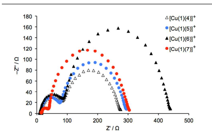
Fig. 14. Nyquist plots for 3-day old DSCs containing dyes [\text{Cu}(1)(4)]^+ , [\text{Cu}(1)(5)]^+ , [\text{Cu}(1)(6)]^+ , [\text{Cu}(1)(7)]^+ measured with a bias-light intensity of 22 \text{ mW cm}^{-2} .
