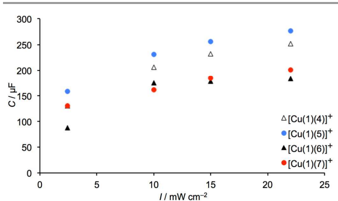
Fig. 15. Capacitance values of 3-day old DSCs containing dyes [\text{Cu}(1)(4)]^+ , [\text{Cu}(1)(5)]^+ , [\text{Cu}(1)(6)]^+ , [\text{Cu}(1)(7)]^+ .
