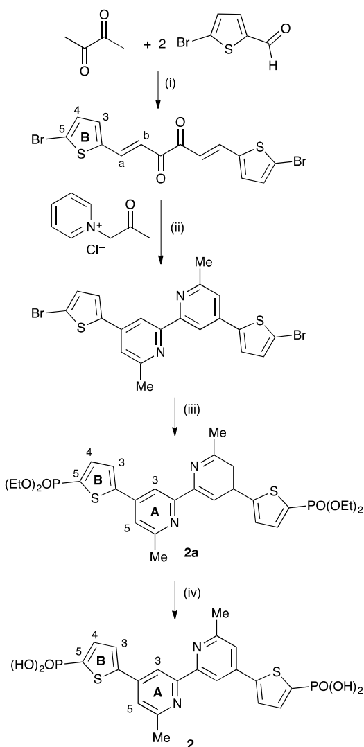
Scheme 4. Synthetic route to compound 2 . Conditions: (i) reflux in MeOH with piperidine, 2h; (ii) \text{NH}_4\text{OAc} , EtOH, reflux, 4h; (iii) \text{Cs}_2\text{CO}_3 , [\text{Pd}(\text{PPh}_3)_4] , \text{HPO}(\text{OEt})_2 in THF, microwave reactor, 90 °C, 2h; (iv) \text{Me}_3\text{SiBr} , \text{CH}_2\text{Cl}_2 . The route to 3 is analogous, with the corresponding diester labelled 3a .
