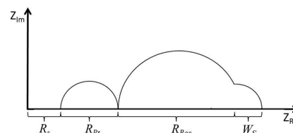
Fig. 12. Schematic representation of a Nyquist plot. R_s is the electrical resistance in cables, contacts and the resistance of the semi-conductor/FTO glass. R_{pt} is the charge transfer resistance of the interface cathode/electrolyte. R_{rec} is the electron recombination resistance of the active layer/electrolyte and W_s is the Warburg short resistance of the ion diffusion in the electrolyte close to the active layer surface.
