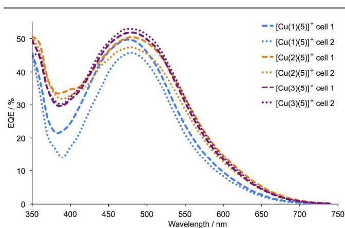
Fig. 8. EQE spectra for duplicate DSCs with [\text{Cu}(\mathbf{1})(\mathbf{5})]^+ , [\text{Cu}(\mathbf{2})(\mathbf{5})]^+ and [\text{Cu}(\mathbf{3})(\mathbf{5})]^+ and commercial FTO/TiO 2 electrodes, recorded on the day of DSC assembly.
