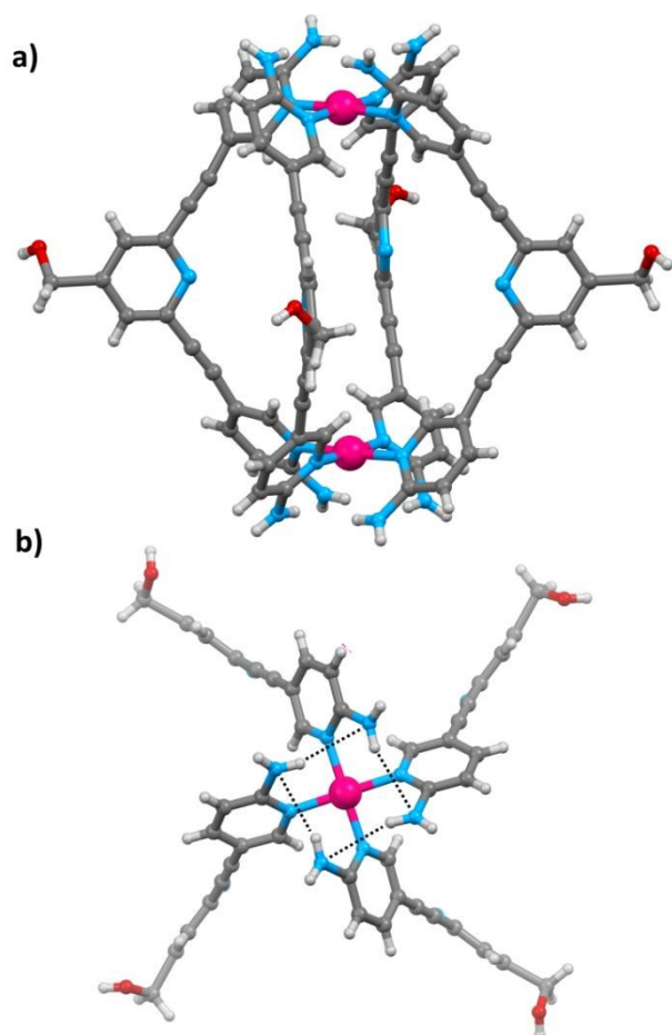
Figure 2. Molecular structure of [Pd 2 ( 2A-tripty ) 4 ] 4+ cations determined using X-ray crystallography: a) a ball-and-stick representation of [Pd 2 ( 2A-tripty ) 4 ] 4+ cation; b) a partial view of the [Pd 2 ( 2A-tripty ) 4 ] 4+ cation from the top showing the hydrogen bonding interactions between the 2-amino substituents of the ligands. Solvent molecules and counterions omitted for clarity. Colours: magenta = palladium, grey = carbon, white = hydrogen, blue = nitrogen, red = oxygen.
