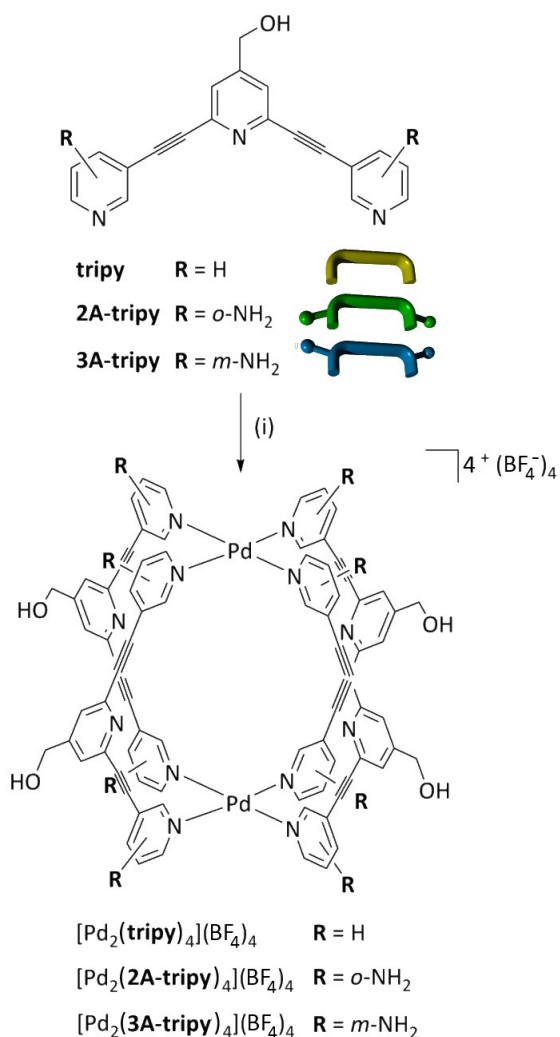
Scheme 1. Synthesis of the [\text{Pd}_2(\text{Ltripy})_4]^{4+} cages from the tripyridyl ligands ( tripy , 2A-tripy , 3A-tripy ). Conditions: (i) [\text{Pd}(\text{CH}_3\text{CN})_4](\text{BF}_4)_2 , solvent ( \text{CH}_3\text{CN} , DMF or DMSO), RT or 50 °C.
