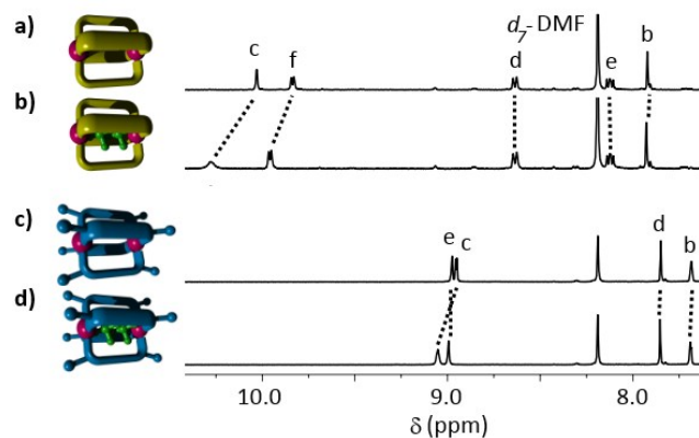
Figure 4. Partial ^1\text{H} NMR spectra (298 K, 500 MHz, d_7 -DMF) of a) [\text{Pd}_2(\mathbf{tripty})_4](\text{BF}_4)_4 , b) [(\text{cisplatin})_2\subset\text{Pd}_2(\mathbf{tripty})_4](\text{BF}_4)_4 and c) [\text{Pd}_2(\mathbf{3A-tripty})_4](\text{BF}_4)_4 and d) [(\text{cisplatin})_2\subset\text{Pd}_2(\mathbf{3A-tripty})_4](\text{BF}_4)_4 .
