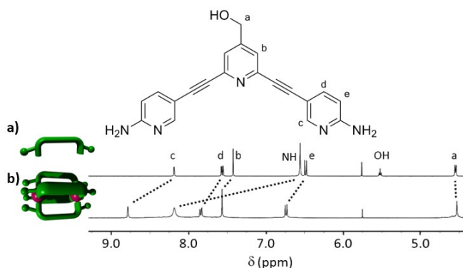
Figure 1. Partial 1 H NMR spectra (298 K, 500 MHz, d 6 -DMSO) of a) 2A-tripy and b) the cage [\text{Pd}_2(\mathbf{2A-tripy})_4](\text{BF}_4)_4 .
