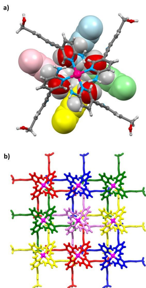
Figure 3. The crystal packing of [Pd 2 ( 2A-tripy ) 4 ] 4+ cations showing a) the interdigitation of the methylene alcohol substituents on adjacent [Pd 2 ( 2A-tripy ) 4 ] 4+ cations into the central cavity of the [Pd 2 ( 2A-tripy ) 4 ] 4+ cation (cage shown in ball-and-stick, methylene alcohol substituents in spacefilling view, and b) the extended lattice.
