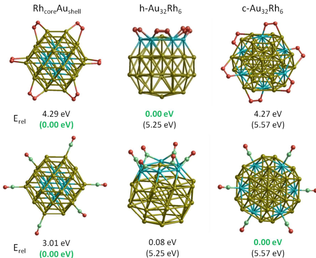
Figure 10. Stability ordering change of \text{Au}_{32}\text{Rh}_6 cluster upon adsorption of 6 \text{O}_2 and 6 \text{CO} molecules. E_{\text{rel}} is the energy relative to the \text{Rh}_{\text{core}}\text{Au}_{\text{shell}} isomer. Numbers in parentheses show the relative energies without \text{O}_2 molecules.
