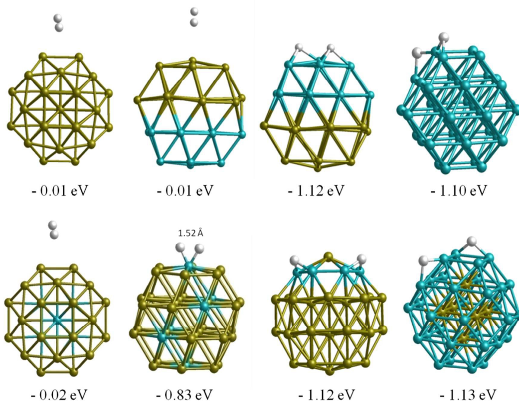
Figure 5. H 2 molecule adsorption configurations and energies on TO 38 clusters.
