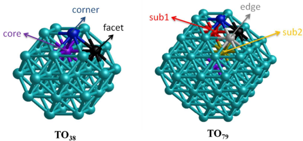
Figure 1. Symmetrical positions on 38- and 79-atom TO cluster models.
