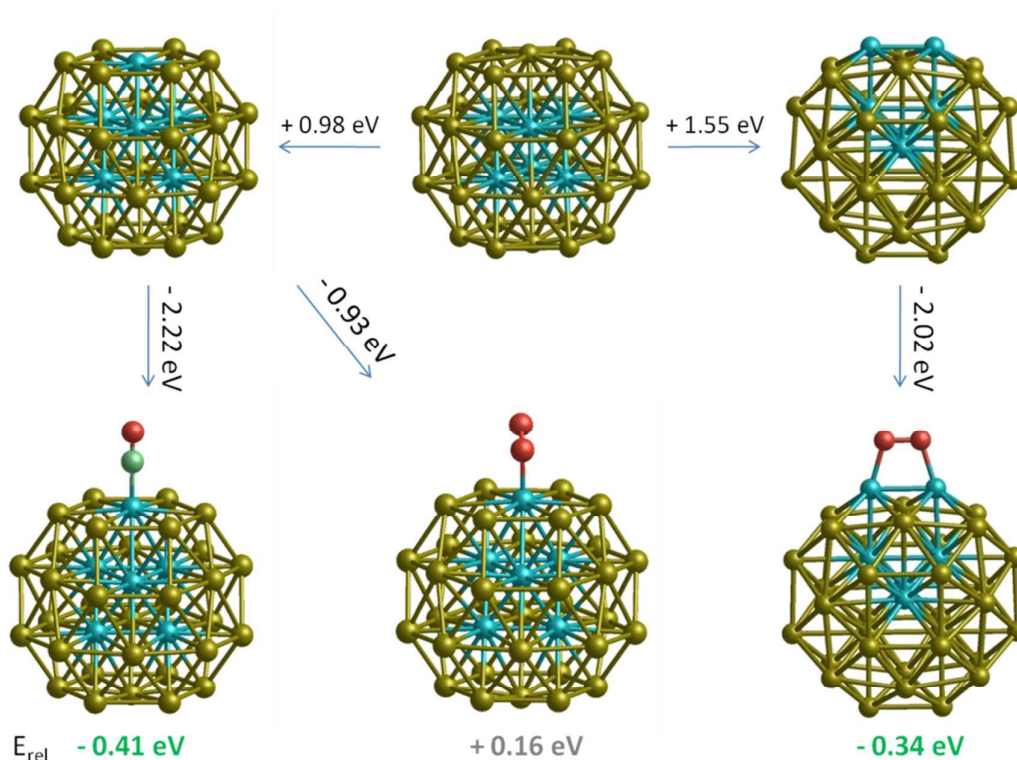
Figure 11. Energy changes for swapping one or two Rh core atoms with surface gold atoms for the bare \text{Rh}_{\text{core}}\text{Au}_{\text{shell}} cluster and in the presence of adsorbed CO and \text{O}_2 . E_{\text{rel}} is the energy relative to the \text{Rh}_{\text{core}}\text{Au}_{\text{shell}} cluster, including the adsorbate.
