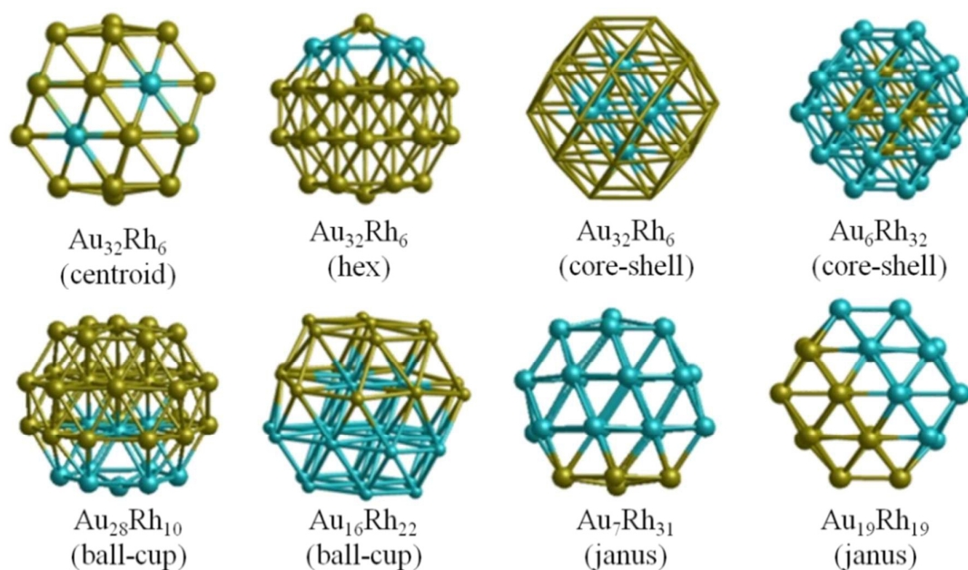
Figure 2. 38-atom TO Au-Rh nanoalloy models showing several compositions and chemical orderings.
