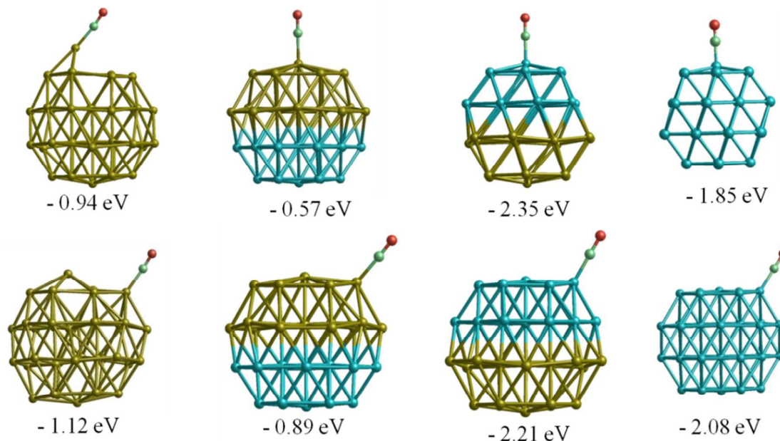
Figure 7. CO adsorption in atop positions on Au, Rh, and Janus clusters. Adsorption energies are given in eV.
