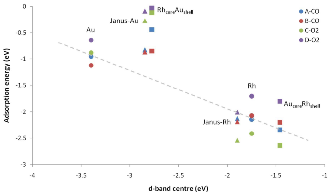
Figure 8. Adsorption energy versus d-band centre for CO and O 2 adsorption on Au, Rh, Au core Rh shell , Rh core Au shell , and Janus particles. Circles, squares and triangles represent adsorption on pure, core-shell and Janus particles. A-CO, B-CO, C-O 2 and D-O 2 denote \mu_2\eta^1 (111)-(111), \mu_1\eta^1 corner, \mu_2\eta^2 (111)-(111), and \mu_2\eta^2 (111) adsorption sites, respectively. The dashed line is a guide for the eye.
