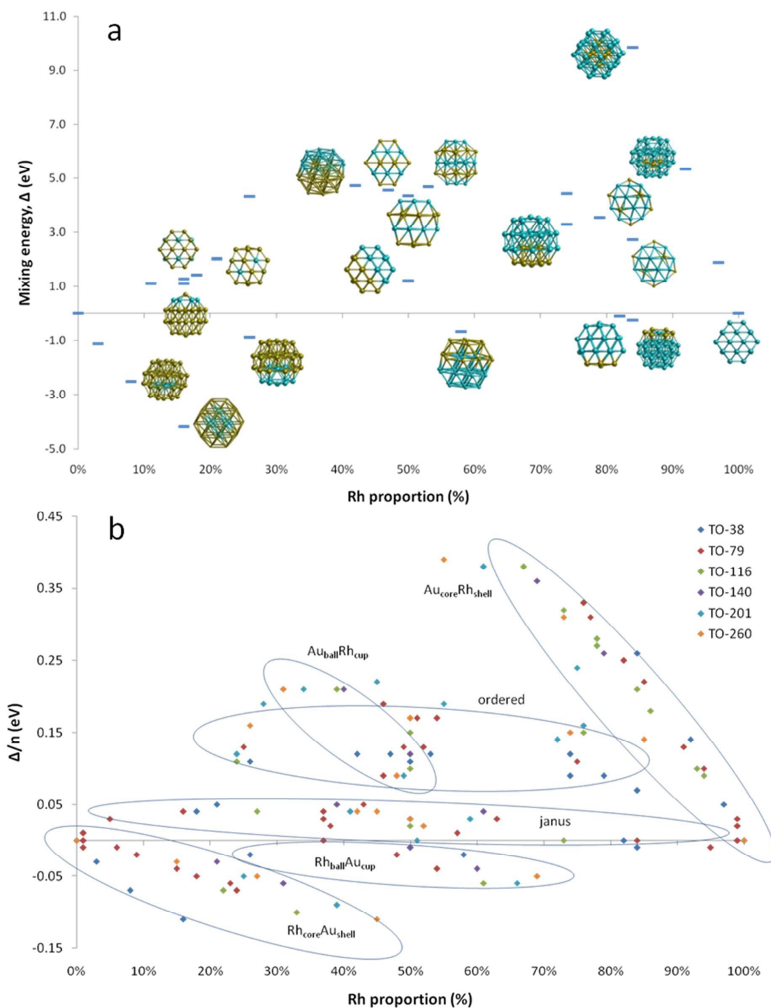
Figure 4. (a) Mixing energy ( \Delta ) versus atomic composition for 38-atom TO nanoalloys. Corresponding structures are shown. Blue spheres represent Rh atoms and yellow spheres represent Au atoms. (b) Mixing energy per atom ( \Delta/n ) versus atomic composition for all considered TO sizes. Ellipses are a guide to eye.
