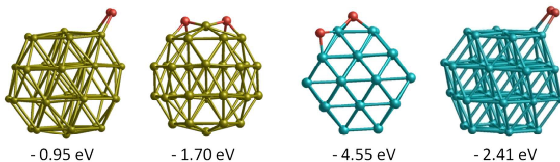
Figure 6. Adsorption energies and structures of both molecular and dissociated O_2 on Au_{38} and Rh_{38} clusters.
