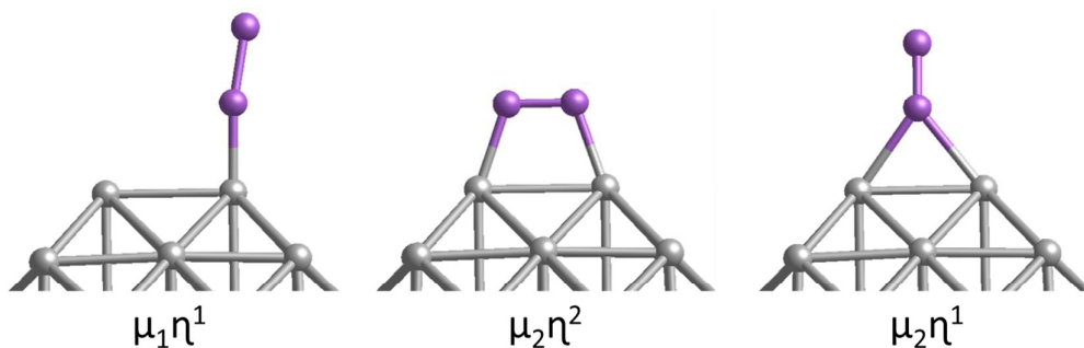
Figure 3. Metal adsorbate bonding types. The symbol \mu stands for the number of metal atoms to which the adsorbate binds and the symbol \eta stands for the number of atoms in the adsorbate which bind to the metal. Grey spheres represent metal atoms and purple spheres represent adsorbate atoms.
