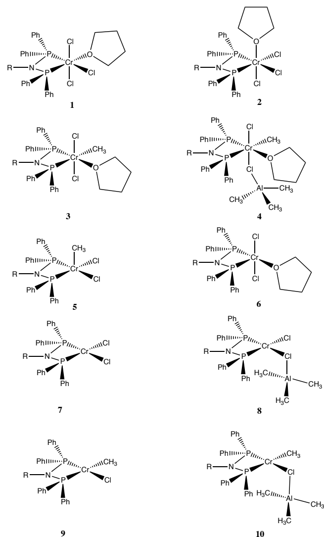
Fig. 2 Structures considered for the reaction of [CrCl 3 {PPh 2 N(R)PPh 2 }(THF)] 1 (a R=Pr, b R=Me) with AlMe 3 .
