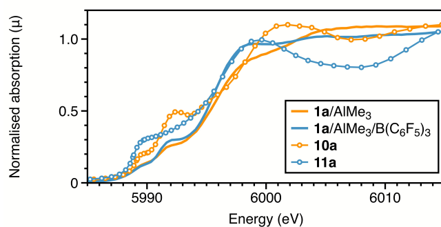
Fig. 8. Cr K-edge XANES: experimental and calculated spectra of 1a with \text{AlMe}_3 with and without \text{B}(\text{C}_6\text{F}_5)_3 .
