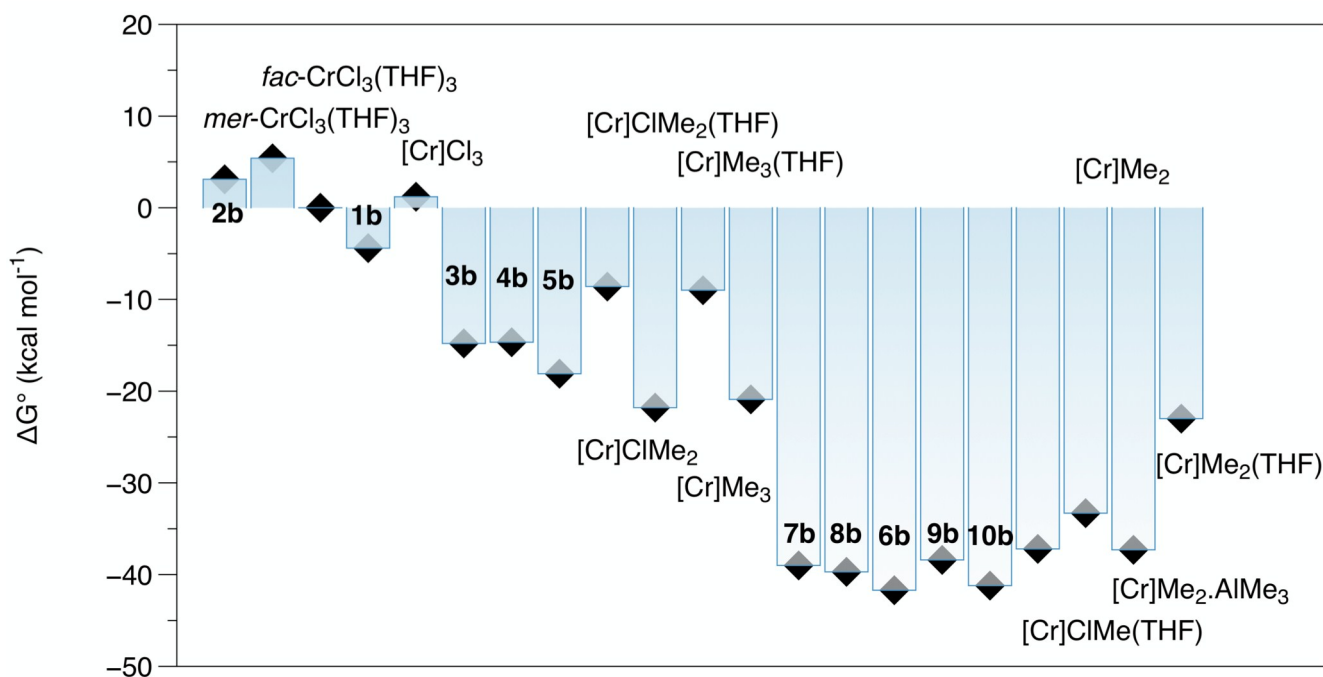
Fig. 3. \Delta G^\circ calculated by EDF2/6-31G* for reactions from \text{CrCl}_3(\text{THF})_3 , (\text{PPh}_2)_2\text{NMe} and \text{Al}_2\text{Me}_6 . Compound numbers as in Fig. 2, [\text{Cr}] = \text{Cr}(\text{PPh}_2(\text{NMe})\text{PPh}_2) . Cr(III) and Cr(II) complexes S=3/2 and S=2 , respectively.
