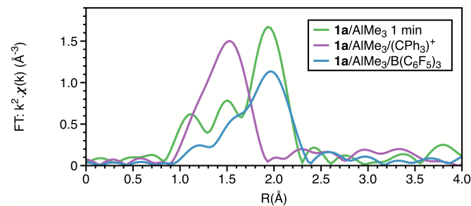
Fig. 6. Cr K-edge Fourier transforms of k^2 -weighted EXAFS data of reactions of 1a with 20 AlMe_3 (1 min); 1a + 30 AlMe_3 + 1 [Ph_3C][Al\{OC(tBu^F)_3\}_4] ; 1a + 30 AlMe_3 + 1 B(C_6F_5)_3 .
