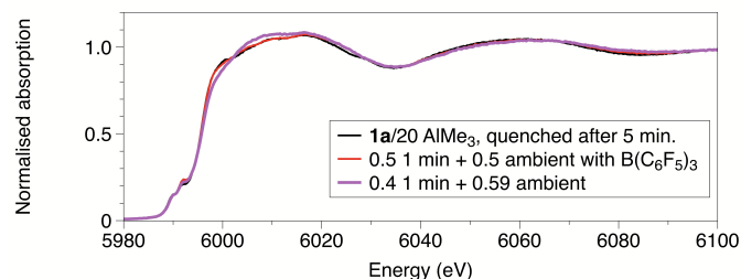
Fig. 5. Comparison of the experimental Cr K-edge XANES of the reaction quenched after 5 minutes with spectra of a combination of a) a 2:3 combination of the spectrum from a sample quenched after 1 minute, and of the room temperature measurement and b) a 1:1 combination of the spectrum from a sample quenched after 1 minute, and of the room temperature measurement with solution containing B(C_6F_5)_3 .
