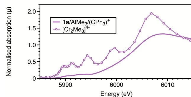
Fig. 7. Cr K-edge XANES: experimental and calculated spectra of 1a with AlMe_3 with (CPh_3)[Al\{OC(tBu^F)_3\}_4] .
