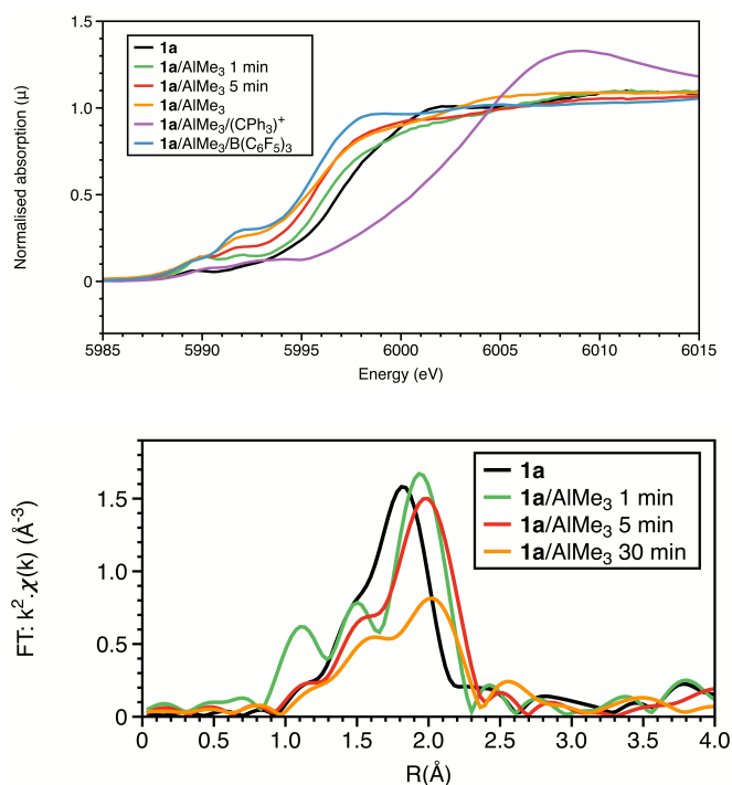
Fig. 1. At the Cr K-edge: (Top) XANES and (bottom) Fourier transforms of k^2 -weighted EXAFS data. Reactions performed at ambient temperature, some quenched by liquid nitrogen after a set reaction time.
