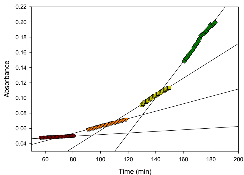
Figure 8. Initial rates of reaction profile at various temperature based on the absorbance of the \nu(\text{C}=\text{O}) of the propylene carbonate (PC). \bullet At 50 °C ( y = 0.0001066x + 0.04121 , R^2 = 0.9838 ), \blacktriangledown At 60 °C ( y = 0.0004866x + 0.01444 , R^2 = 0.9987 ), \blacksquare At 70 °C ( y = 0.001141x - 0.05657 , R^2 = 0.9971 ), \blacklozenge At 80 °C ( y = 0.002372x - 0.2107 , R^2 = 0.988 ).
