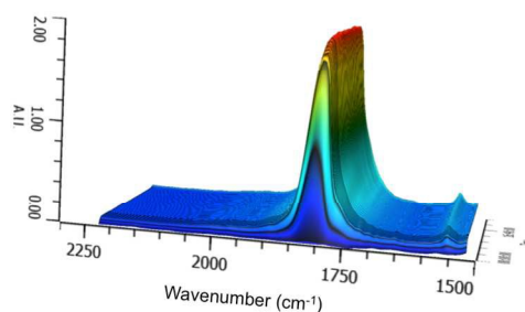
Figure 7. Three-dimensional stack plots of the IR spectra using 1 at 20 bar, 100 °C and [Fe]:[PO]:[Cocat] 1:4000:4.
