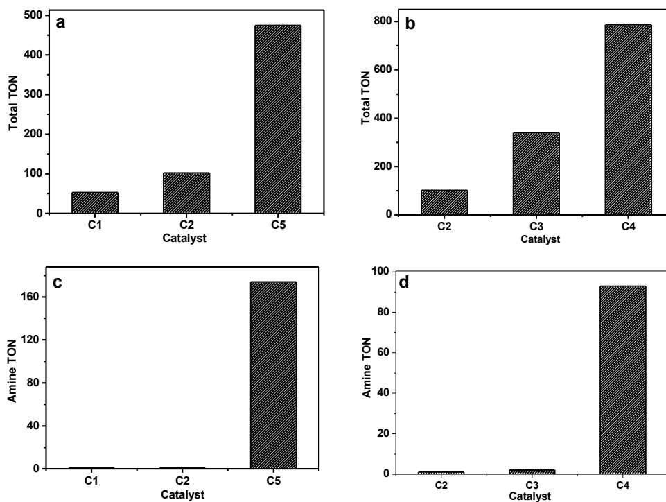
Figure 2. Comparison of TONs of monometallic and bimetallic catalysts for the tandem synthesis of 5 and 6 . (a): Ru and Pd for total TON; (b): Au and Pd for total TON; (c): Ru and Pd for amine TON and (d): Au and Pd for amine TON; Key; C1: 1%Ru/TiO 2 ; C2: 1%Pd/TiO 2 ; C3: 1%Au/TiO 2 ; C4: 1%Au-Pd/TiO 2 ; C5: 1%Ru-Pd/TiO 2 . Reaction conditions: catalyst: 0.1 g; nitrobenzene: 4.5 mmol; benzyl alcohol: 45 mmol; mesitylene (solvent): 5 mL; Ar: 20 bar; T: 433 K; t: 3 h.
