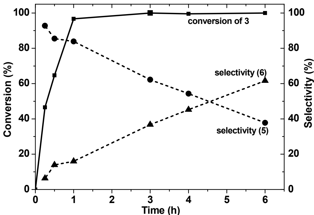
Figure 3. Time-on-line profile of the nitrobenzene conversion and product selectivity for the tandem synthesis of 5 and 6 using the 1%RuPd/TiO 2 (M 1m ) catalyst. Reaction conditions: catalyst: 0.1 g; nitrobenzene: 4.5 mmol; benzyl alcohol: 45 mmol; mesitylene (solvent): 5 mL; Ar: 20 bar; T: 433 K.
