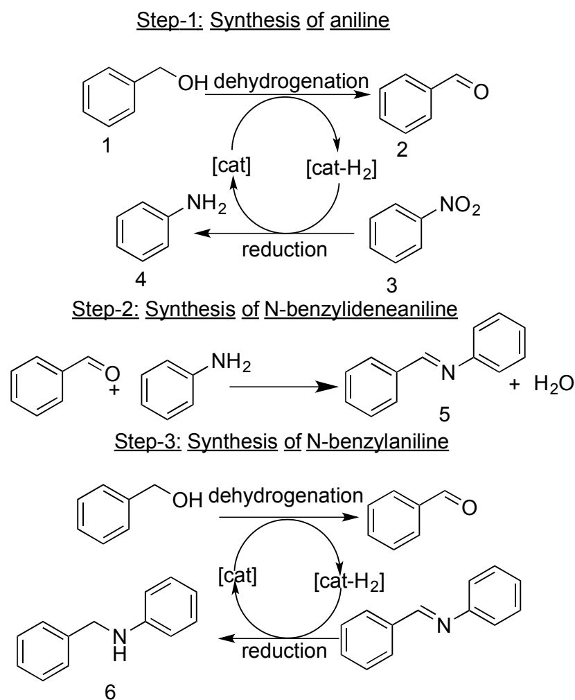
Figure 1. Sequence of reactions involved in the one-pot tandem synthesis of N -benzylideneaniline (5) and N -benzylaniline (6) from nitrobenzene (3) and benzyl alcohol (1).
