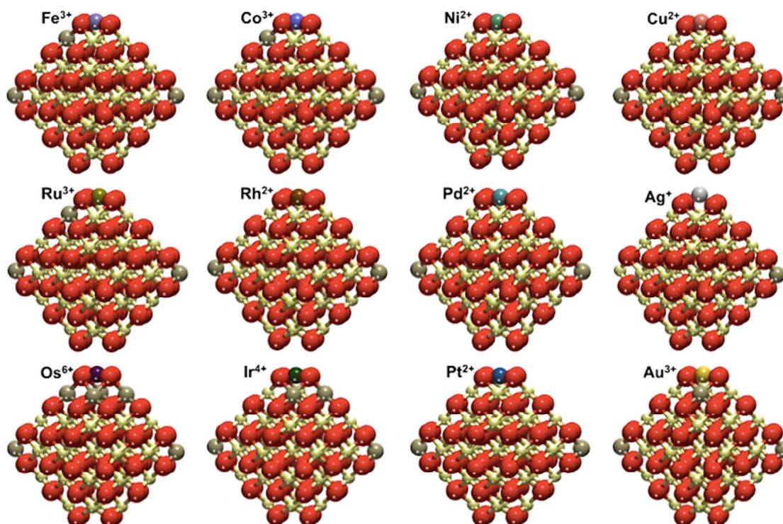
Figure 3. Overview of the M_1 - Ce_{40}O_{80} structures calculated for the adsorption of different transition metal atoms (M) on the {100} facet of the Ce_{40}O_{80} nanoparticle. Yellow, brown and red spheres represent Ce^{4+} , Ce^{3+} and O^{2-} ions, respectively. See selected calculated interatomic distances in Figs. S1 and S2.
