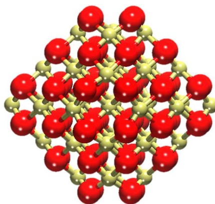
Figure 1. Cuboctahedral Ce 40 O 80 nanoparticle model of nanostructured ceria. Yellow and red spheres represent Ce 4+ cations and O 2- anions, respectively.
