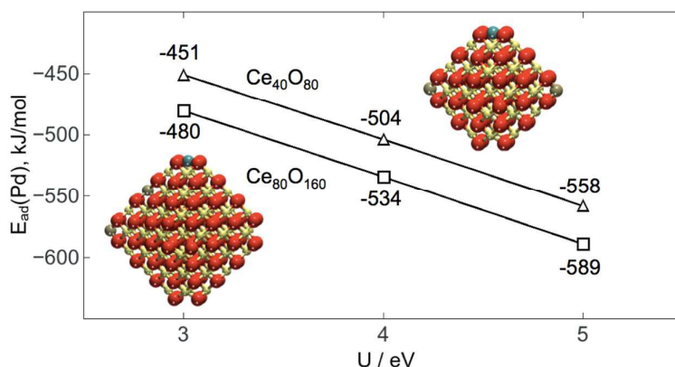
Figure 4. Calculated adsorption energies E_{ad}(\text{Pd}) of single Pd atoms on the \text{O}_4 site of \text{Ce}_{40}\text{O}_{80} and \text{Ce}_{80}\text{O}_{160} NPs as a function of the U value used with the PW91 functional.
