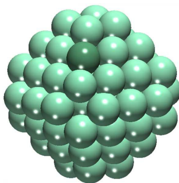
Figure 2. Model \text{M}_{79} NP used for estimating the binding energy of atoms in metal particles. The darker green M atom in edge position was removed for calculating its binding energy to the remaining \text{M}_{78} species.
