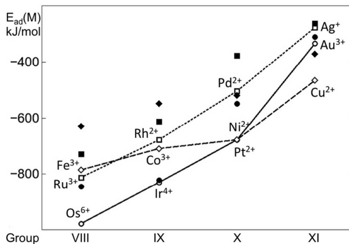
Figure 5. Adsorption energies of single transition metal atoms (M) on the {100} facet of the Ce_{40}O_{80} NP (empty points, connected for guiding eye) and binding energies of these atoms in edge positions of the M_{79} NP depicted in Fig. 2 (filled points). Results for 3d , 4d and 5d metals are shown by diamonds, squares, and circles, respectively.
