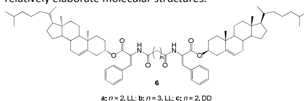
Figure 6. Molecular structures of the diacid amides of dicholesteryl L-phenylalaninate 6 employed by Fang and co-workers. 26
