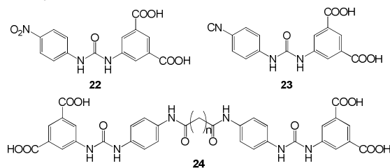
Figure 15. Chemical structure of urea based gelators 22-24 developed by Hayes, Miravet, Escuder and co-workers for dye adsorption. 48,49
