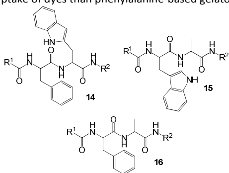
Figure 12. Chemical structures of dipeptide gelators 14-16 reported by Das and co-workers – those including tryptophan groups have the best dye adsorption characteristics.
