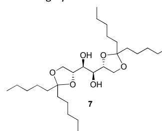
Figure 7 Gelator 7 employed by Prathap and Sureshan for the formation of mechanically robust gels in petrol and diesel.
