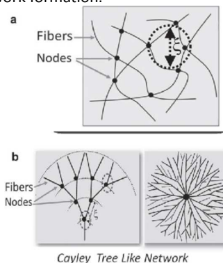
Figure 38. Illustration of fibre networks commonly observed in supramolecular materials. a) Interconnecting fibre network consisting of fibres and joints (or nodes) with closed loops. b) Cayley tree-like network (left) with open loops, and spherulites. Figure adapted from reference 113 with permission.
