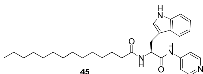
Figure 31. Pyridine-functionalised 45 which forms gels in mixed aqueous solvents in the presence of HCl. 96
