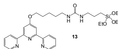
Figure 11. Chemical structure of terpyridine-based ligand 13 which forms organogels in the presence of metals, the xerogels of which are capable of dye adsorption.
