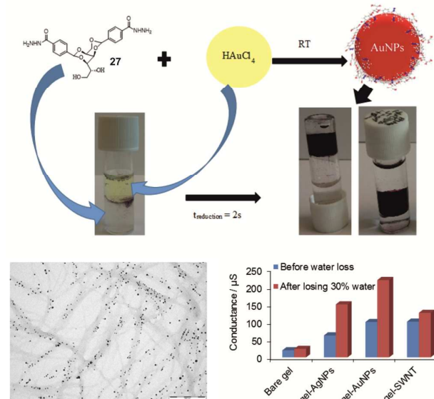
Figure 24. Scheme showing uptake of noble metal and in situ reduction to nanoparticles by hydrogel nanofibres of DBS-CONH 2 ( 27 ), TEM image showing nanoparticles aligned along gel nanofibres and enhanced conductances of the nanoparticle-embedded gels compared with bare gel, and gels containing single walled nanotubes. Figure adapted from reference 80 with permission.
