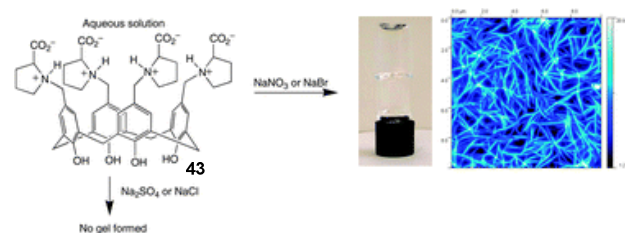
Figure 29. (a) Chemical structure of proline-functionalized calix[4]arene 43 which forms gels in the presence of nitrate or bromide anions. Figure adapted from reference 93 with permission.
