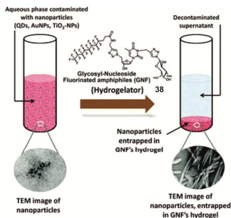
Figure 25. Schematic illustration of the removal of NPs from aqueous samples using fluorinated glycoside-nucleoside amphiphile hydrogelator 38 and TEM images of nanoparticles and GNF nanofibres with entrapped NPs. Figure adapted from reference 83 with permission.
