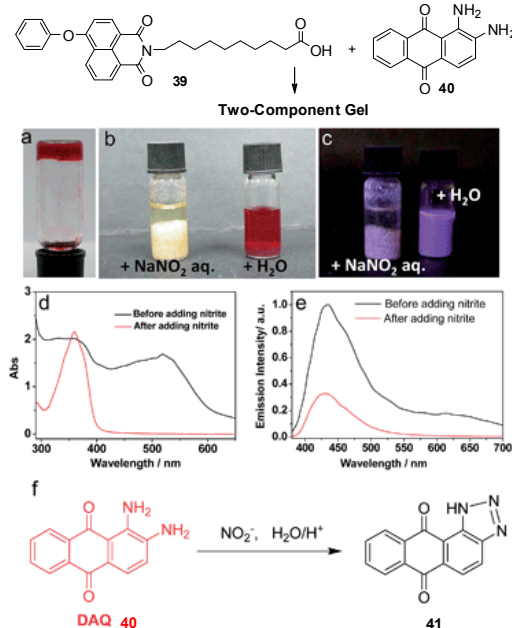
Figure 27. Chemical structure of two-component gel formed by naphthalimide undecanoic acid 39 and diaminoanthraquinone 40 . Photo of gel 39 + 40 (25 mg mL -1 in acetonitrile) (a), and the gel with added NaNO 2 solution (left) and pure water (right) (b) and with 365 nm light irradiation (c). (d) Absorption and (e) emission spectra of 39 + 40 before and after treatment with NO 2 - . (f) Reaction scheme between 40 and NO 2 - . Figure adapted from reference 90.
