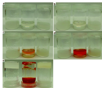
Figure 35. Chemical structure of cyclohexyl diamide 52 and photographs of gels containing compound 55d (20 mg) and DMSO (1 mL), pyridine (1 mL) and TEA (1 mL). (b) The addition of DCP (0.1 mL) to the surface of gel samples. (c) 1 h 48 min after DCP addition. (d) 2 h 58 min after DCP addition. (e) 5 h 5 min after DCP addition showing gel breakdown and intense red colour. Figure adapted from reference 101 with permission.
