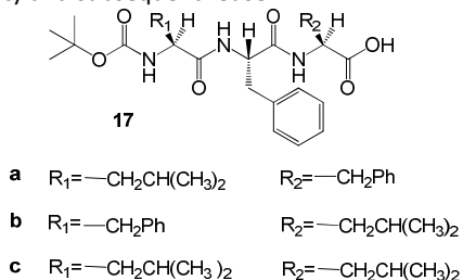
Figure 13. Structures of phenylalanine-based tripeptide gelators 17a-c . 46
