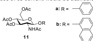
Figure 9. Structures of \beta -glycosides of N -acetyl glucosamine 11a and b . 30
