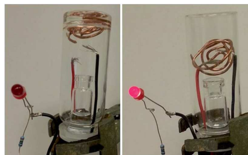
Figure 36. Structure of two-component gelator 56 and photographs: Left: copper coil suspended in organogel above the sample of DCP and positive/negative contacts; right: organogel breaks down in response to DCP, resulting in the release of copper coil, completion of the electrical circuit and the LED switching on. Figure adapted from reference 102 with permission.
