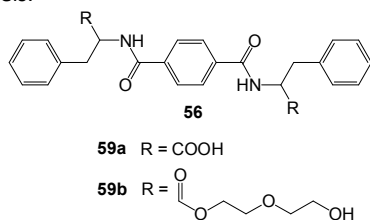
Figure 40. Chemical structures of C_2 -symmetric benzene-based gelators 59 – the nature of the R groups plays a key role in controlling network dimensions and porosity – and hence dye uptake. 116
