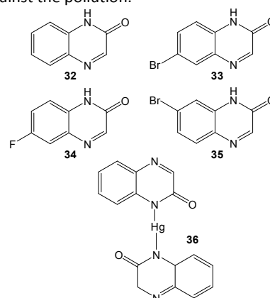
Figure 22. Chemical structures of quinoxalinone compounds 32-35 and hydrogelator complex 36 formed by complexation of compound 32 with Hg(II). 76
