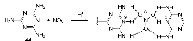
Figure 30. Melamine 44 binds the nitrate anion and forms gels when protonated – scheme shows the proposed hydrogen-bonding interactions of the complex which underpins the gel.
