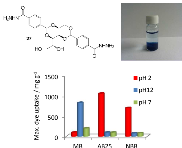
Figure 17. Chemical structure of DBS acylhydrazide (DBS-CONHNH 2 , 27 ), photograph of gel extracting methylene blue from basic water and the maximum dye adsorption onto 27 supramolecular gel under various conditions of pH. Figure adapted from reference 58 with permission.
