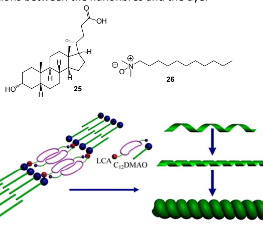
Figure 16. Chemical structures of amphiphilic lithocholic acid 25 and dodecyl (dimethyl) amine oxide 26 and schematic of the Formation of the two-component hydrogelator and the subsequent formation of a chiral aggregate. Figure adapted from reference 54 with permission.
