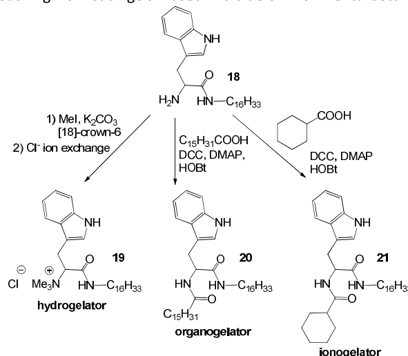
Figure 14. Tuning the amphiphilicity of a non-gelator 18 to a hydrogelator, 19 , an organogelator 20 and an ionogelator 21 by simple chemical modifications.
