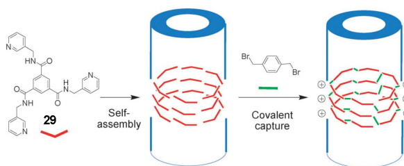
Figure 19. Self-assembling compound 29 and its covalent capture through surface crosslinking with 1,4-bis(bromomethyl)benzene. Figure adapted from reference 69 with permission.
