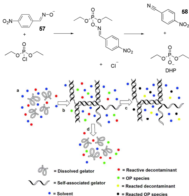
Figure 37. 4-Nitroaldehyde oxime 57 reactive nerve agent decontamination compound, the mechanism of its reaction with DCP to form 58 , and a schematic of how a gel incorporating reactive decontaminant can respond to the presence of nerve agents and act to remediate against them. Figure adapted from reference 104 with permission.
