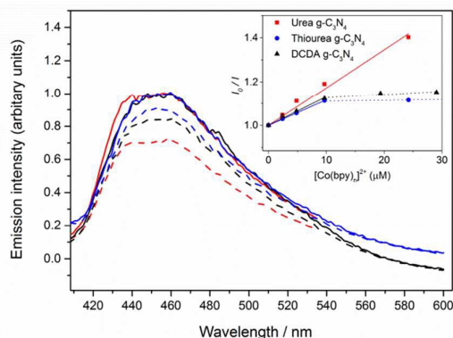
Fig. 2: Normalised emission of urea (red), DCDA (black) and thiourea (blue) derived g\text{-C}_3\text{N}_4 ( 0.1 \text{ mg ml}^{-1} in 1:1 \text{CH}_3\text{CN}/\text{H}_2\text{O} ) in the absence of a quencher (solid lines) and relative quenching in the presence of [\text{Co}(\text{bpy})_3]^{2+} (dashed lines). Inset shows the Stern-Volmer plots for g\text{-C}_3\text{N}_4 in \text{CH}_3\text{CN}/\text{H}_2\text{O} with a [\text{Co}(\text{bpy})_3]^{2+} quencher.
