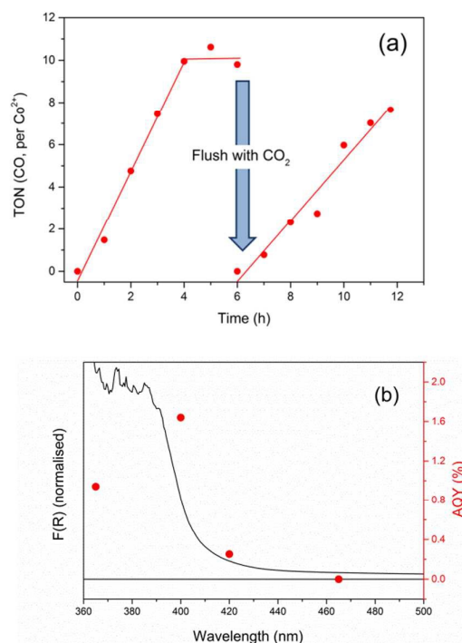
Fig. 1: Photocatalytic \text{CO}_2 reduction under (a) prolonged 400 nm LED illumination ( ca. 5 \text{ mW} \cdot \text{cm}^{-2} ). (b) AQY for CO production measured at wavelengths shown (red) and overlaid UV/Vis spectrum of the reaction suspension. Conditions: g\text{-C}_3\text{N}_4 (urea, 2.5 mg), \text{CoCl}_2 ( 50 \mu\text{mol dm}^{-3} ) and \text{bpy} ( 5 \text{ mmol dm}^{-3} ) in 5 ml \text{CH}_3\text{CN}:\text{H}_2\text{O}:\text{TEOA} , 3:1:1 purged with \text{CO}_2 .
