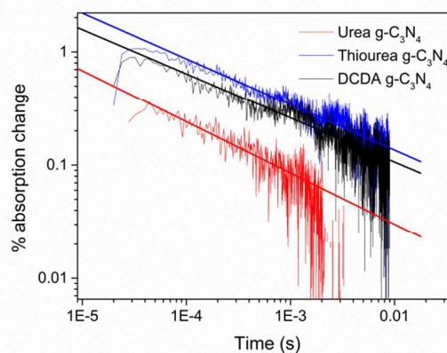
Fig. 3: DR-TA kinetic traces recorded at 850 nm for the g\text{-C}_3\text{N}_4 sample indicated under an Argon atmosphere, following UV (355 nm, 91 \mu\text{J.cm}^{-2} ) excitation.
