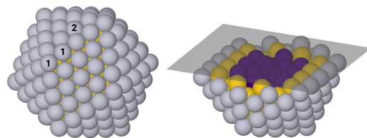
Fig. 1 Schematic showing the complete icosahedral nanoparticle (left) and the position of the cross-section at which RMSD values are projected (right). The atoms are coloured showing the Pt shell (grey), Au subsurface (yellow) and M core (purple). Adsorption sites are also denoted on the complete particle, showing the edge-bridge position (1) and the atop position (2), investigated later in the article.
