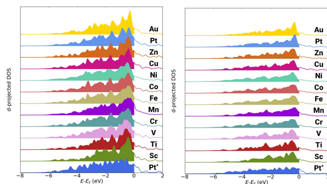
Fig. 4 Projected d -band DOS for the edge-bridge sites (Left) and atop sites (Right). The Pt 162 Au 92 M 55 nanoparticles are compared to the pure Pt 309 nanoparticle, denoted Pt*.
