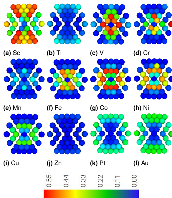
Fig. 2 RMSD plots for a cross-section of the ternary nanoparticles relative to the \text{Pt}_{309} nanoparticle. Each atom is coloured according to displacement from the range 0.00 to 0.55 Å, coloured blue to red, respectively.
