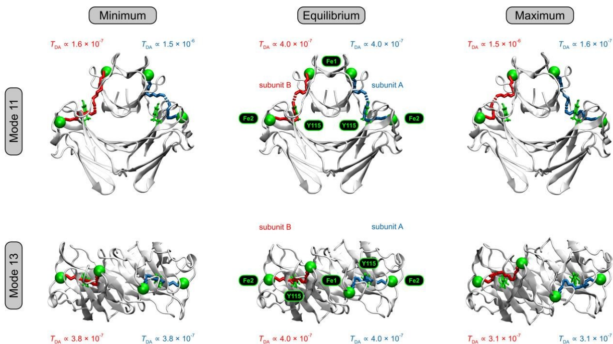
Fig 3 Effects of two low-frequency normal modes on the structure and electronic couplings of Dd 2Fe-SOR, as calculated by ENM-NMA and the pathways model. 86,90 (Top) Front view schematic representation of interdomain Fe–Fe stretching mode 11. (Bottom) Schematic representation of domain torsional mode 13, with the molecule viewed from the top along the crystallographic C_2 axis. Turning point structures where the Fe–Fe distance in subunit A and the Fe1–C1–C2–Fe2 dihedral angle is smallest (largest) are depicted on the left (right) for mode 11 and 13, respectively. The equilibrium geometry reflected by the crystal structure (pdb entry: 1DFX) 45 is shown as a reference in the centre. Electron transfer pathways corresponding to the two subunits are colour-coded, and Fe atoms of centre I and II, depicted as green spheres, are labelled Fe1 and Fe2, respectively. The quasi conserved tyrosine between both metals sites, 43,46,47 Y115 in Dd 2Fe-SOR, is shown in green. C1 and C2 are two points on the C_2 crystallographic axis (not shown). Mode amplitudes are scaled to an average RMSD of 1 Å, and dynamic representations of mode 11 and 13 are available as Animations SI 1 and SI 2, respectively.
