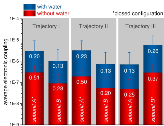
Fig 6 Statistical analysis of interdomain electronic couplings between centres I and II within one subunit, as calculated by the pathways model 86 for all three MD trajectories. Data sets derived from analyses including (excluding) water are presented in blue (red). Arithmetic means, calculated from all time steps, are represented by vertical bars, while the corresponding standard deviations are indicated by whiskers. Values of the coherence-like parameter C_p are listed as white numbers. Subunits assuming a closed configuration during the MD simulations are indicated by an asterisk.
