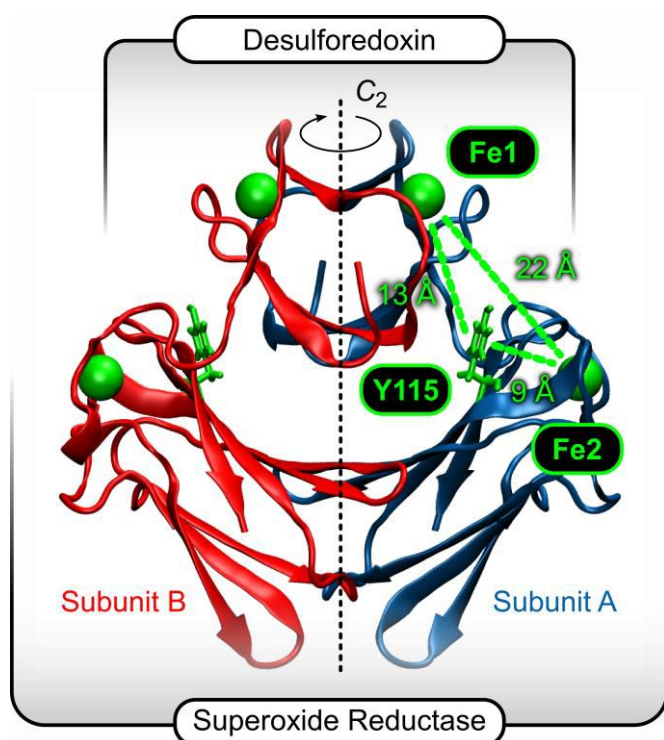
Fig 1 Crystal structure of 2Fe-SOR from Dd (pdb entry: 1DFX). 45 The crystallographic C_2 axis is drawn as a dashed vertical line, and the different domains are indicated. The two equal subunits are colour-coded, and Fe atoms of centre I and II, depicted as green spheres, are labelled Fe1 and Fe2, respectively. Y115 indicates a quasi conserved tyrosine between both metals sites, 43,46,47 and approximate distances between Fe1, Fe2, and the Y115 side chain are displayed.
