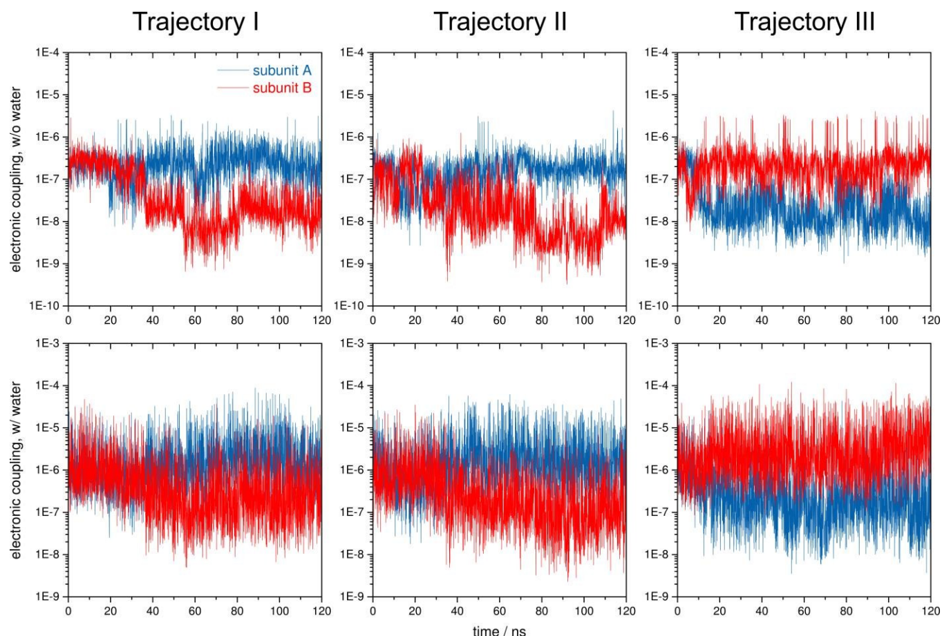
Fig 7 Time evolution of interdomain electronic couplings between centres I and II within one subunit, as calculated by the pathways model 86 for all three MD trajectories. Values corresponding to subunit A (B) are plotted in blue (red), and datasets derived from pathways analyses including (excluding) water are presented at the bottom (top).
