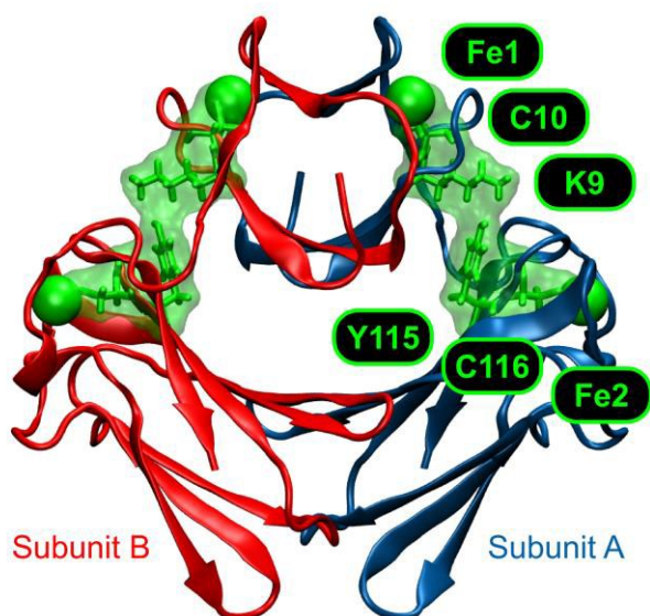
Fig 8 Crystal structure of 2Fe-SOR from Dd (pdb entry: 1DFX) 45 visualizing the dominating route for intramolecular electron transfer between centres I and II within one subunit (green surface). Involved amino acids are shown in stick representation and labelled in one letter code. The two equal subunits are colour-coded, and Fe atoms of centre I and II, depicted as green spheres, are labelled Fe1 and Fe2, respectively.
