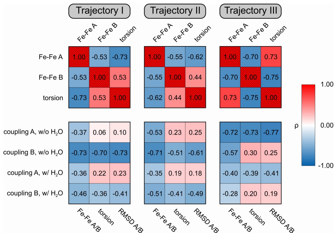
Fig 5 Overview of Spearman rank correlation coefficients \rho calculated for selected molecular properties of Dd 2Fe-SOR as extracted from the three MD trajectories. Entries are colour coded, where saturated red (blue) indicates a perfect positive (negative) correlation. Diagonal entries reflecting trivial self correlations are crossed out. For reasons outlined in the Supplementary Information (SI 3), only the first 25 ns were considered in the calculation of \rho values for trajectory III. All correlations are statistically significant at the 0.01 level. (Top) Correlations between selected internal coordinates (also see Figure SI 1). Fe–Fe A and Fe–Fe B refer to the interdomain Fe–Fe distances within the respective subunits. The interdomain torsion is defined as the dihedral angle Fe1–C1'–C2'–Fe2, where Fe1 and Fe2 refer to the Fe atoms of centres I and II in one subunit, while C1' (C2') specifies the centroid of the two Fe1 (Fe2) atoms. (Bottom) Correlations between Fe1–Fe2 interdomain electronic couplings and selected geometric properties of the same subunit (also see Figures SI 3 – SI 8). RMSD values were calculated with respect to the first trajectory frame. Electronic couplings were determined by the pathways model 86 in the presence (w/ H 2 O) and absence (w/o H 2 O) of water.
