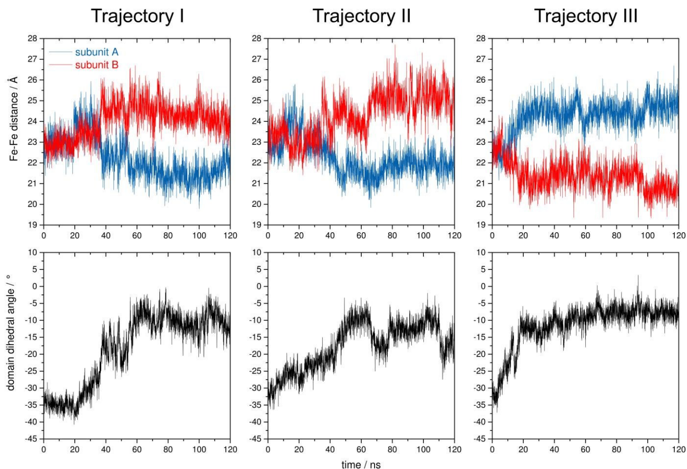
Fig 4 Time evolution of selected internal coordinates of Dd 2Fe-SOR, plotted for all three MD trajectories. (Top) Interdomain Fe–Fe distances for subunits A (blue) and B (red). (Bottom) Domain dihedral angle defined as Fe1–C1′–C2′–Fe2, where Fe1 and Fe2 refer to the Fe atoms of centres I and II in one subunit, while C1′ (C2′) specifies the centroid of the two Fe1 (Fe2) atoms.
