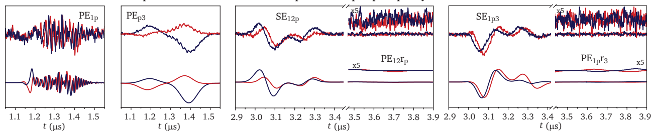
Fig. 5 Experimental (top) and simulated (bottom) two- and three-pulse echoes generated by Gaussian observer pulses, with pulse lengths of 80 ns and 160 ns and FWHM of 32 ns and 64 ns for \pi/2 and \pi pulses, respectively, and a 200 ns sech/tanh pulse ( BW_\infty = 70 MHz, \beta = 4/t_p ) at a coherent pump frequency ( \Delta\nu = +75 MHz). The echoes are labelled as in Table 1. Two-pulse echoes were recorded and simulated with a delay \tau equal to 600 ns, three-pulse echoes with a first delay of 600 ns and a second delay of 1800 ns. The simulations were performed as described in the main text. The time axis, intensity and phase were adjusted individually to match the experiment. The complete set of echoes for Gaussian observer pulses is shown in Fig. S8 in the SI.
