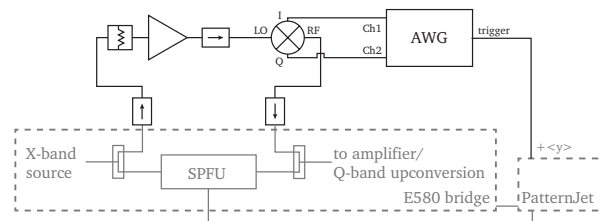
Fig. 10 Schematic block diagram of the homebuilt AWG extension to the Bruker Elecsys X/Q-band spectrometer. The X-band microwave signal from the power splitter before the spectrometer's pulse forming channels is amplified and drives an IQ mixer connected to the two channels of the AWG. The pulses from the AWG are routed back into the bridge through the power combiner after the pulse forming channels.
