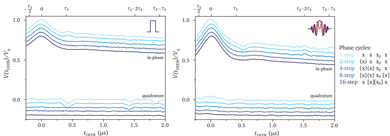
Fig. 6 Four-pulse DEER traces recorded with different phase cycles for a monochromatic rectangular pump pulse (left, t_p = 64 ns, \Delta v = 70 MHz) and a sech/tanh pump pulse (right, t_p = 200 ns, BW_\infty = 70 MHz, \beta = 4/t_p , \Delta v = 75 MHz). Traces recorded with different phase cycles are slightly offset for better comparison. In both cases, the observer pulse lengths were t_{\pi/2} = 32 ns and t_\pi = 64 ns and inter-pulse delays were set to \tau_1 = 400 ns and \tau_2 = 2.3 \mu s. Further experimental details can be found in section 5. Remaining distortions at the end of the trace were found to be due to instrumental effects due to the close proximity of the pump and the last observer pulse.
