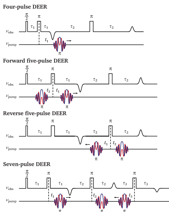
Fig. 1 Schematic representation of the pulse sequences for four-pulse, the forward and reverse versions of five-pulse, and seven-pulse DEER. The time axis of the DEER experiment is obtained as t_{\text{DEER}} = t_1 - \tau_1 for the four-pulse experiment, t_{\text{DEER}} = t_1 - t_2 for the five-pulse DEER experiments and t_{\text{DEER}} = \tau_1 + \tau_2 + \tau_3 - t_1 - t_2 - t_3 for the seven-pulse DEER experiment.
