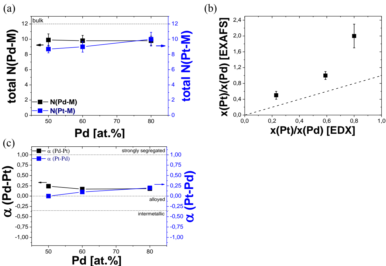
Figure 4. (a) Total coordination numbers ( N_{Pt-M} and N_{Pd-M} ) versus aerogel composition. (b) Chemical compositions obtained from EXAFS and EDX analysis. The dashed lines visualize the ideal mixture of bimetallic system. (c) Short range order parameter ( \alpha_{Pt-Pd} and \alpha_{Pd-Pt} ) in dependence of the content of Pd for the pristine Pd-Pt aerogels. Dashed lines symbolize the possible 3D-architectures of bimetallic systems such as intermetallic fcc motifs for \alpha = -1/3 , randomly disordered alloyed motifs for \alpha = 0 and strongly segregated motifs for \alpha = +1 .
