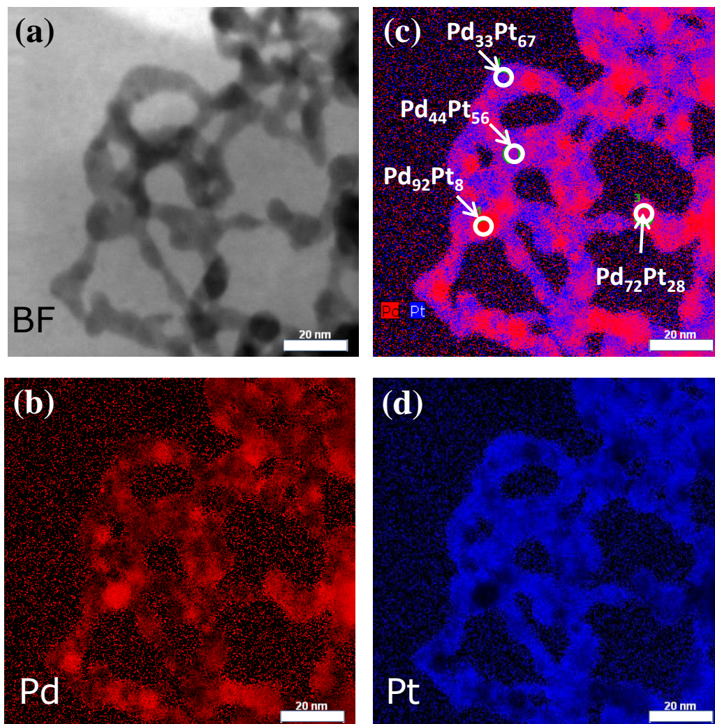
Figure 5. Bright-field STEM micrograph (a) and the corresponding EDX maps for the Pd (b) and Pt (d) measured from this region of the Pd 50 Pt 50 aerogel. (c) Overlap of the EDX maps for each element. The Pd and Pt are denoted with red and blue color, respectively. The scale bar is 20 nm.
