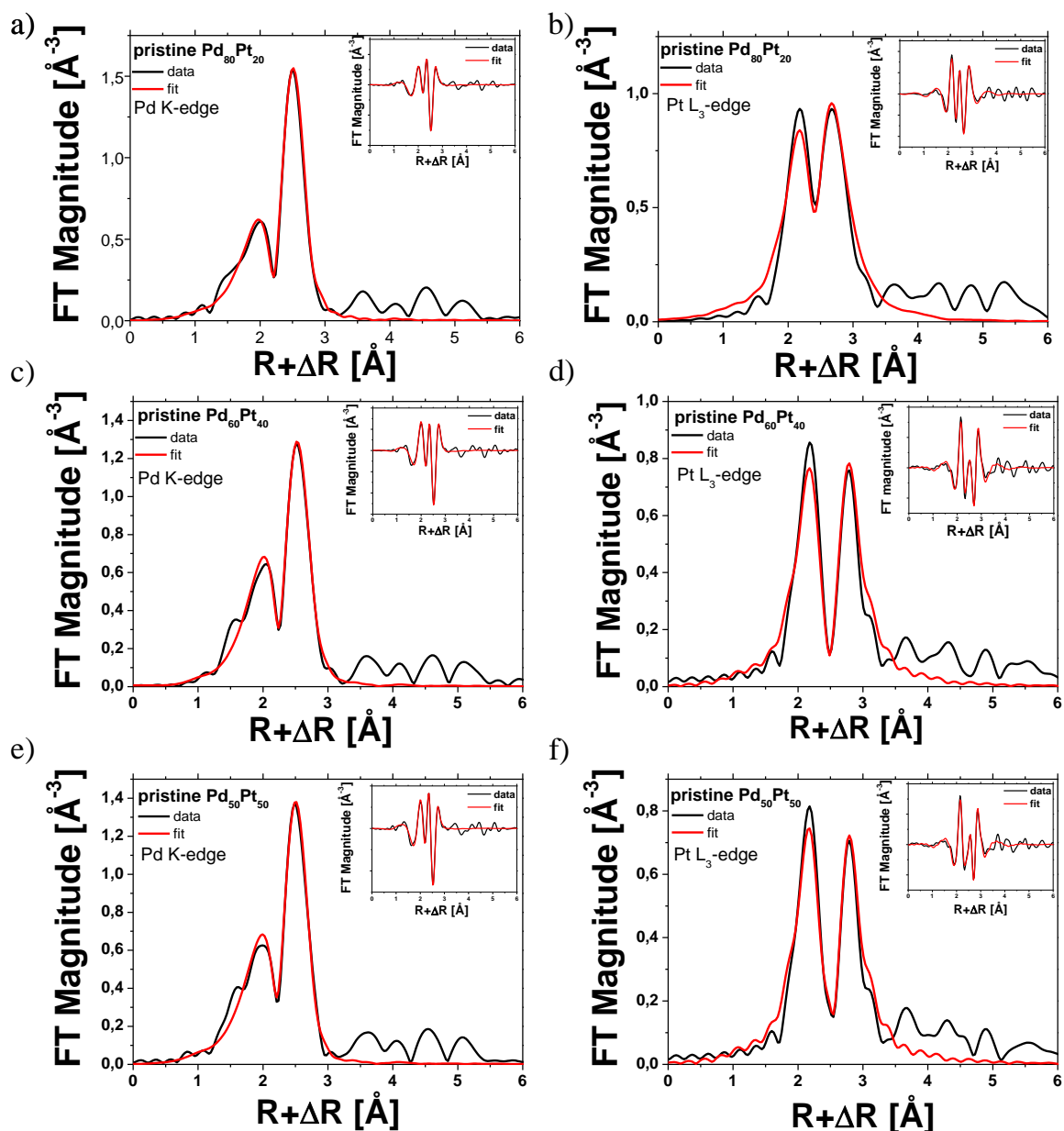
Figure 3. Fourier-transform magnitudes of the k^2 -weighted EXAFS data (black line) and of the corresponding fit (red line) at the Pd K-edge (left side) and Pt L_3 -edge (right side) for the (a, b) Pd_{80}Pt_{20} , (c, d) Pd_{60}Pt_{40} and (e, f) Pd_{50}Pt_{50} aerogels. The inserted plots (b, d and f) show the imaginary part of the k^2 -weighted Fourier transformed EXAFS spectra (black lines) and the corresponding fits (red lines). The k -ranges for the Fourier-transformed spectra at the Pd K-edge and Pt L_3 -edge were from 3 to 15 \text{\AA}^{-1} and from 3 to 14 \text{\AA}^{-1} for Pd K-edge and Pt L_3 -edge, respectively, while the ranges for the fits were from 1.6 to 3.1 \text{\AA} and 1.8 to 3.2 \text{\AA} for Pd K-edge and Pt L_3 -edge, respectively.
