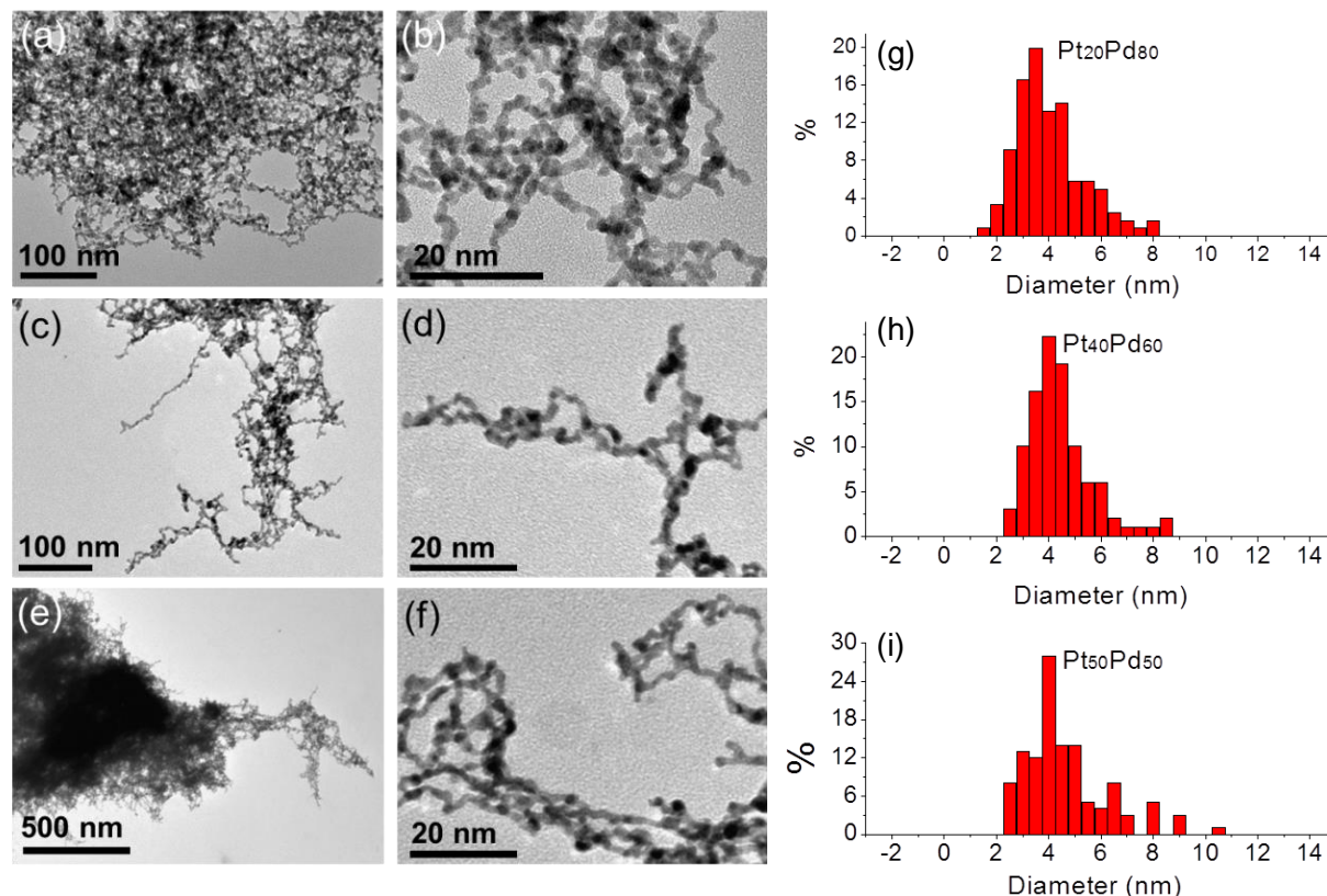
Figure 1. TEM micrographs of the Pd 80 Pt 20 (a, b), Pd 60 Pt 40 (c, d) and Pd 50 Pt 50 (e, f) aerogels at different magnifications. (g, h, i) Diagrams of the nanochain diameter distributions for each Pd-Pt aerogel were established by measuring of more than 100 regions of the nanochain segments. The mean diameters of the nanochains are 4.0 \pm 1.4 nm, 4.3 \pm 1.2 nm and 4.2 \pm 1.2 nm for the Pd 80 Pt 20 , Pd 60 Pt 40 and Pd 50 Pt 50 aerogels, respectively.
