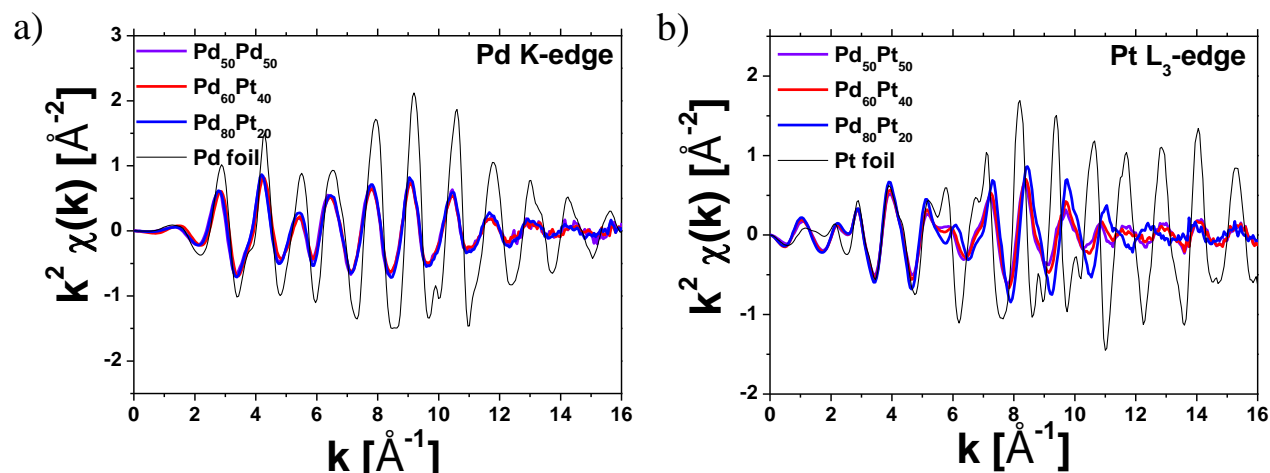
Figure 2. k^2 -weighted EXAFS data of the Pd_{50}Pt_{50} (purple line), Pd_{60}Pt_{40} (red line), Pd_{80}Pt_{20} (blue line) aerogels and of the Pt or Pd foil (thin black line) measured at the (a) Pd K-edge and (b) Pt L_3 -edge, respectively.
