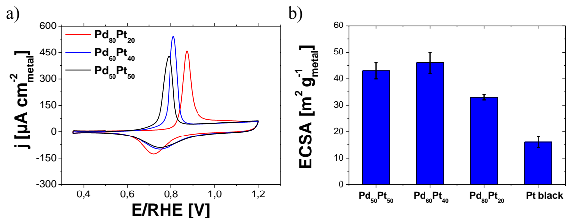
Figure 7. (a) CO stripping cyclic voltammetry (CV) profiles of the \text{Pd}_{80}\text{Pt}_{20} (red line), \text{Pd}_{60}\text{Pt}_{40} (blue line) and \text{Pd}_{50}\text{Pt}_{50} (black line) aerogels. Experimental parameters: scan rate of 50 \text{ mV s}^{-1} , metal loading of 12 - 17 \mu\text{g cm}^{-2}_{(\text{geo.})} in 0.1 \text{ M HClO}_4 at room temperature. (b) Comparison between the values of the electrochemically active surface area (ECSA) for the various Pd-Pt aerogels and commercially available unsupported Pt black catalyst.
