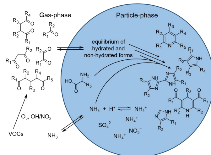
Fig. 8 Schematic overview of secondary BrC and potential photosensitizer formation in the aqueous aerosol phase by (di-)carbonyls and amines, yielding (synergistic) nitrogen heterocyclic compounds.
