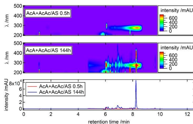
Fig. 4 HPLC-DAD analysis image plot for AcA+AcAc/AS: 0.5 h (top) and 144 h (middle) reaction time; bottom: UV/Vis chromatogram, \lambda = 300 - 500 nm, for AcA+AcAc/AS. The signal at 8.3 min RT accounts for \sim 51 % of the total absorbance in the plotted wavelength range.
