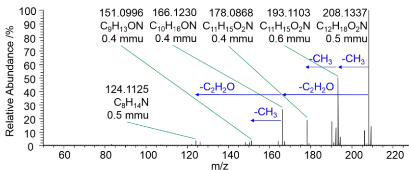
Fig. 6 High-resolution fragment ion mass spectrum (MS 2 ) of a compound with the exact m/z 208.1337 identified to be light-absorbing at \lambda \sim 380 nm in AcA+AcAc/AS system. MS 2 signals are labeled with exact mass, sum formula, and mass deviation (in milli mass units, mmu) to the calculated mass of the respective sum formula. Blue arrows indicate proposed neutral losses.
