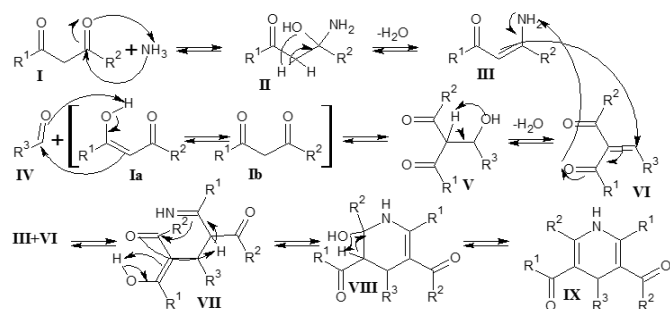
Fig. 7 Mechanism of the Hantzsch 1,4-dihydropyridine synthesis. 55 In the AcA+AcAc/AS system R^1 , R^2 , and R^3 are methyl groups. Product identity was confirmed to be 3,5-diacetyl-2,4,6-trimethyl-1,4-dihydropyridine by reference compound analysis (Fig. S34).
