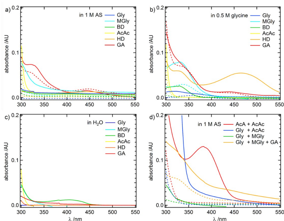
Fig. 3 Zoom in of UV/Vis spectra for the actinic flux wavelength region: 1M dicarbonyls in a) AS (1 M), b) glycine (0.5 M), and c) H 2 O; d) UV/Vis spectra of dicarbonyl mixtures (1M) in AS (1M). All samples were diluted by a factor of 167 before analysis. Dashed colored lines represent spectra recorded after 0.5 h reaction time, solid lines are spectra recorded after 144 h reaction time.
