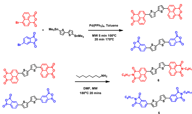
Figure 3 Synthesis of compounds 5 and 6 .
