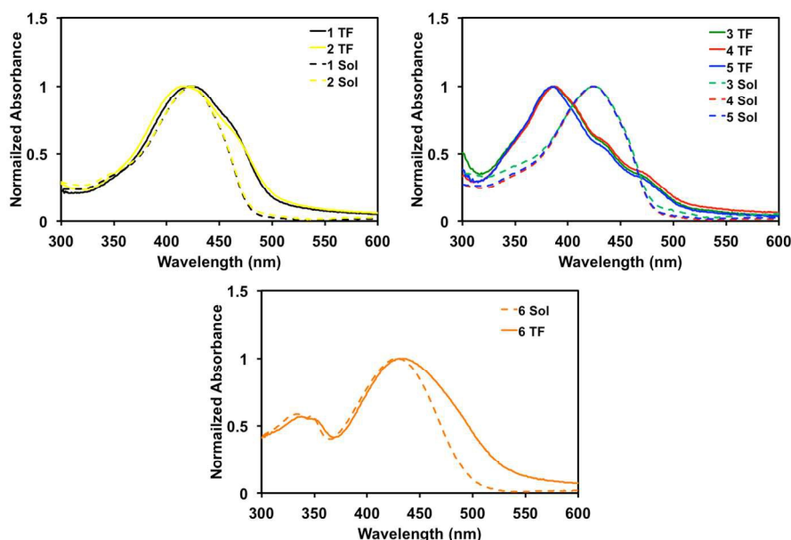
Figure 4 UV-vis absorption of small molecules 1–6 in \text{CHCl}_3 (Sol) or as thin-films (TF) cast from \text{CHCl}_3 . Absorption profiles in solution (dashed lines) and as-cast spin coated films (dark solid lines).
