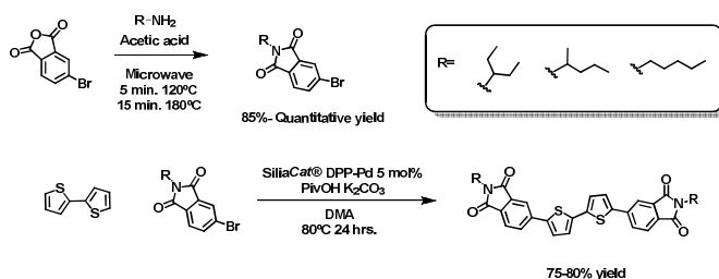
Figure 2 Synthesis of compounds 1-3.
