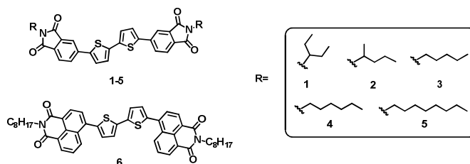
Figure 1 Structures of compounds 1-6. Compound 6 incorporates linear octyl chains.
