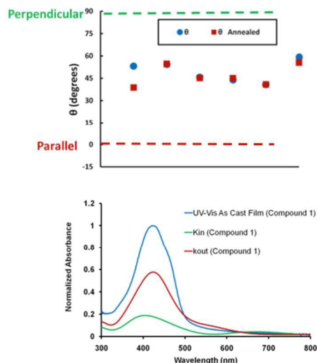
Figure 9. Plot of the orientation angles ( \theta ) found for each film B ) Comparison of pseudo optical coefficients with experimental UV-Vis data, the differences in optical constant values in the in-plane and out of plane directions were used to describe the optical anisotropy in the thin films.
