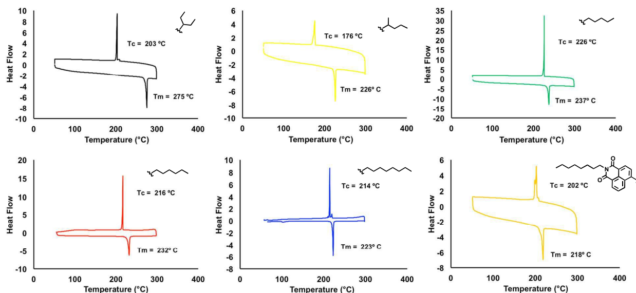
Figure 6 DSC thermograms of compounds 1-6 .
