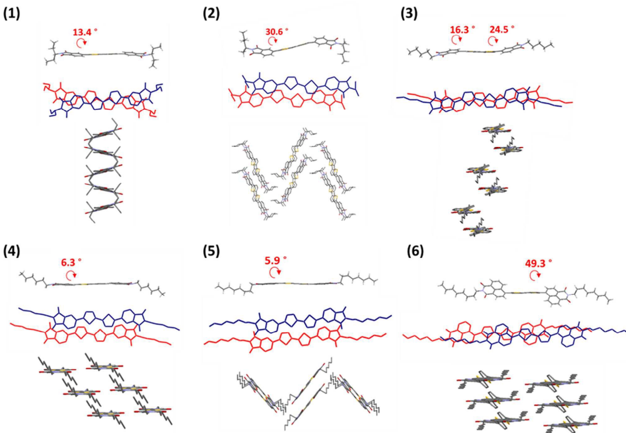
Figure 7: Single crystal structures of 1-6 . Depiction of a single molecular units of 1-6 from crystal structure data, the dihedral angle between the end-capping phthalimide units and the thienyl linkers is given for each molecule ( Top ). Illustration of the extent of molecular overlap between adjacent molecules within the crystal structures ( Middle ). Packing diagrams illustrating the different packing
