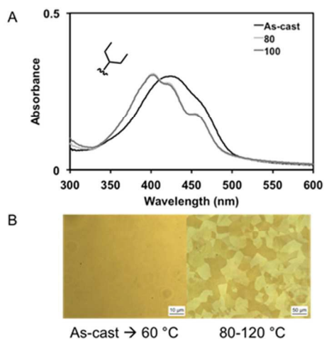
Figure 5 A) Absorption profile of as-cast and thermally annealed films of compound 1 . B) Optical microscopy images of as-cast and annealed films of compound 1 at 100x (left) and 20x (right).
