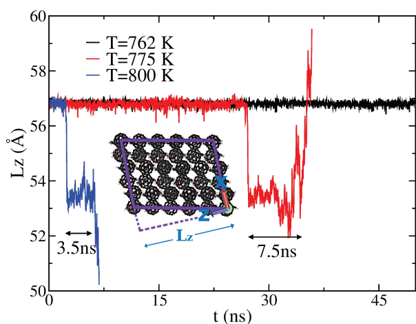
Fig. 1 Variation of L_z versus time at T=762 K (black), T=775 K (red), and T=800 K (blue). The inset shows a snapshot from the simulation at T=700 K, as well as the magnitude and direction of L_z .
