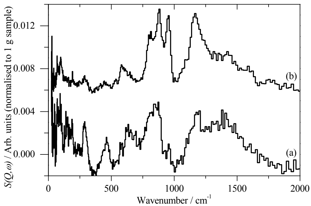
Figure 1. Inelastic neutron scattering spectrum of a. XC72R, b.G-60. a. is \times 2 ordinate expanded relative to b.
