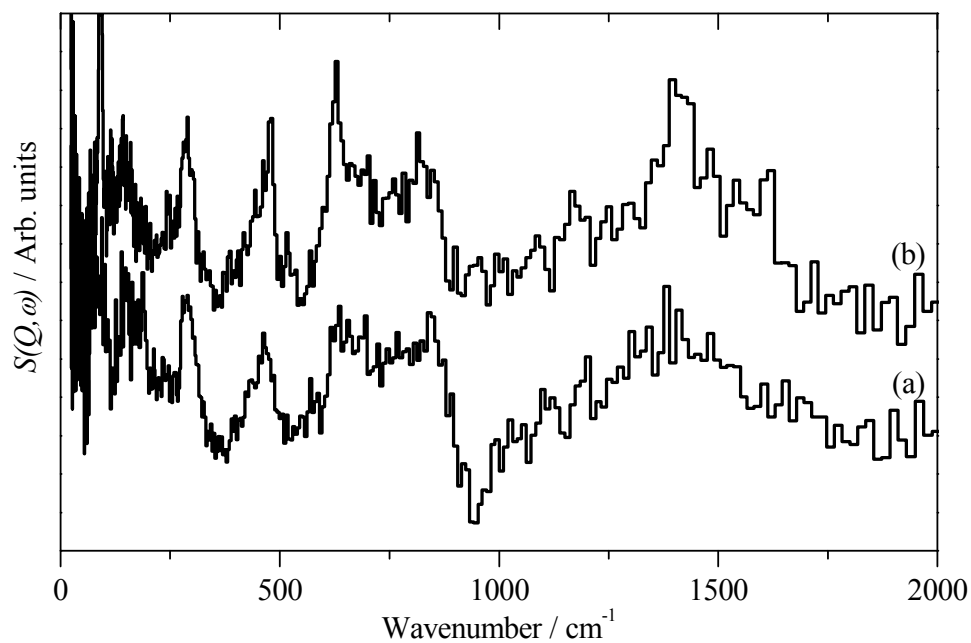
Figure 2. a. Inelastic neutron subtracted spectra of: [XC72R - G-60] to emphasise the non-hydrogen features, b. Graphite
