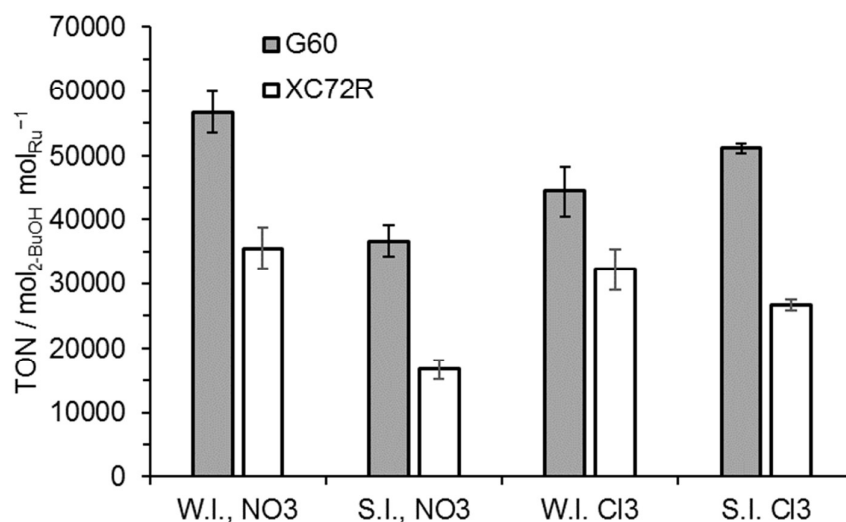
Figure 4. The effect of different carbons, precursors, and preparation methods on Ru/C catalysts for 2-butanone hydrogenation. W.I. = wet impregnation; S.I. = sol immobilisation; NO 3 = Ru(NO)(NO 3 ) 3 precursor; Cl 3 = RuCl 3 precursor. Reaction conditions: 110 °C, 1 bar H 2 , 0.5 h, 5 wt.% 2-butanone in H 2 O, 0.05 g of catalyst.
