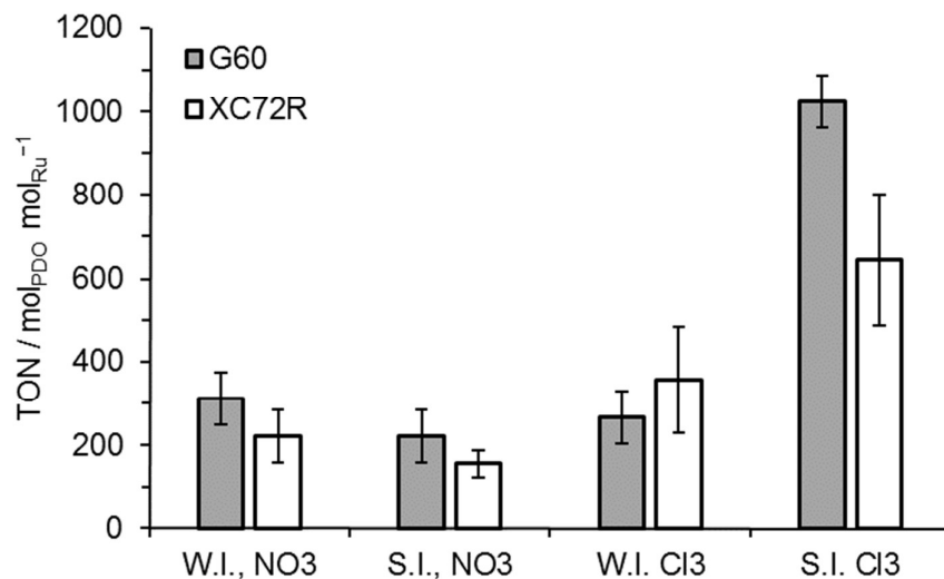
Figure 3. The effect of different carbons, precursors, and preparation methods on Ru/C catalysts for lactic acid hydrogenation. W.I. = wet impregnation; S.I. = sol immobilisation; NO 3 = Ru(NO)(NO 3 ) 3 precursor; Cl 3 = RuCl 3 precursor. Reaction conditions: 125 °C, 35 bar H 2 , 2.5 h, 5 wt.% lactic acid in H 2 O, 0.1 g of catalyst.
