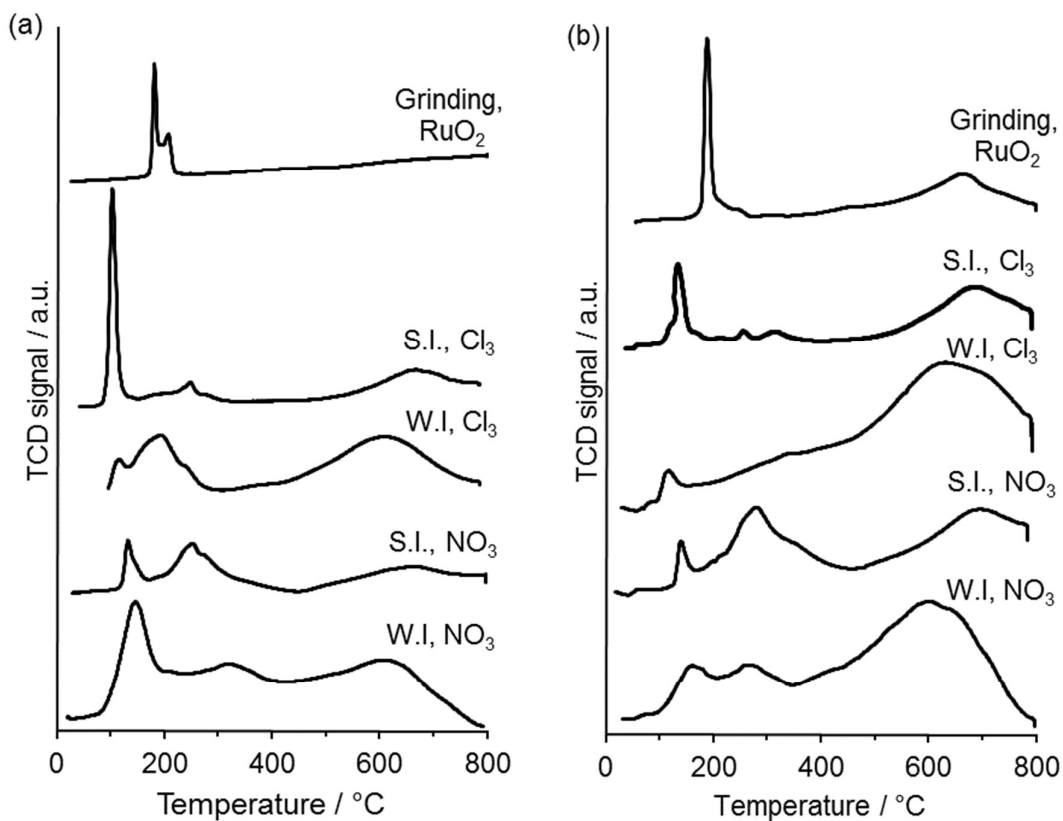
Figure 6. TPR profiles for 1 wt.% Ru/C catalysts prepared using (a) XC72 carbon and (b) G60 carbon. W.I. = wet impregnation; S.I. = sol immobilisation; NO 3 = Ru(NO)(NO 3 ) 3 precursor; Cl 3 = RuCl 3 precursor
