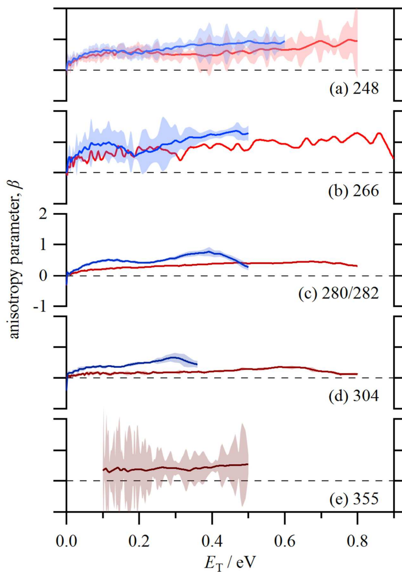
Figure 8. E_T -dependent anisotropy parameters derived from ion images probing I (red) and I* (blue) at the excitation wavelengths (a) 248 nm, (b) 266 nm, (c) 280/282 nm, (d) 304 nm, and (e) 355 nm. 85x120mm (300 x 300 DPI)
