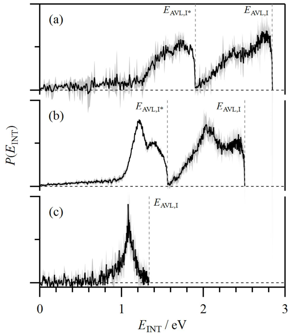
Figure 11. Overall \text{CH}_2\text{I} internal energy distributions, constructed from I and \text{I}^* measurements weighted by respective quantum yields at pump wavelengths of (a) 248 nm, (b) 266 nm, and (c) 355 nm. 82x95mm (300 x 300 DPI)
