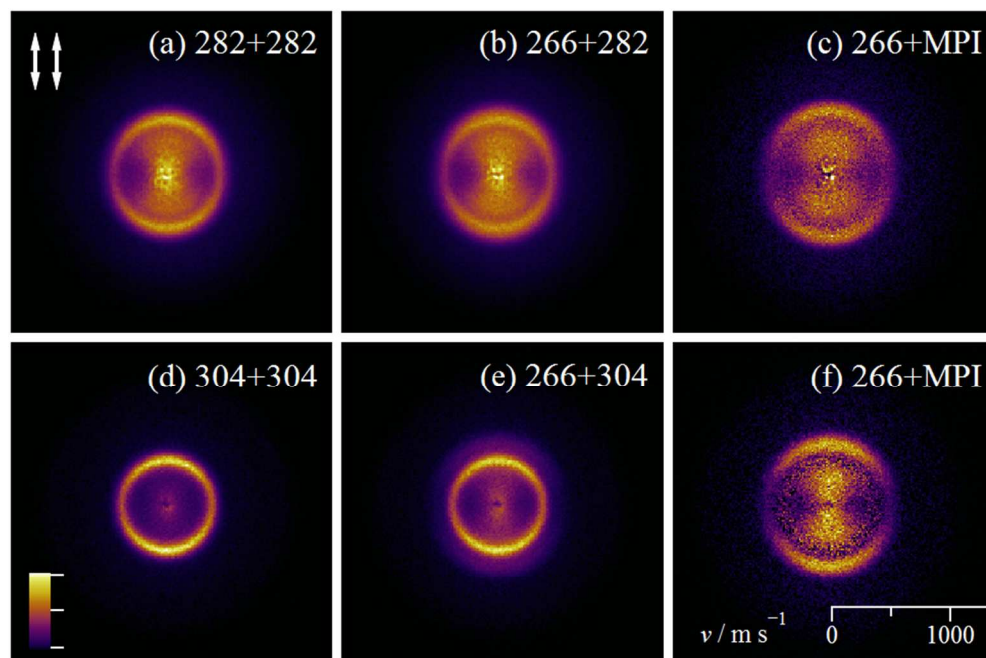
Figure 4. Ion images of I^* products detected with REMPI after the photodissociation of \text{CH}_2\text{I}_2 at \lambda_{\text{pump}} + \lambda_{\text{probe}} (in nm). Top row: (a) 282 + 282, (b) 266 + 282, (c) 266 + MPI difference image obtained from scaled subtraction i.e. (b) - f (a). Bottom row: (d) 304 + 304, (e) 266 + 304, (f) 266 + MPI difference image obtained from scaled subtraction i.e. (e) - f (d)
