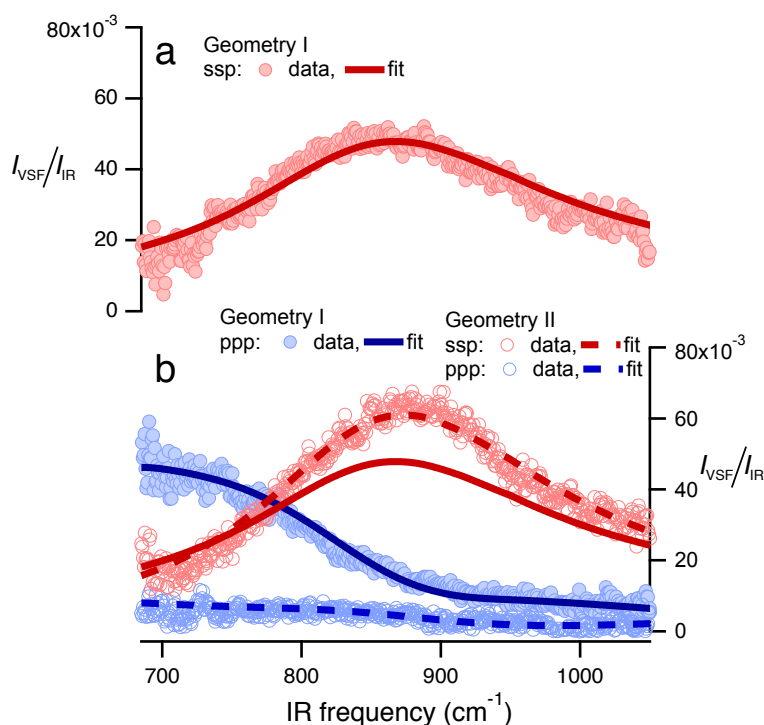
Fig. 2 I_{\text{VSF}}/I_{\text{IR}} plotted as a function of incident IR frequency for spectra collected in (a) geometry I under the ssp polarization condition and (b) in geometry I under the ppp , and geometry II under both ssp and ppp . Solid and dashed lines are fits to the data using the line-shape model described in the text. The fit of the spectra shown in (a) is reproduced in (b) for comparison. All spectra shown have been normalized to account for the frequency-dependent IR intensity and to account for intensity variations between experimental configurations (see section 2 of the Supplementary Information for details).
