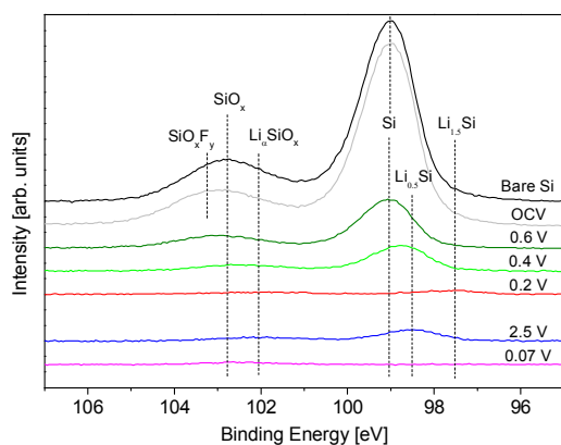
Fig. 6 Ex situ Si 2p XPS spectra used to calculate SEI thickness using Eq. 3. Spectra colored to match that of the closest SLD profile determined from NR.
