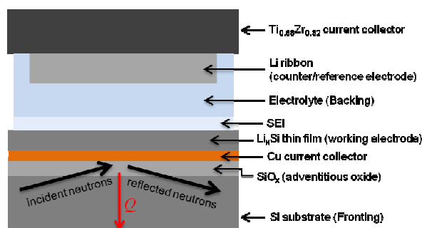
Fig. 1 Experimental geometry for collecting NR data.
