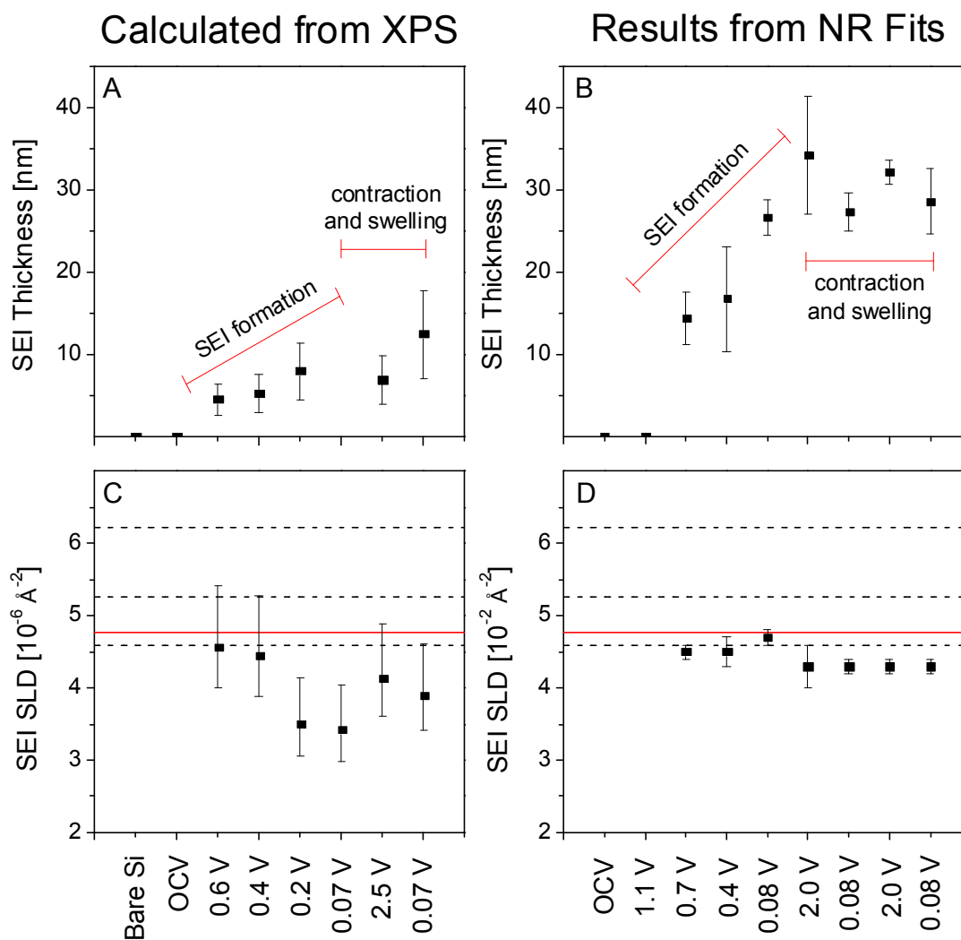
Fig. 8 SEI thickness and SLD as determined via ex situ XPS (A, C) and in situ NR (B, D). The black dashed lines in C and D indicate the expected SLD for lithium perfluoroglutarate (Sect. 3.4) at the atomic density of LiF (upper), \text{Li}_2\text{CO}_3 (middle), and EC (lower). The solid red line indicates the SLD of the electrolyte.
