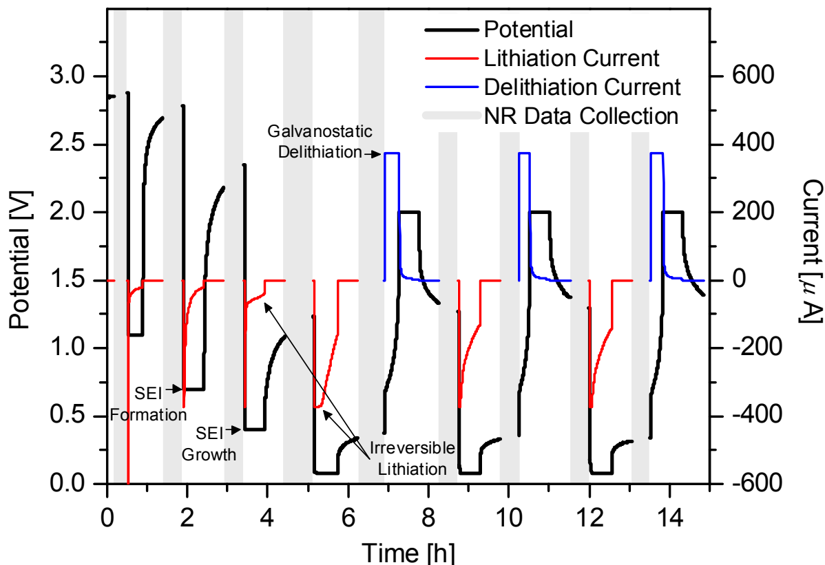
Fig. 3 Electrochemical data for in situ NR cell. NR data was collected during the gaps (grey). The voltage profile is shown in black while the current profile is shown in red (lithiation) and blue (delithiation).
