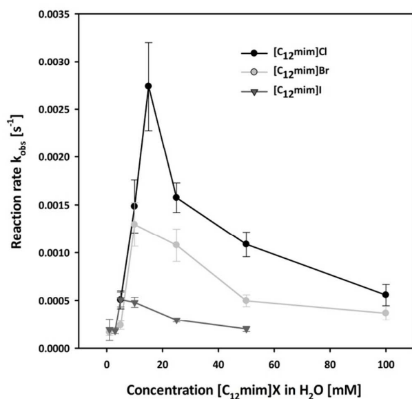
Figure 3. Pseudo first order reaction rate constant of the nucleophilic substitution of nitrophenyl diphenyl phosphate (PNPDPP) with acetaldoxime as a function of [C_{12}mim] with X = Cl, Br and I in water.
