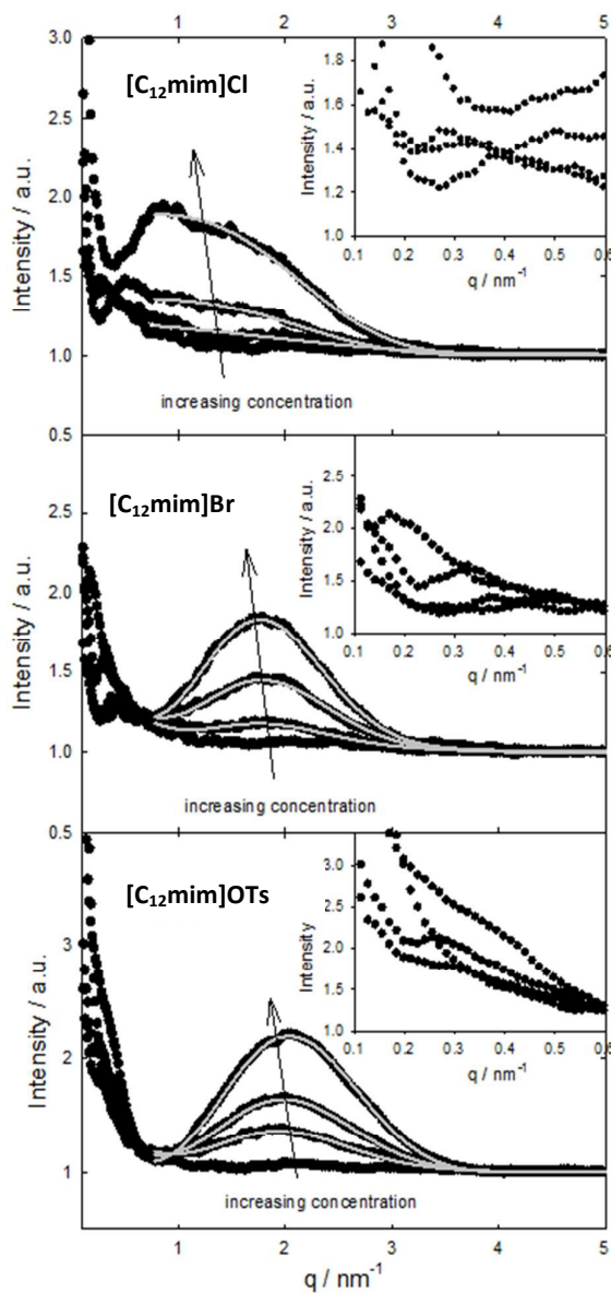
Figure 2. Small-angle X-ray intensities for the different ionic liquids. The experimental intensities are shown as filled circles, the fit from the core-shell model with grey fit lines and the inserts show the scattering intensities towards very low q -values.
