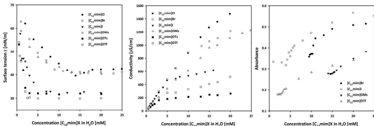
Figure 1. Surface tension (left), conductivity (center) and UV-Vis profiles (right) of the investigated ionic liquids at 25 °C.
