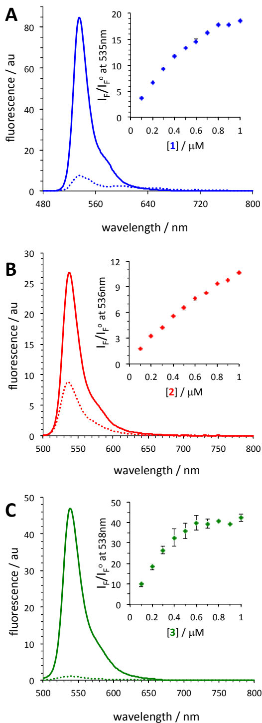
Figure 2. Representative fluorescence spectra of BODIPY dyes (0.5 \mu\text{M} ) 1 (A), 2 (B), and 3 (C) in the presence (solid line) and absence (dotted line) of BSA (39.2 \mu\text{M} ). \lambda_{\text{ex}} = 475 nm. Buffer: 10 mM TRIS (0.1 M NaCl, pH 7.4). Insets: fluorescence enhancement as a function of dye concentration; I_F – fluorescence in the presence of BSA, I_F^0 – fluorescence in the absence of BSA. The data are the average of 2-3 measurements \pm SD.
