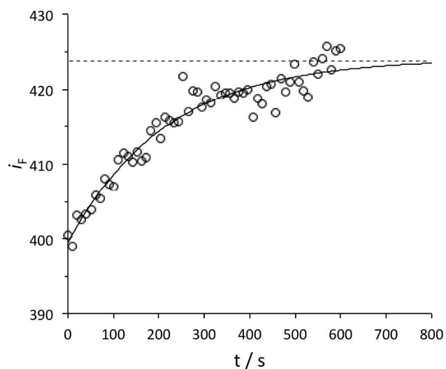
Figure 3. Experimental fluorescence intensity of dye 3 , i_F , as a function of time, t , at C_D = 0.3 \mu\text{M} and C_P = 8.7 \mu\text{M} (open circles); \lambda_{\text{ex}} = 530 nm; \lambda_{\text{em}} = 538 nm; buffer: 10 mM TRIS (0.1 M NaCl, pH 7.4). The solid curve is a fit through the data using I_F(\infty)[1 - \alpha \exp(-bt)] . The dashed horizontal line indicates the obtained value of I_F(\infty) .
