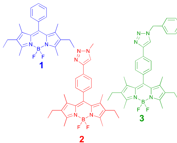
Figure 1. Structures of krypto-BODIPY ( 1 ) and click-BODIPY ( 2 and 3 ) dyes.
