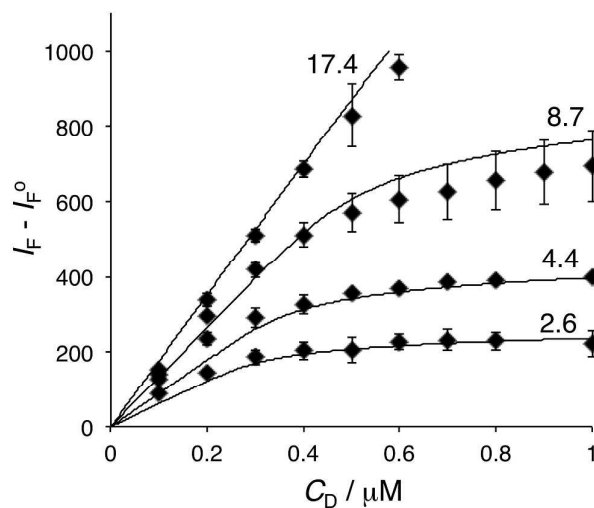
Figure 5. Experimental fluorescence intensity difference, I_F - I_F^0 , as a function of dye concentration, C_D at several protein concentrations, C_p (diamonds; the numbers associated with each curve identify the corresponding experimental values of C_p in \mu\text{M} ). The data are the average of 2-3 measurements \pm SD. The solid curves represent I_F - I_F^0 calculated using Eqs. 6 and 7 with K = 0.12 \mu\text{M}^{-1} , n = 10 , S_D = 0.40 \mu\text{M} , and proportionality constant, k = 2600 \mu\text{M}^{-1} . Conditions: \lambda_{\text{ex}} = 530 \text{ nm} , \lambda_{\text{em}} = 538 \text{ nm} ; buffer: 10 mM TRIS (0.1 M NaCl, pH 7.4).
