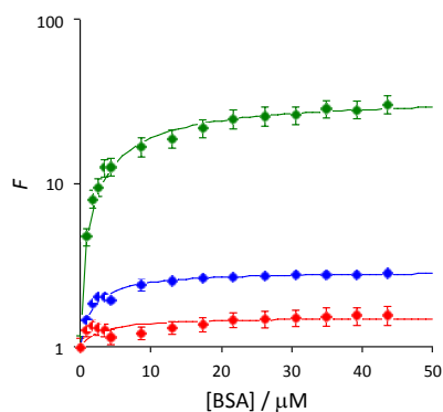
Figure 4. Experimental fluorescence ratios ( F = I_F/I_F^0 ) as a function of protein concentration, C_p , at constant dye concentration, C_D = 0.20 \mu\text{M} , for dyes 1 (blue), 2 (red), and 3 (green); \lambda_{\text{ex}} = 530 \text{ nm} ; \lambda_{\text{em}} = 538 \text{ nm} ; buffer: 10 mM TRIS (0.1 M NaCl, pH 7.4); the data are the average of 2-3 measurements \pm SD. The solid curves are the theoretical fits through the experimental data, obtained using Eqs. 4 and 5.
