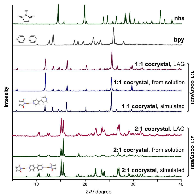
Figure 2. Comparison of reactants, mechanochemical products, crystallization products and calculated powder patterns.
