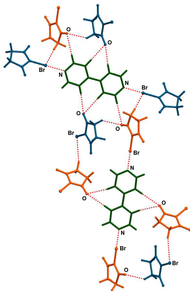
Figure 4. Network of halogen and hydrogen bonded molecules in the crystal structure of (\text{nbs})_2(\text{bpy}) .
