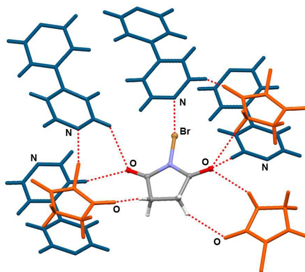
Figure 3. Halogen and hydrogen bonding of nbs molecule with neighbouring molecules in the crystal structure of ( nbs )( bpy ).
