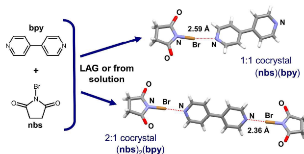
Figure 1. Structures of reactants, N -bromosuccinimide ( nbs ) and 4,4'-bipyridine ( bpy ), and cocrystal structures obtained as a result of the single crystal X-ray diffraction experiment.
