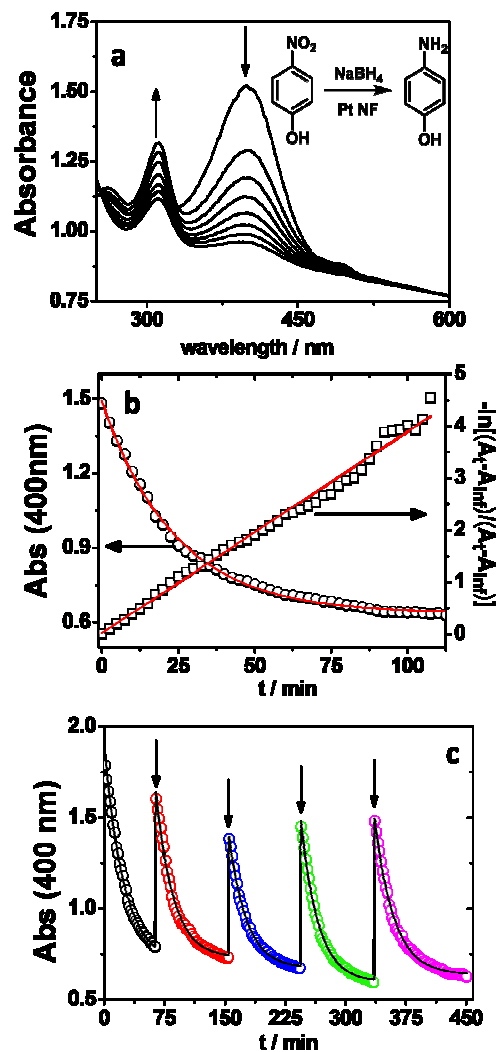
Fig. 3 a) Spectral evolution of a mixture of 4-NP and Pt nanoflowers upon borohydride addition. [4-NP] = 0.05 mM, 0.1 mg Pt NF and [NaBH 4 ] = 0.030 M, T = 25 °C. b) Kinetic trace of the absorbance at 400 nm during the reduction of 4-NP, and linearized data for first-order analysis corresponding to Fig. 3a. c) Absorbance kinetic traces at 400 nm, registered during the sequential reduction of 4-NP. The arrows indicate the times at which 4-NP was added to obtain [4-NP] = 0.05 mM. The line represents the best fit to a first-order rate equation.
