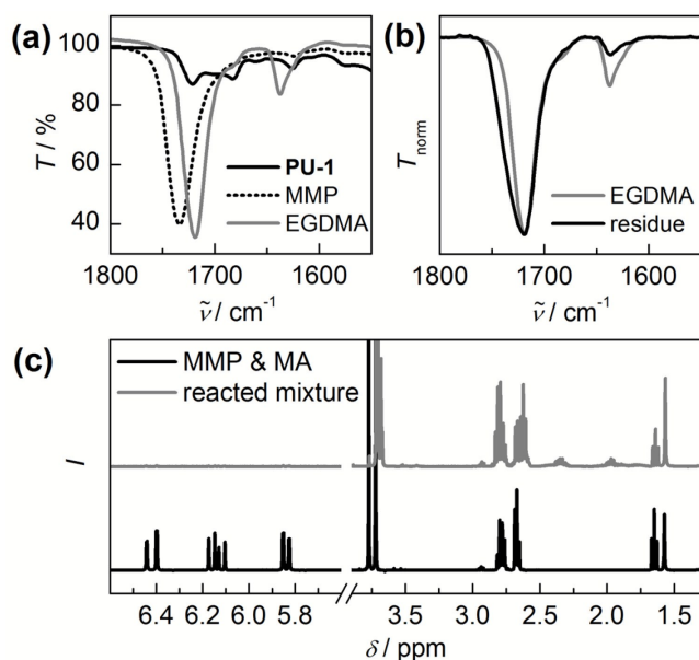
Fig. 3 FTIR transmission spectra of (a) PU-1, PU-1 swollen with MMP and PU-1 swollen with EGDMA as well as (b) PU-1 swollen in EGDMA and the insoluble residue obtained after mechanically induced polymerization normalized to the C=O stretch signal at 1719\text{ cm}^{-1} . (c) ^1\text{H-NMR} spectra of a mixture of MA with 50 mol% MMP before and after subjecting it to the mechanically induced oligomerization by freezing swollen PU-1.
