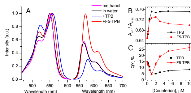
Fig. 2. (A) Absorption (normalized) and fluorescence spectra of 1 \mu\text{M} solutions of Cy3A in methanol and water in the presence of TPB or F5-TPB (10 mol. eq.). Emission spectra were normalized to the same absorbance at 520 nm. \lambda_{ex} = 520 \text{ nm} . (B) The ratio of the absorption bands A_{sh}/A_{max} and (C) the fluorescence quantum yield of 1 \mu\text{M} Cy3A in water vs. counterion concentration.
