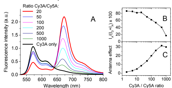
Figure 4. Fluorescence spectra showing FRET from Cy3A to Cy5A co-assembled with F5-TPB (10 mol. eq.) at different donor/acceptor ratios (A). The relative FRET efficiency (B) and antenna effect (C) as a function of donor/acceptor ratio. Concentrations of Cy3A was systematically 1 \mu M. \lambda_{ex} = 520 nm.
