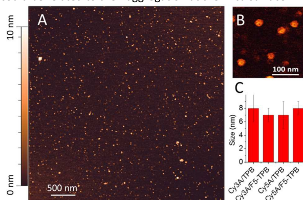
Figure 3. Atomic force microscopy of NPs formed by Cy3A and F5-TPB (10 mol. eq.) (A), a zoomed image (B) and particle sizes measured by AFM (height) for different samples (C).
