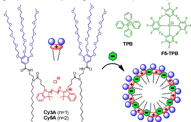
Figure 1. Cyanine amphiphiles and their expected assembly into micelles in the presence of non-coordinating anions.
