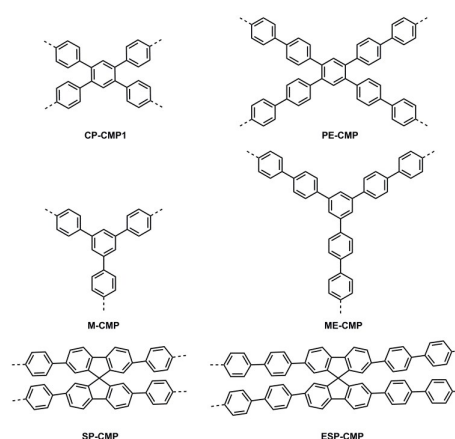
Figure 1 Structures of the conjugated microporous polymers. 32
