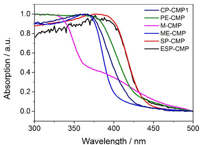
Figure 2 UV/Vis reflectance spectra of the CMPs in the solid-state.
