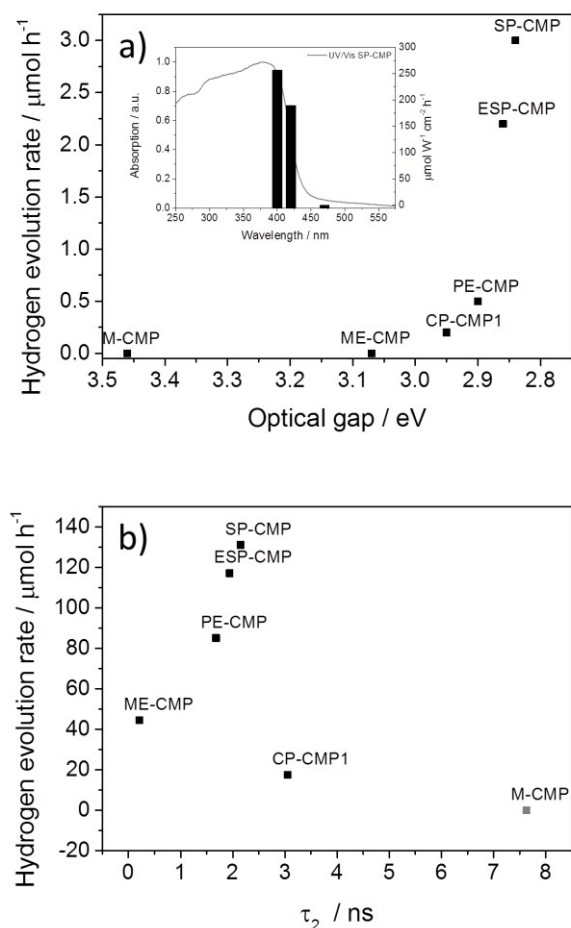
Figure 3 a) Hydrogen evolution rates under visible light ( \lambda > 420 nm) correlated with the optical gap of the CMPs. Each measurement was performed with 25 mg catalyst in water/MeOH/triethylamine mixture. Wavelength dependency of the photocatalytic hydrogen evolution for SP-CMP (insert). b) Correlation of the life-time of the excited state with hydrogen evolution rates under broadband illumination ( \lambda > 295 nm).
