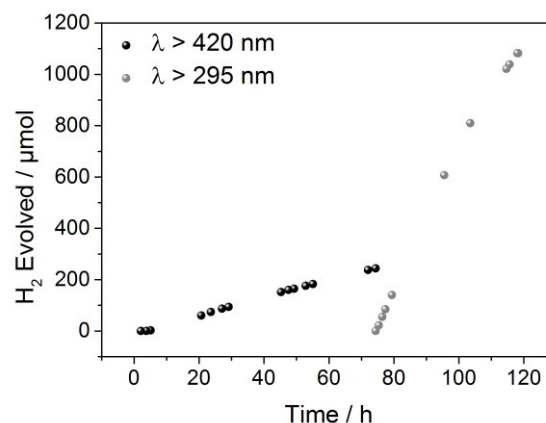
Figure 4 Hydrogen experiment of SP-CMP under visible light ( \lambda > 420 nm) for 74 hours followed by a further 44 hours under combined UV and visible light ( \lambda > 295 nm). The experiment was performed with 25 mg catalyst in water/MeOH/triethylamine mixture.
