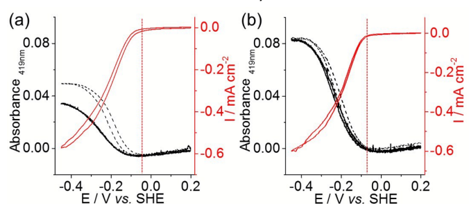
Figure 3. Voltabsorptometry (at 419 nm; black; left axis) and PFV (red; right axis) of (a) mesoITO|FccA and (b) mesoITO|MtrC|FccA electrode in absence (dash black trace) and presence (full black trace and red trace) of 10 mM of fumarate at pH 7 ( \nu = 10 \text{ mV s}^{-1} ) in a pH 7 electrolyte solution. PFV gives a similar catalytic response for mesoITO and IOmesoITO (see Fig. 2).
