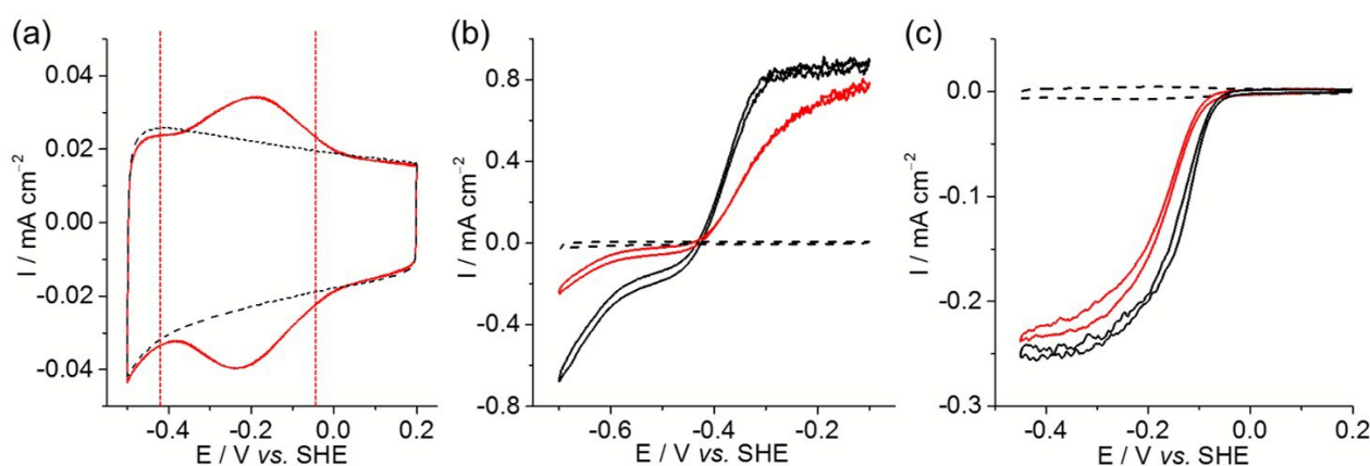
Figure 2. PFV of (a) protein-free IOmesolITO (dashed trace) and IOmesolITO|MtrC, (b) protein-free IOmesolITO (dashed trace), IOmesolITO| H_2 ase (black trace) and IOmesolITO|MtrC| H_2 ase (red trace) under 1 bar 100% H_2 and (c) IOmesolITO|MtrC|FccA in absence of fumarate (dash trace), IOmesolITO|FccA (black trace) and IOmesolITO|MtrC|FccA (red trace) in the presence of 1 mM of fumarate. General conditions: a 2 \mu m thick IOmesolITO electrode in a mixed buffer electrolyte solution at pH 7 and under stirring at a scan rate ( v ) of 10 \text{mV s}^{-1} was employed.
