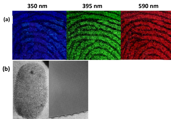
Fig. 3 (a) Fluorescent microscopy images of a fingerprint developed with the C-SiO 2 nanopowder. (b), Comparison between the C-SiO 2 and a commercial fingerprint powder on a fluorescent background investigated on a crime lite imager (445 nm laser with a 455 nm filter).
