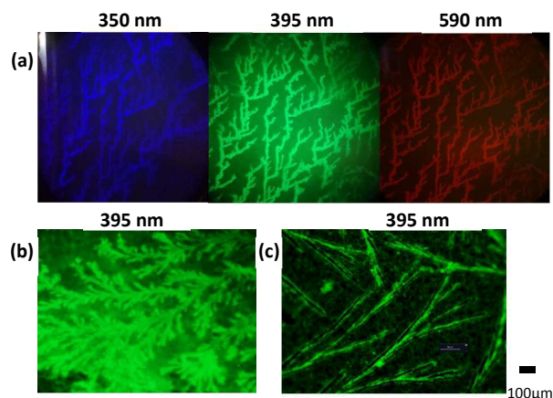
Fig. 4 Fluorescent microscopy images of the nanotags; (a) deposited in glass and illuminated under different excitation wavelengths, (b) deposited in glass from a more concentrated suspension, (c) deposited on a polymeric surface.
