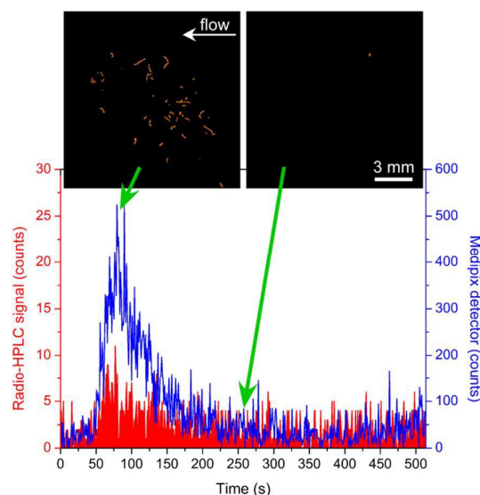
Fig. 3 Plot of ^{68}\text{Ga} -citrate radioactive emissions as it passed through the monolithic column. The blue signal shows the signal from the positron detector below the monolith, while the red signal was taken from a flow-through NaI/PMT radio-HPLC detector. Note that the plots are on different scales. Inset are images (14 x 14 \text{mm}^2 ) taken from the detector at different time points.
