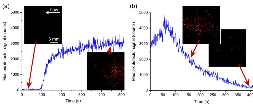
Fig. 4 Trap and release of 68 Ga 3+ on the silica-based monolith, with the positron detector showing the activity in real-time. (a) Trapping in phosphate solution (0.4 M). (b) Release in citric acid (0.1 M). The flow of solution was right-to-left in the images.
