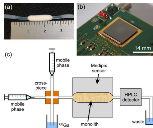
Fig. 1 (a) Silica-based monolithic column encased in heat-shrink tubing. (b) Medipix positron detector, featuring a 14 x 14 mm 2 sensor area. (c) Schematic of the experimental setup, with the monolith placed above the Medipix sensor, and featuring a cross-injection system and a standard sodium iodide radio-HPLC detector.
