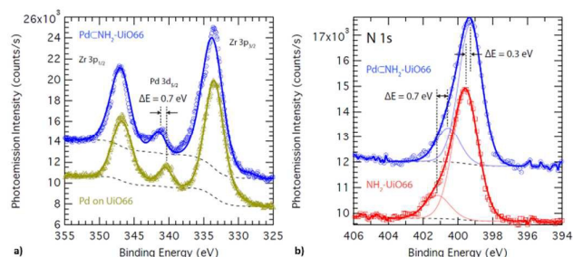
Figure 2 XPS spectrum of a) Pd supported on UiO-66 (mustard) and embedded in \text{NH}_2 -UiO-66 (blue), and b) of N in the bare (red) and Pd-supporting (blue) \text{NH}_2 -UiO-66
