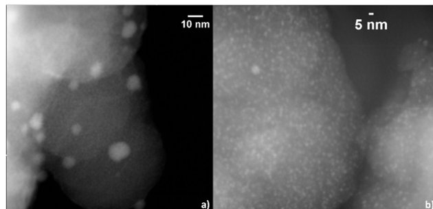
Figure 3 HAADF-STEM micrographs of a) Pd nanoparticles on UiO-66 and b) Pd nanoclusters embedded in \text{NH}_2 -UiO-66
