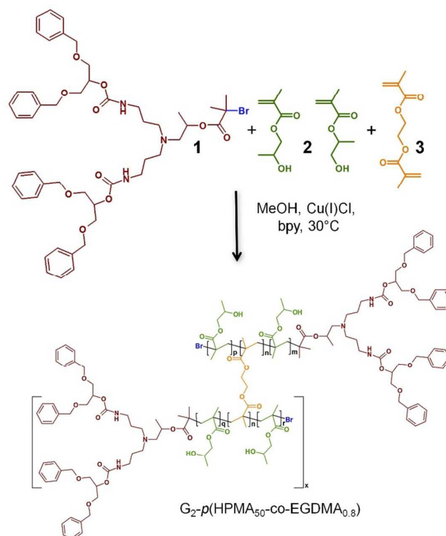
Scheme 1: Cu-catalysed ATRP synthesis of hyp-polydendrons using HPMA, 2 (both isomers shown), EGDMA, 3 , and a G_2 dendritic initiator, 1 .
