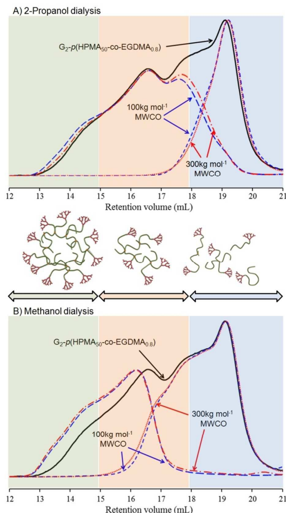
Figure 1: SEC (DMF/0.01 M LiBr eluent) refractive index chromatograms of hyperbranched polydendron samples before (solid black line) and after (red and blue dashed lines) dialysis using either A) 2-propanol or B) methanol as the dialysis solvent. Tubing with two different molecular weight cutoffs (MWCO) were utilized in each solvent condition.
