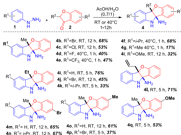
Scheme 4 Scope of the Fischer indolization for the synthesis of benzofuro[3,2- b ]indoline amines from benzofuran-3-ones.
