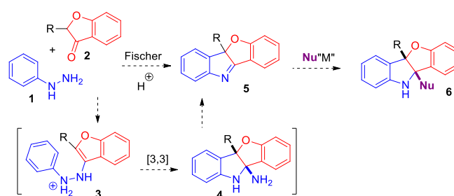
Scheme 2 Planned Fischer indolization strategy towards disubstituted benzofuro[3,2- b ]indolines.
