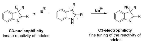
Scheme 1. C3-nucleophilicity and electrophilicity of indoles.
