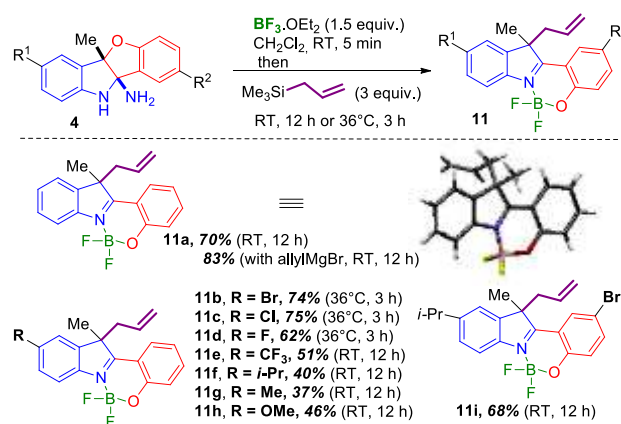
Scheme 5 Addition of allyl nucleophiles to the Fischer indolization products.
