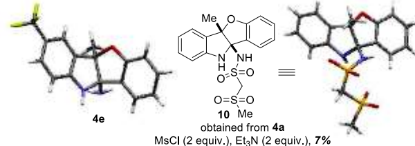
Figure 2 X-Ray structures of benzofuro[3,2- b ]indoline amines 4e and 10 .
