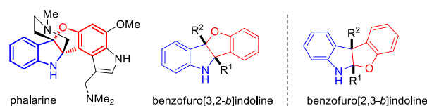
Figure 1 Benzofuroindoline motifs.
