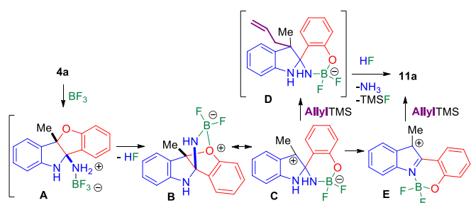
Scheme 6 Postulated activation of the benzofuro[3,2- b ]indoline amines.
