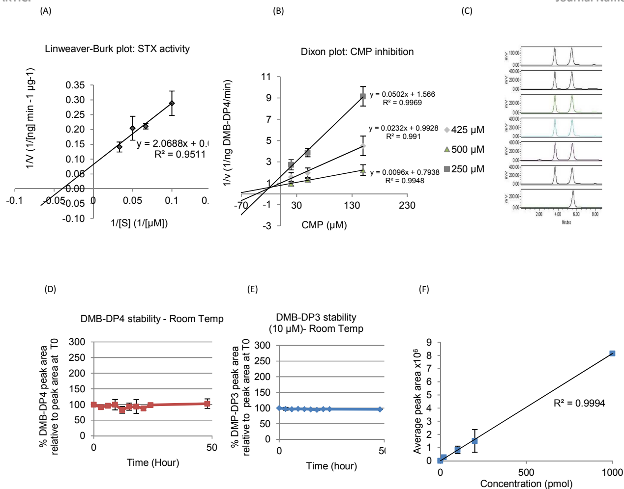
Figure 5. Analysis of assay kinetics and optimisation of the chromatography to allow high throughput-HPLC analysis. Lineweaver-Burk plot (A) and Dixon plot (B). K_m of DMB-DP3 for ST8SialI (derived from x axis intercept, Lineweaver-Burk plot) was calculated as 29.5 \pm 3.0 \mu\text{M} and V_{max} value (calculated from y axis intercept) was calculated as 14.8 \pm 2.7 \mu\text{mol}/\text{min}/\text{mg} . The K_i value of CMP was calculated from the Dixon plot. Graph lines converge above the x axis; where they intersect is -K_i . Data points are from a single determination representative of three independent experiments. (C) The reproducibility of the results when running 6 samples of standard DMB-DP3 and DMB-DP4 consecutively. The first peak at 3.9 minutes represents DMB-DP4 while the second peak at 5.9 minutes represents DMB-DP3, the last chromatogram shows DMB-DP3 only. (D) Stability of DMB-DP4 and (E) DMB-DP3. The experiment was carried out by incubating DMB-DP3 and DMB-DP4 at room temperature for 48 hours. 10 \mu\text{l} of the sample at T0 was analysed using HPLC, then similar volumes of sample were analysed at regular intervals over 24h, then again at 48h. Peak area was measured and percent peak area compared to T0 was calculated and plotted. The experiment was repeated three times and the standard deviation was determined. (F) Limit of detectability of DMB-DP4 standard.
