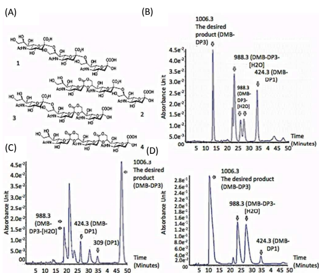
Figure 2. DP3 lactonised forms and different methods used for the purification of DMB-DP3. (A) Structure of non-lactonised alpha-2,8-linked sialic acid trimer 1 , 1-monolactone trimer 2 , 2-monolactone trimer 3 , and di-lactone trimer 4 ; (B) System 1, mobile phase A: 1% methanol, 0.01% formic acid (pH 3.5) and mobile phase B: 55% methanol, 0.01% formic acid (pH 5.8); (C) System 2, mobile phase A: Ammonium formate buffer (pH 6) and mobile phase B: 55% methanol, 0.01% formic acid (pH 5.8); (D) System 3, mobile phase A: ammonium formate buffer (pH 6) and mobile phase B: 55% methanol (pH 7.2).
