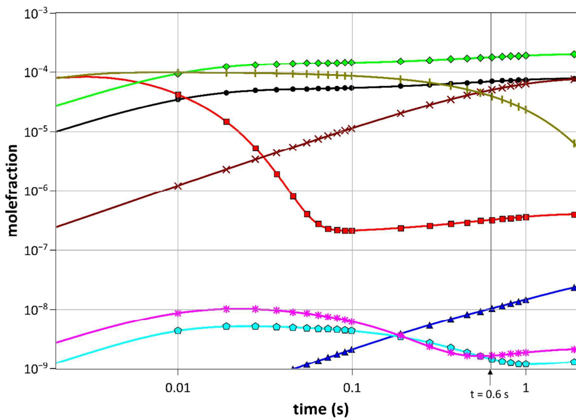
Fig. 2 Calculated molefractions of the most abundant species in the gas phase. ( \text{H}_2 , \text{N}_2 , and \text{NH}_3 are omitted.) Process conditions: T = 1050^\circ\text{C} , \text{NH}_3/\text{TMGa} = 625 . H (●), \text{CH}_3 (■), \text{CH}_4 (◆), \text{C}_2\text{H}_2 (▲), \text{C}_2\text{H}_4 (△), \text{C}_2\text{H}_6 (*), Ga (×), \text{GaCH}_3 (|).
