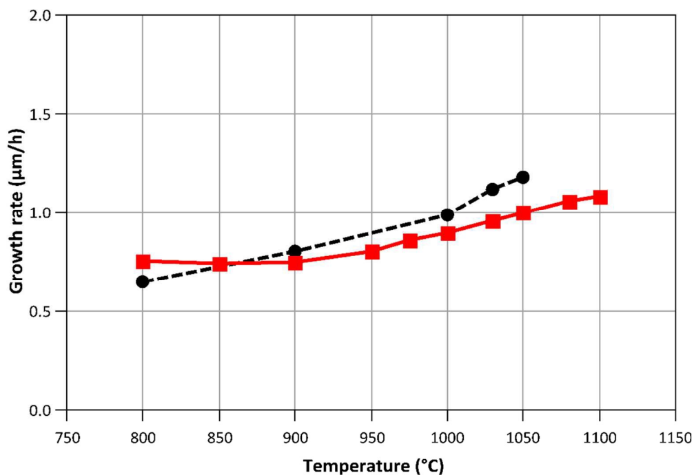
Fig. 5 Calculated (—■—) and measured (---●---) growth rates when varying process temperature. NH 3 /TMGa ratio = 625.
