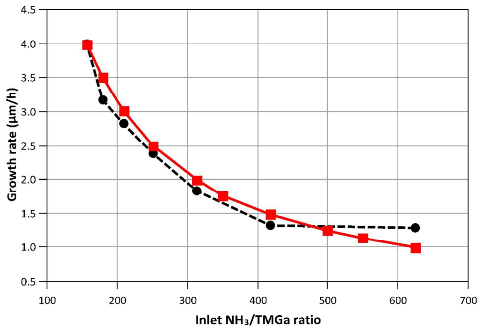
Fig. 4 Calculated (—■—) and measured (---●---) growth rates when varying inlet NH 3 /TMGa ratio at constant NH 3 flow (2000 sccm). Process temperature is 1050°C.
