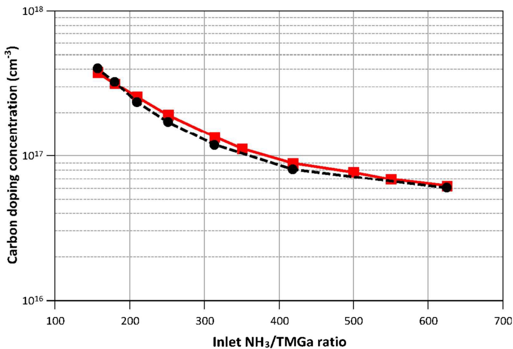
Fig. 6 Calculated (—■—) and measured (---●---) carbon doping concentrations when varying NH 3 /TMGa ratio at constant NH 3 flow (2000 sccm) and T = 1050°C.
