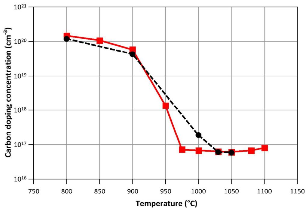
Fig. 7 Calculated (—■—) and measured (---●---) carbon doping concentrations when varying process temperature. NH 3 /TMGa ratio = 625.
