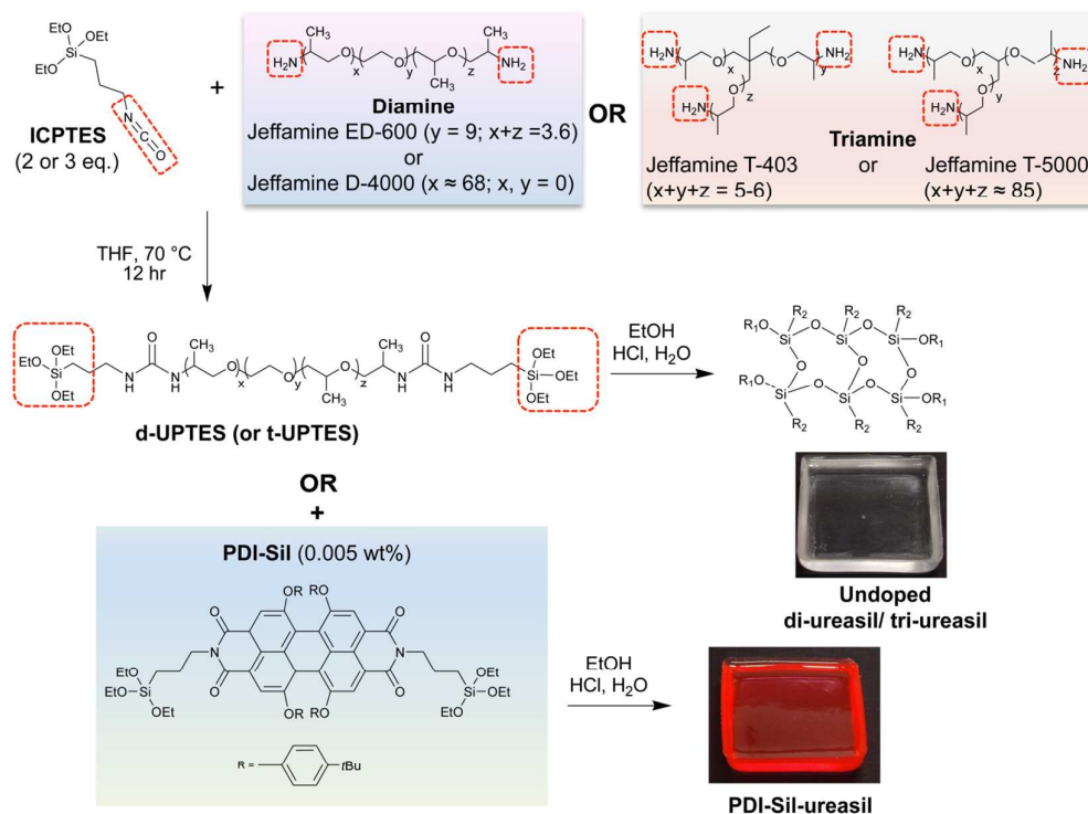
Figure 1. Targeted synthesis of undoped and PDI-Sil-ureasil ( R_1 = \text{Si-O-Si-} or \text{H} , R_2 = \text{-(CH}_2\text{)}_3\text{-NHCONH-Jeffamine} ).
