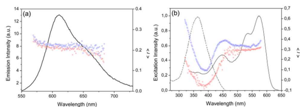
Figure 6. Steady-state anisotropy of the fluorescence (a) emission ( \lambda_{ex} = 500 nm) and (b) excitation ( \lambda_{em} = 630 nm) of PDI-Sil-d-U(600) (red open squares) and PDI-Sil-d-U(4000) (blue open circles). The emission and excitation spectra (black lines) obtained using non-polarised light are shown for comparison.
