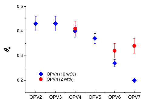
Fig. 6 Coefficient for vertical orientation ( \theta_v ) for transition dipole moments in TPBi/OPV n host/guest layers obtained by fitting the experimental angular p -polarised fluorescence intensity to simulated profiles for partial horizontal ( \theta_h ) and vertical ( \theta_v ) orientation.
