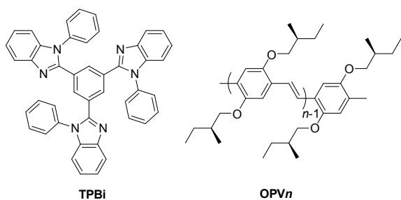
Fig. 1 Chemical structure of host and guest molecules used in this work. (a) Host: TPBi. (b) Guest: OPV n with n the number of phenyl rings ranging from 2 to 7.
