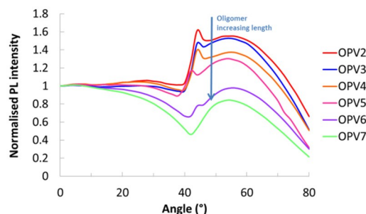
Fig. 4 Angular dependence of the p -polarised fluorescence of solution processed TPBi/OPV n (10 wt.%) layers. The fraction of horizontal dipoles increases with increasing the length of the OPV n molecule. Layers containing OPV6 and OPV7 show preferential horizontal transition dipole moment orientation.
