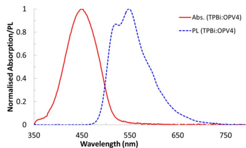
Fig. 3 Absorption (solid line) and fluorescence (dashed line) spectra for a TPBi/OPV4 (10 wt.%) layer.
