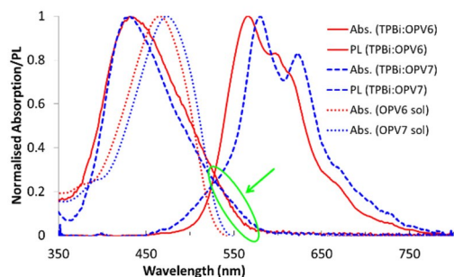
Fig. 7 Absorption and fluorescence spectra for TPBi/OPV6 10% (solid lines) and TPBi/OPV7 (10 wt.%) (dashed lines) and of OPV6 and OPV7 in solution (dotted lines). The tail at high wavelengths in the absorption spectra for both the blends (circled area), indicates aggregation of the films.
