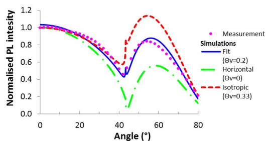
Fig. 5 Experimental angular dependence of the p -polarised fluorescence intensity for a solution processed TPBi/OPV7 (10 wt.%) layer (solid circles) compared to simulated profiles with a different anisotropy factors (solid line for \theta_v = 0.2 ; dashed-dotted line for fully horizontal orientation, \theta_v = 0 ; dashed line for isotropic orientation, \theta_v = 0.33 ).
