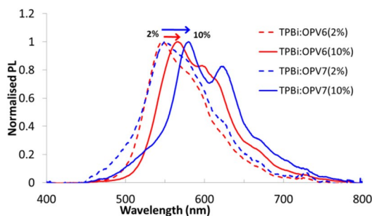
Fig. 8 Normalized fluorescence spectra for TPBi/OPV6 and TPBi/OPV7 host guest films with low loading (2 wt.%, dashed lines) and high loading (10 wt.%, solid lines).
