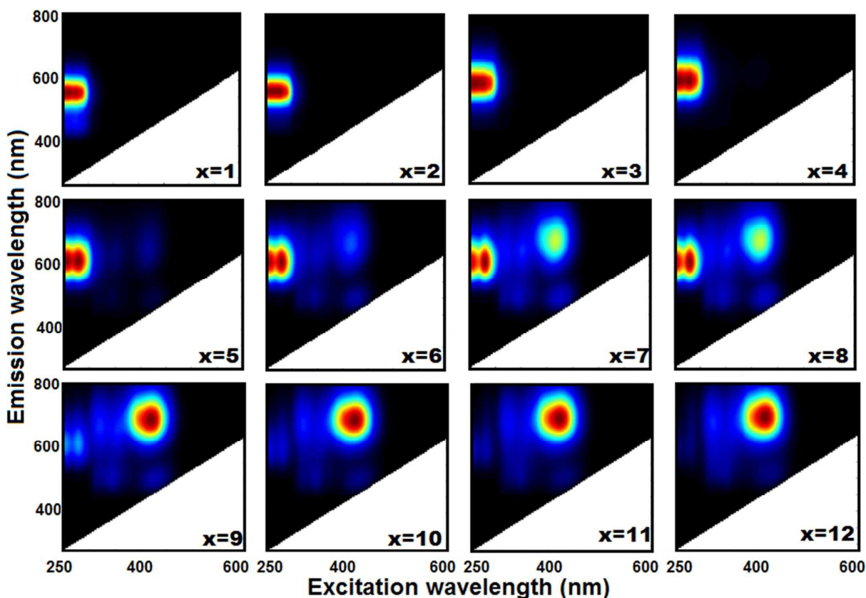
Fig. 2 Two dimensional excitation-emission profiles of luminescent LTA(Li)-Ag x samples in their fully hydrated state.
