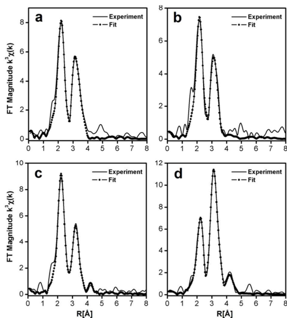
Fig. 7 Phase corrected FTs of the Ag K-edge k^3 -weighted EXAFS of LTA(Li)-Ag 1 composites (a) fully hydrated (pellet, ~ 19 % water content), (b) partially dehydrated (quartz cuvette, ~ 2 % water content), (c) partially dehydrated (glass capillary, ~ 1 % water content), (d) fully dehydrated (glass capillary).
