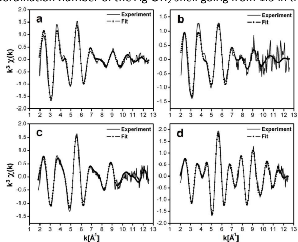
Fig. 6 Ag K-edge k^3 -weighted EXAFS spectra of LTA(Li)-Ag 1 composites, (a) fully hydrated (pellet, ~ 19 % water content), (b) partially dehydrated (quartz cuvette, ~ 2 % water content), (c) partially dehydrated (glass capillary, ~ 1 % water content), (d) fully dehydrated (glass capillary).
