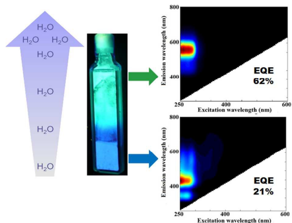
Fig. 4 Water dependence of the emission color observed in LTA(Li)-Ag 1 composites. In fully hydrated samples (19 % water content) a green emission was found, whereas in partially hydrated samples (2 % water content) blue emission was recorded. The water gradient observed in the cuvette was generated by leaving the material exposed to air under ambient conditions.
