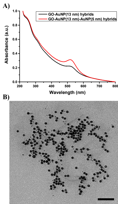
Figure 4 A) Normalized UV-vis spectra of GO-AuNP (13 nm) (black) and GO-AuNP (13 nm)-AuNP (5 nm) (red) hybrid assemblies; B) TEM micrograph of GO-AuNP (13 nm) - AuNP (5 nm) hybrid assemblies. Scale bar is 100 nm.
