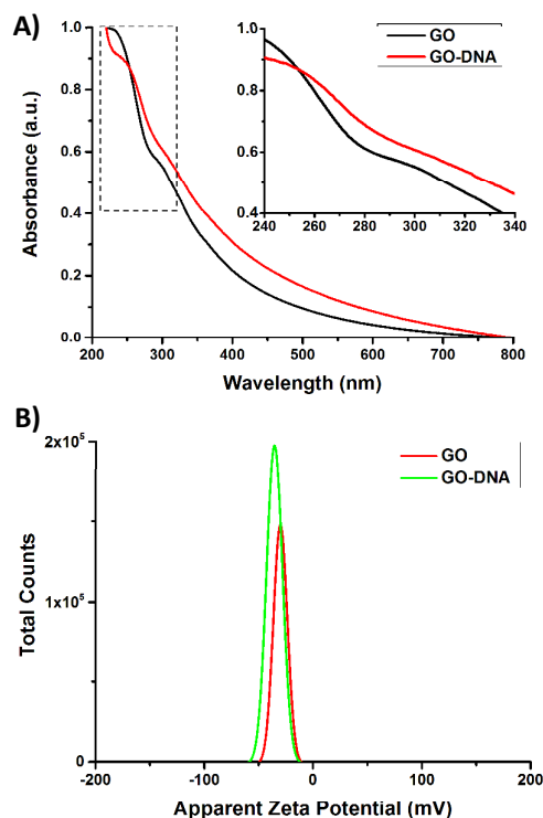
Figure 1 A) Normalized UV-vis spectra of GO (black) and DNA-modified GO (red). Inset: magnification of spectral region in the boxed area. B) \zeta -potential graphs of GO (red) and GO-DNA (green).
