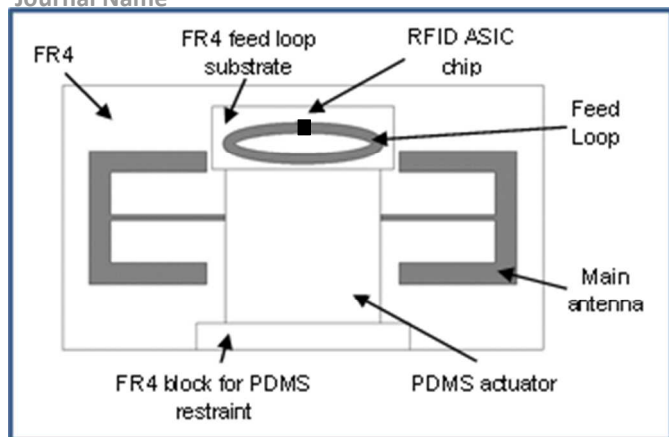
Figure 1: Displacement Feed Loop RFID Tag Antenna
