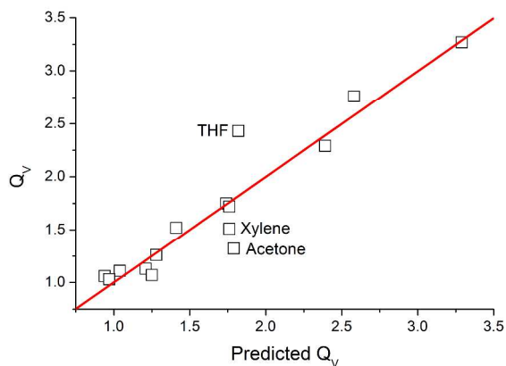
Figure 5: Measured volume swelling ratio versus predicted swelling ratio calculated using equation 6.
