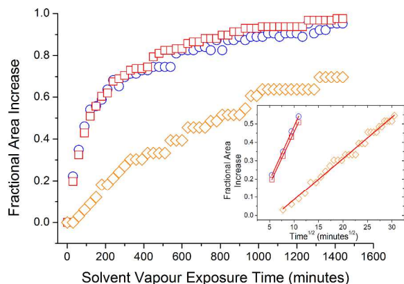
Figure 7: Swelling Kinetics for PDMS in \square diethyl ether, \circ DCM and \diamond xylene. Insert figure shows the first 55% swelling data versus the square root of time.
