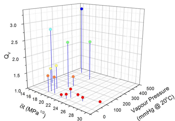
Figure 4: Swelling ratio versus the total Hansen solubility parameter and vapour pressure of each solvent
