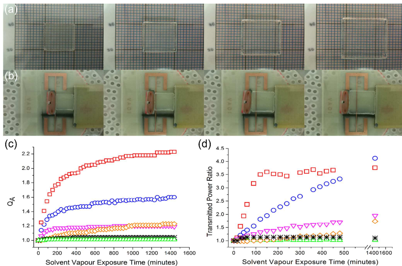
Figure 6: (a) Image of an elastomer from left to right after 0 minutes, 30 minutes, 150 minutes and 1440 minutes diethyl ether vapour exposure: top – images taken during absorption rate measurements; (b) Images taken during RFID measurements. (c) Area swelling ratio versus solvent exposure time. (d) Transmitted power ratio versus the solvent vapour exposure time. The symbols representing different solvents are the same for both (c) and (d) where: \square diethyl ether, \circ DCM, \nabla acetone, \diamond xylene, \triangle methanol and * acetonitrile.
