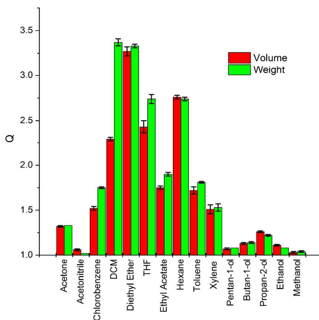
Figure 2: Swelling Ratio ( Q ) of PDMS elastomers after exposure to a range of solvent vapours
