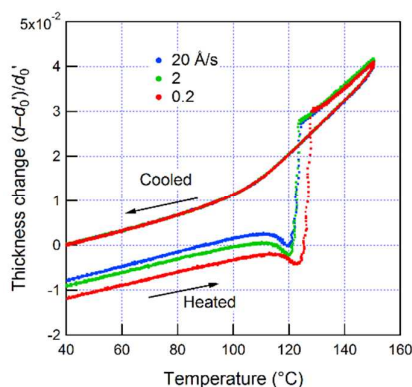
Fig. 16 Thickness changes of vacuum-deposited 2-TNATA films fabricated at different deposition rates of 0.2, 2, and 20 \text{ \AA/s} during a heating and cooling cycle. To compare the densities of the as-prepared films, the thicknesses at 40^\circ\text{C} after cooling d_0' are used as the standards for normalization.
