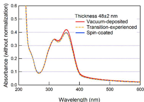
Fig. 9 Absorption spectra without normalization of as-prepared and transition-experienced vacuum-deposited TPD films, and a spin-coated TPD film. The original thicknesses of the vacuum-deposited and spin-coated films were approximately the same (47.0 and 49.1 nm, respectively).
