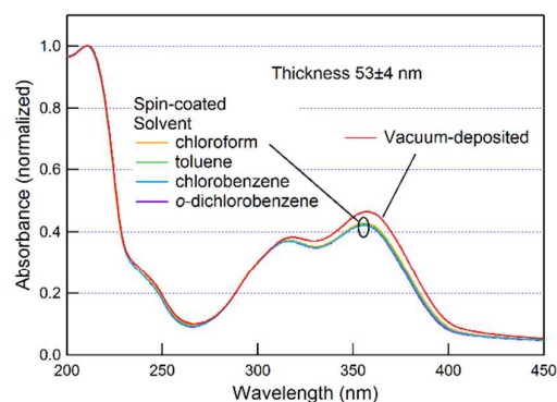
Fig. 6 Normalized absorption spectra of spin-coated TPD films fabricated using four different solvents and a vacuum-deposited TPD film. All films had approximately the same thickness of 53±4 nm: 49.6 nm (chloroform), 51.1 nm (toluene), 53.8 nm (chlorobenzene), 56.3 nm ( o -dichlorobenzene), and 52.3 nm (vacuum-deposited).
