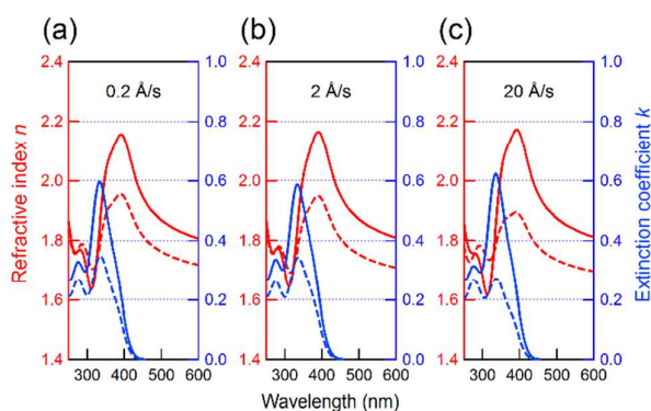
Fig. 17 Anisotropic optical constants of vacuum-deposited 2-TNATA films with a thickness of \sim 100 nm fabricated at deposition rates of (a) 0.2, (b) 2, and (c) 20 Å/s. The red solid and broken lines show the refractive indices in the horizontal and vertical directions ( n_o and n_e ), respectively, and the blue solid and broken lines show the extinction coefficients in the horizontal and vertical directions ( k_o and k_e ), respectively.
