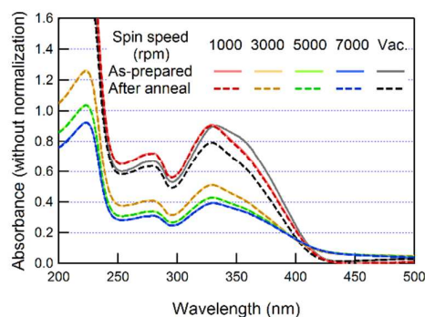
Fig. 14 Absorption spectra without normalization of as-prepared and transition-experienced spin-coated 2-TNATA films fabricated with a solution concentration of 15 mg ml -1 and different spin speed. Absorption spectra of as-prepared and transition-experienced vacuum-deposited 2-TNATA films with a thickness of ~100 nm are also shown.
