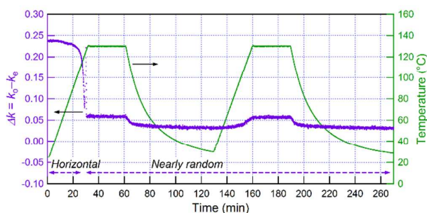
Fig. 15 Change of the anisotropy of extinction coefficients \Delta k = k_o - k_e at 332 nm of vacuum-deposited 2-TNATA films with a thickness of ~100 nm during heating-cooling cycles. The temperature during the cycles is also shown (green).
