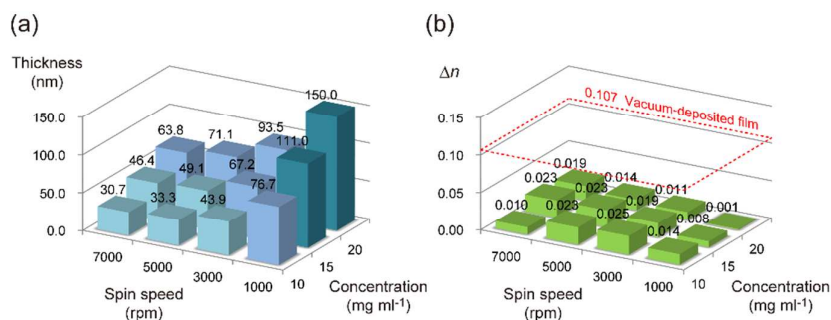
Fig. 13 (a) Thicknesses and (b) birefringences of spin-coated 2-TNATA films fabricated using chloroform as the solvent with different spin speed and solution concentration. The birefringence of the vacuum-deposited 2-TNATA film is also shown as a red dotted line.
