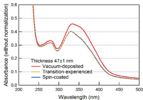
Fig. 12 Absorption spectra without normalization of as-prepared and transition-experienced vacuum-deposited 2-TNATA films, and a spin-coated 2-TNATA film. The original thicknesses of the as-prepared vacuum-deposited and spin-coated films were approximately the same (46.5 and 47.8 nm, respectively).
