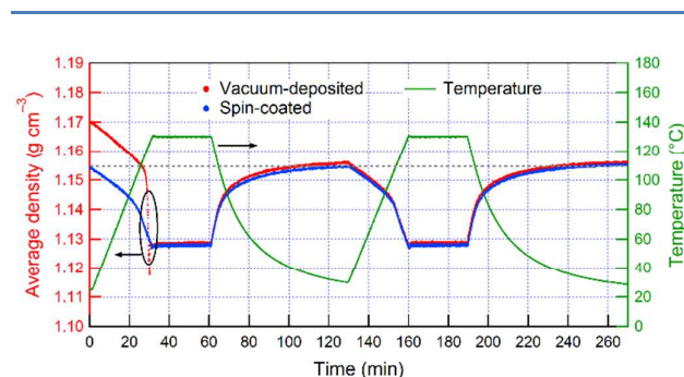
Fig. 10 Changes of the densities of vacuum-deposited (red) and spin-coated (blue) 2-TNATA films with a thickness of \sim 100 nm during heating-cooling cycles. The temperature during the cycles is also shown (green). The gray dotted horizontal line shows the identical density of the transition-experienced vacuum-deposited film and the spin-coated film at room temperature.
