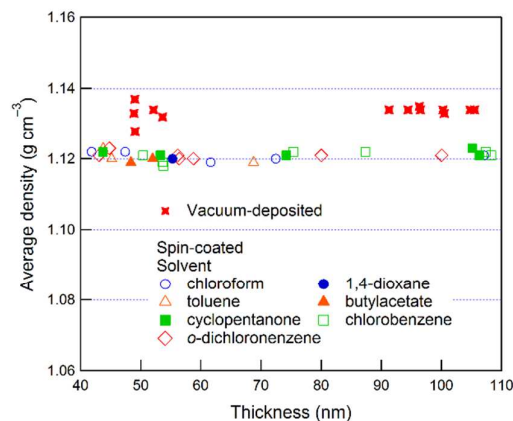
Fig. 5 Densities of spin-coated TPD films fabricated using different solvent, spin speed, and solution concentration. The densities of vacuum-deposited films with different thickness are also shown for comparison.
