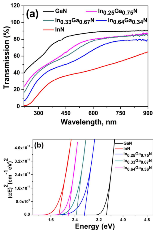
Figure 6. (a) Optical transmission spectra of GaN, InN, and In x Ga 1-x N thin films deposited on double-side polished quartz substrates. (b) (\alpha E)^2 vs. E plots, indicating the optical band gaps of GaN, InN, and In x Ga 1-x N thin films.
