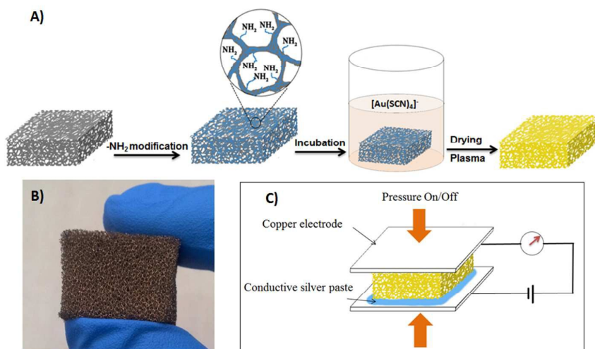
Fig. 1 Preparation of the Au-coated polyurethane piezoresistive sensor. A) Schematic illustration of the fabrication process. The PU sponge is functionalized to display amine residues. Subsequent incubation with Au thiocyanate results in thin gold coating of the polymer framework. B) Photograph of the Au/PU sponge. C) Schematic illustration of the operating principle of the piezoresistive sensor comprising the Au/PU sponge.
