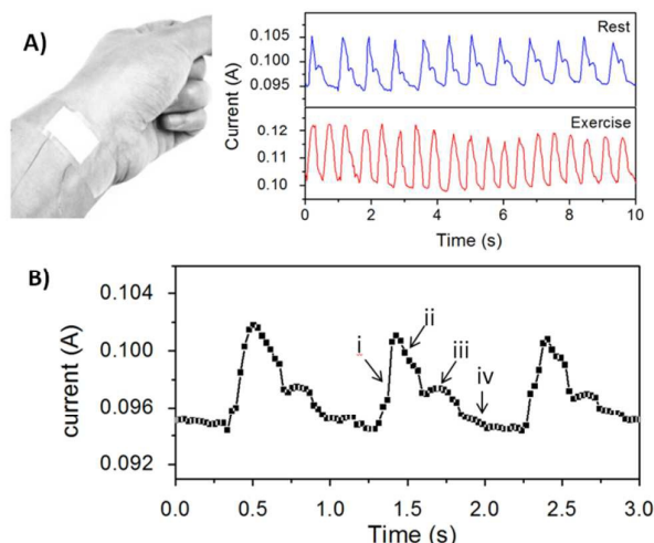
Fig. 4 Blood pulse sensing by the Au/PU sponge. A) Photograph of the pulse sensor placed upon the wrist artery, and signals of heartbeat measurement at rest (72 beats \text{min}^{-1} ) and after physical activity (114 beats \text{min}^{-1} ). B) High resolution monitoring of blood pressure in arterial pulses. The Au/PU sensor is capable of distinguishing the systolic uptake (i), systolic decline (ii), dicrotic notch (iii), and diastolic runoff (iv).
