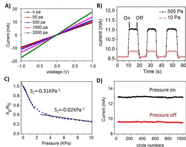
Fig. 3 Pressure-dependent electrical properties of the Au/PU sponge. A) Current-voltage (I-V) curves of Au/PU sponges recorded at different pressures. B) Pressure-dependent current recorded at different pressures (indicated). C) Pressure-response resistance plots for the Au/PU sponge pressure sensor. R_p corresponds to the resistance at pressure p , while R_0 is the pressure without pressure applied. The indicated slopes reflect the pressure sensitivities of the system (rates of resistance change upon pressure modulation). D) Stability of the sensor is demonstrated by repeatedly applying and releasing a pressure of 1 KPa in 1000 cycles.
