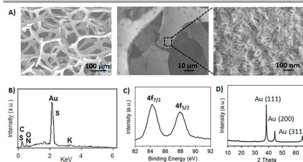
Fig. 2 Characterization of the Au films grown on the polyurethane sponge. A) Scanning electron microscopy (SEM) images of Au/PU sponge in different magnifications. B) The energy-dispersive X-ray spectroscopy (EDS) spectrum corresponding to the Au/PU sponge shown in A. C) X-ray photoelectron spectrum (XPS) of the Au/PU sponge; the two Au 0 peaks in the (4f) region are highlighted. D) X-ray diffraction (XRD) pattern of the Au/PU sponge; the reflections corresponding to Au crystal planes are apparent.
