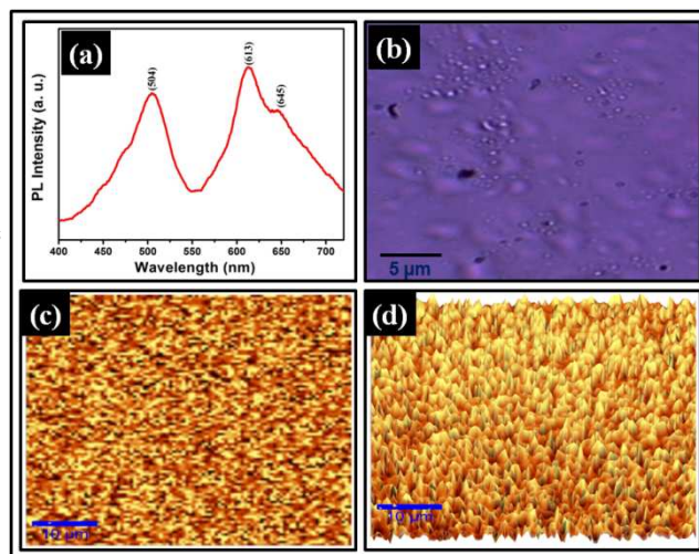
Fig. 4: (a) PL spectrum, (b) Optical micrograph image, (c) 2D top view and (d) 3D lateral view of combined PL mapping of plasmonic emission from Ag thin film as well as defect induced emission of Ag/ZnS/Ag multilayer thin film (sample 2; details are given in Table 1).
