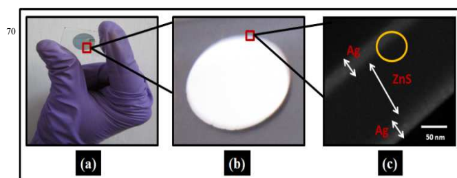
Fig. 2: (a) optical picture of Ag/ZnS/Ag multilayer thin film and (b) close view of thin film of Fig. 2a and (c) cross-sectional TEM image of multilayer alternate films of Ag and ZnS of sample 2 (details are given in Table 1). The yellow marked circle (in Fig. 2c) represents the interface between Ag and ZnS layers.
