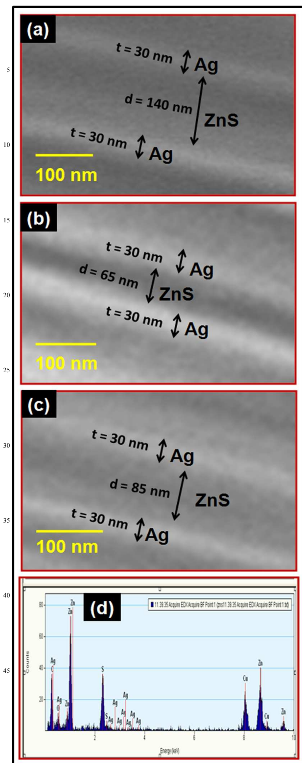
Fig. 10. Cross sectional SEM images of Ag/ZnS/Ag multilayer thin films; (a) blue color filter (30 nm /140 nm/ 30 nm), (b) green color filter (30 nm/ 65 nm/ 30 nm), (c) red color filter (30 nm/ 85 nm/ 30 nm) and (d) EDX spectrum of red color filter multilayer thin film.
