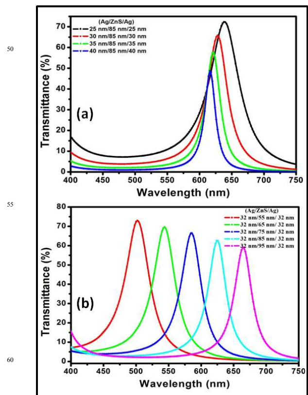
Fig. 6: Transmittance spectra of Ag/ZnS/Ag multilayer thin film structures (a) for varying the thickness of Ag (sample 1-4; details are given in Table 2) and (b) for different values of ZnS thickness (sample 5-9; details are given in Table 2) at normal angle of incidence.
