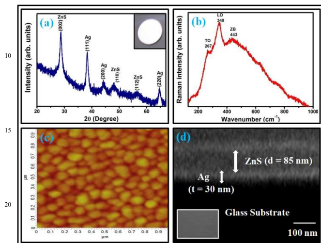
Fig. 1: (a) XRD pattern; inset shows the deposited film, (b) Raman spectrum, (c) 2D AFM image (sample 2) and (d) cross sectional SEM image; inset shows the top surface image of Ag/ZnS/Ag multilayer thin film of sample 2 (details are given in Table 1).
