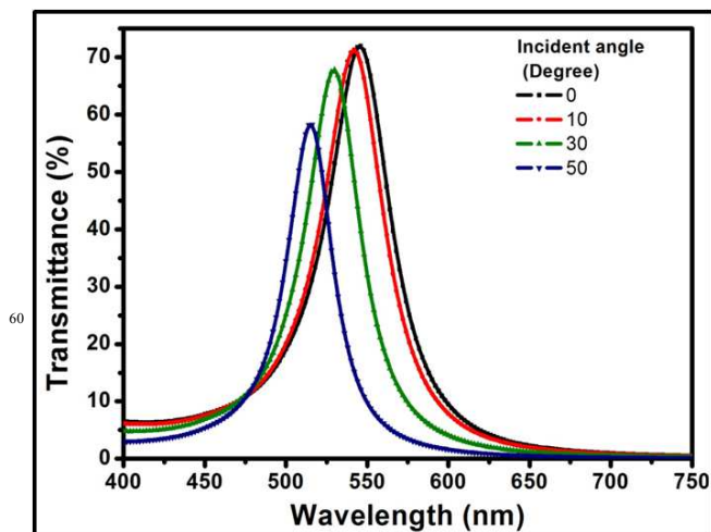
Fig. 7: Transmittance spectra of Ag/ZnS/Ag multilayer thin film (sample 6, details are given in Table 1) at different angle of incidence.
