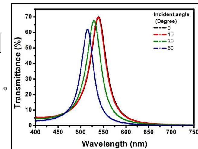
Fig. 9: Transmittance spectra for green color filter at different angle of incidence.
