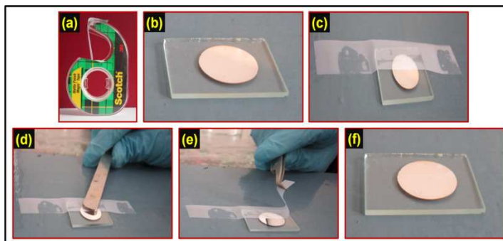
Fig. 3: Application of the “Scotch-tape” test to the artificially stacked Ag/ZnS/Ag multilayer film for measuring the mechanical stability; optical image of (a) Scotch-tape, (b) Ag/ZnS/Ag multilayer film, (c) applied a Scotch-tape to the Ag/ZnS/Ag multilayer film, (d) pressed the coating film by forceps, (e) pulled off the tape using forceps through hand and (f) Ag/ZnS/Ag multilayer film after removed the tape, resulting in a no delamination of film and mechanical stability was observed.
