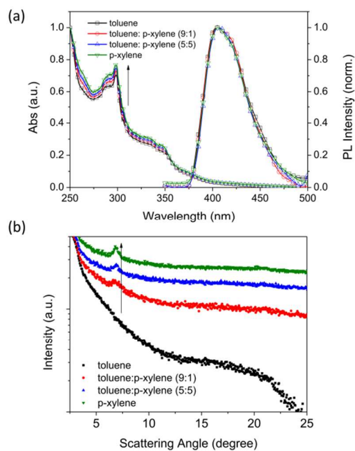
Figure 3. (a) UV-vis absorption and PL spectra and (b) GIXRD patterns of the H2 films spin-cast from different solvents or solvent mixtures.
