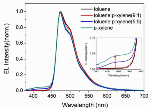
Figure 6. EL spectra of the solution-processed blue phosphorescent OLEDs with the H2:Flrpic emissive layer processed with toluene, p-xylene and toluene:p-xylene mixtures, respectively.
