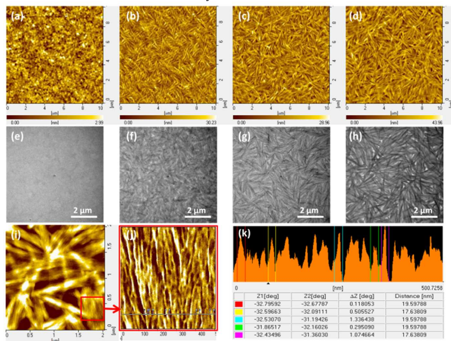
Figure 2. The AFM (a-d) and TEM (e-h) images for the H2 dendrimers spin-cast from (a, e) toluene, (b, f) toluene:p-xylene (9:1), (c, g) toluene:p-xylene (5:5), and (d, h) p-xylene solutions. (i, j) The magnified AFM images of the selected area in d. (k) The profiles across the line in j.
