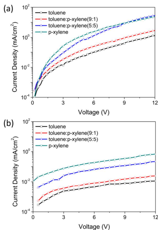
Figure 4. The current density-voltage characteristics of the (a) hole-only and (b) electron-only devices based on dendrimer H2 films prepared with different solvents or solvent mixtures.
