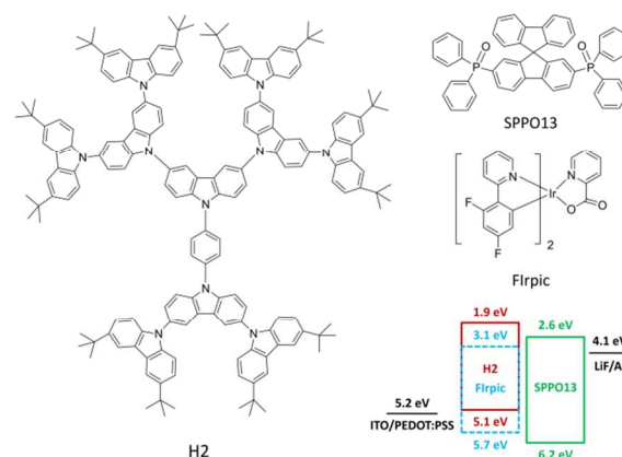
Figure 1. Chemical structures of the used materials and energy levels diagram of OLEDs.
