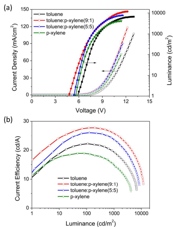
Figure 5. (a) Current density-luminance-voltage and (b) current efficiency-luminance curves of the solution-processed blue phosphorescent OLEDs with the H2:Firpic emissive layer processed with toluene, p-xylene and toluene:p-xylene mixtures, respectively.
