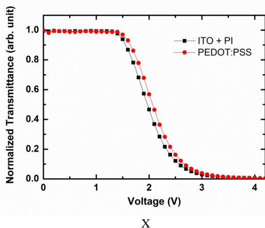
Fig. 10 Transmittance of TN LC cells fabricated by the rubbed highly conductive PEDOT:PSS on glass and polyimide on ITO glass under applied AC square wave voltage.
