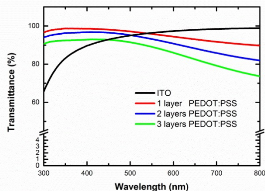
Fig. 7 Transmittance spectra of ITO and PEDOT:PSS film with different layers. The sheet resistance of the ITO is 95\ \Omega/\square .
