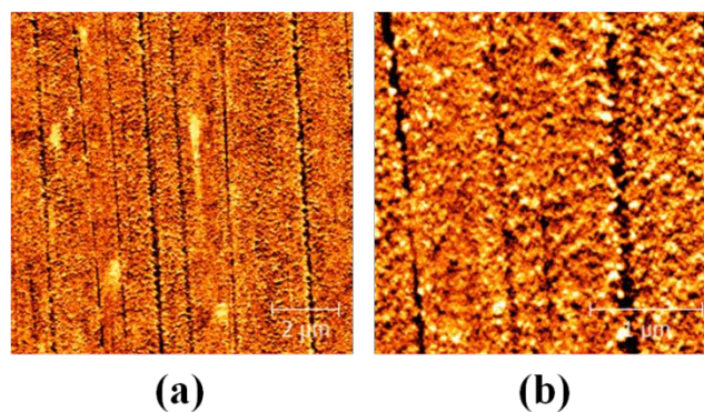
Fig. 8 Surface topography of the rubbed highly conductive PEDOT:PSS films. The dimension of these images are (a) 10\ \mu\text{m} \times 10\ \mu\text{m} and (b) 3\ \mu\text{m} \times 3\ \mu\text{m} .
