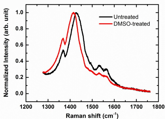
Fig. 6 Raman spectra of PEDOT:PSS films before and after the DMSO post-treatment.
