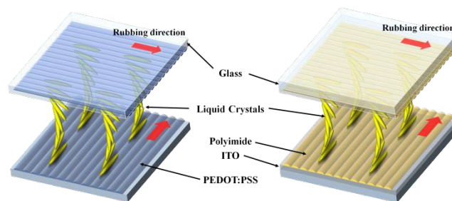
Fig. 1 The structure of LC cells fabricated by the rubbed highly conductive PEDOT:PSS on glass and polyimide on ITO glass.
