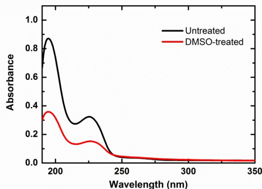
Fig. 4 UV absorption spectra of PEDOT:PSS films before and after the DMSO post-treatment.
