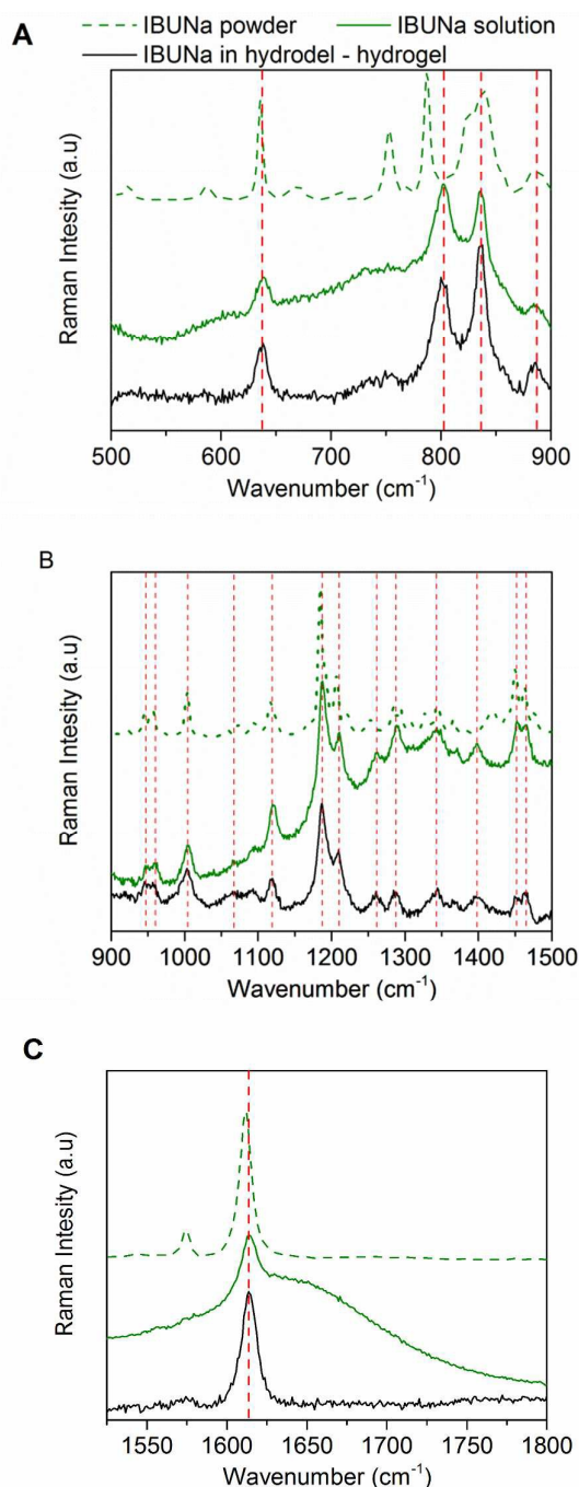
Fig. 3. Raman spectra of IBUNa: powder (green dot line) and aqueous solution (green line) in relation to differential spectrum of IBUNa in hydrogel and hydrogel in three regions: 500-900 (A), 900-1500 (B), 1525-1800 (C) cm^{-1} .
