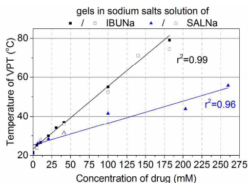
Fig. 2. Comparison of T_{VPT} determined by DSC and TOA. Dependence of T_{VPT} as a function of IBUNa concentration - full symbols correspond to the deflection points of TOA curves, while empty symbols correspond to the DSC thermogram extremes. T_{VPT} for SALNa were added for comparison.
