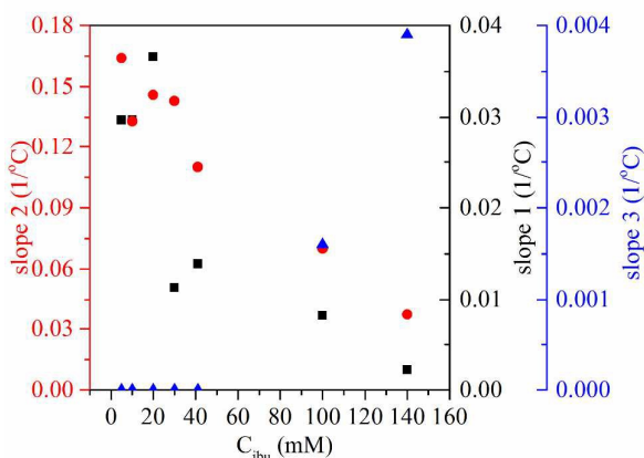
Fig. 4. VPT dynamics in the presence of ibuprofen sodium salt. Dynamics of VPT transition represented by slopes of TOA dependences shown in Fig. 1 in three regimes: slope 1 – squares, slope 2 – dots, slope 3 – triangles (see text for details).
