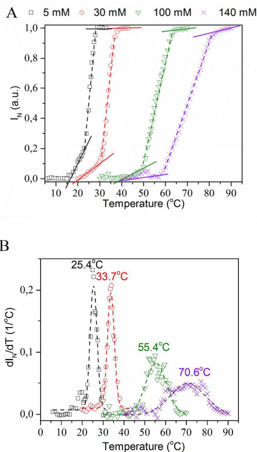
Fig. 1. Influence of IBUNa on VPT in PMEO 2 MA hydrogels. (A) I_N (normalised white light intensity transmitted through the sample) as a function of temperature for PMEO 2 MA hydrogels immersed in aqueous solutions of IBUNa with different concentrations; (B) first derivative of I_N(T) with respect to T .
